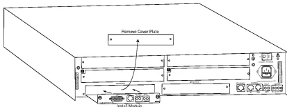
Figure 1. Installing the T1 Network Interface Module
