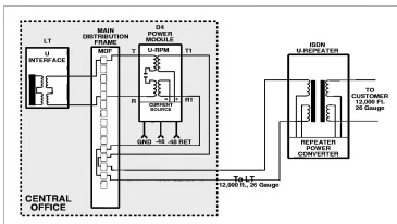
FIGURE 2. U-Repeater Powering Module Application
