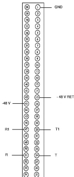
FIGURE 3. Connector Pin Assignments
