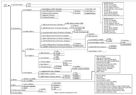
Figure 3. SHDSL T1/E1 NTU Menu Tree
