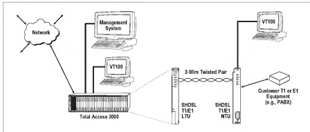
Figure 2. Typical System Application
