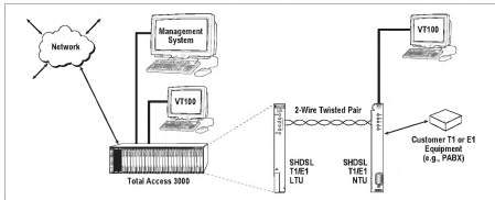
Figure 2. Typical System Application
