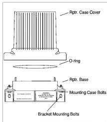
Figure 5. T400 Environmental Housing Assembly
