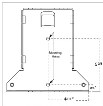
Figure 3. Mounting Holes
