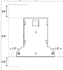
Figure 2. Clearances
