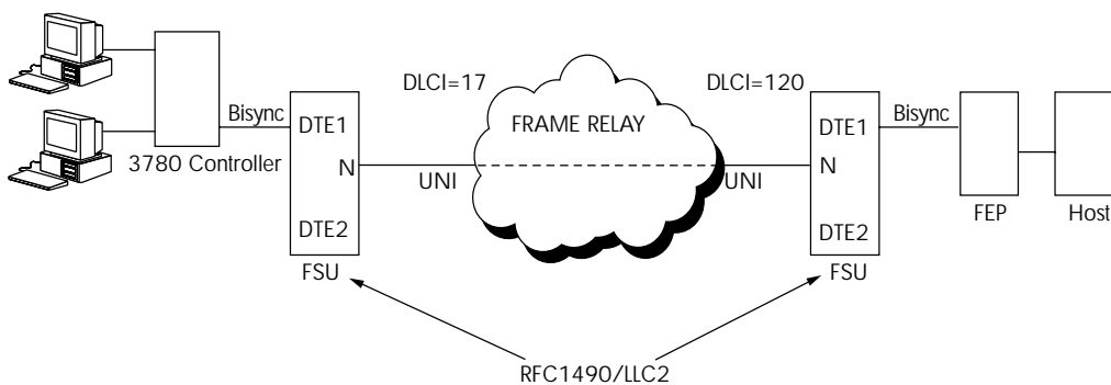
Figure 4-3 Bisync Point-to-Point
