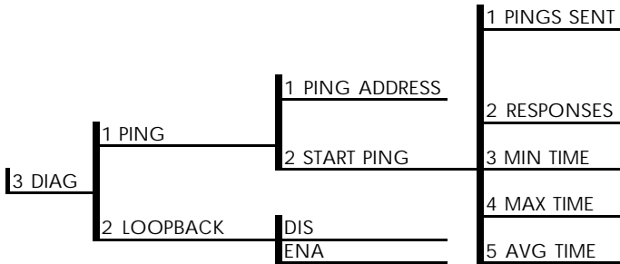
Figure 11-2 Front Panel Diagnostics Menu
