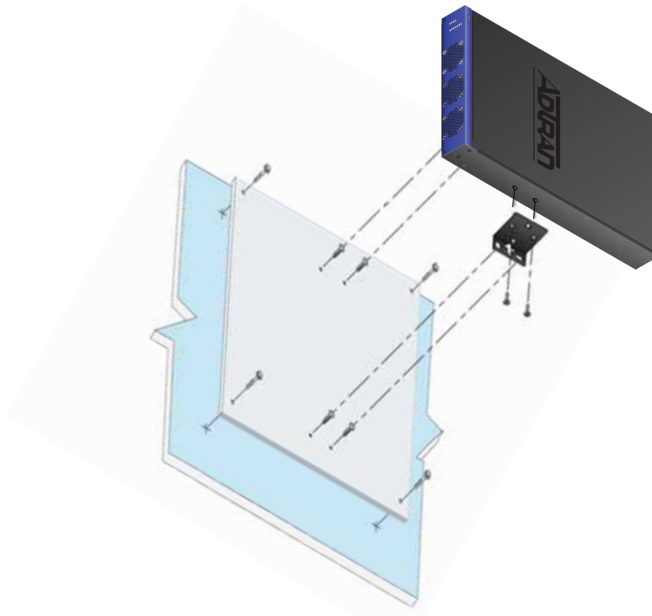
Figure 25. Wall Mounting the NetVanta 1131
