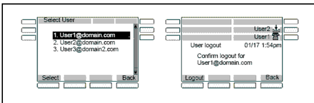
Figure 47: Logout screens
