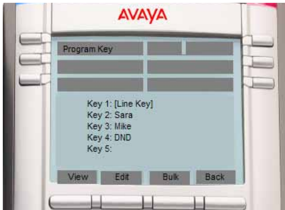
Figure 38: Feature keys
