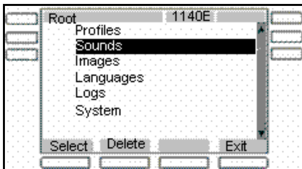
Figure 69: Root screen
