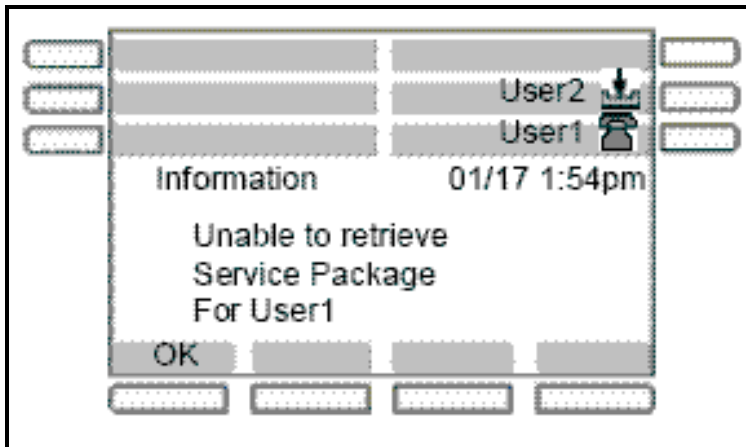
Figure 51: Per-account notifications
