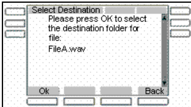
Figure 72: Select destination
