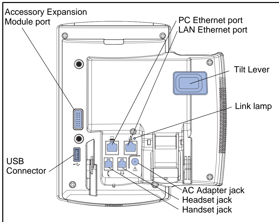
Figure 9: IP Deskphone connections
