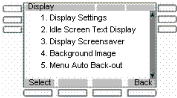
Figure 63: Display menu
