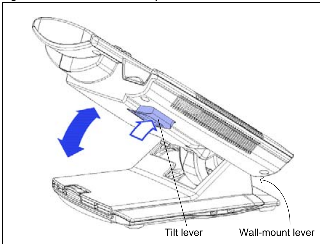
Figure 13: Rotate the IP Deskphone into the wall mount
