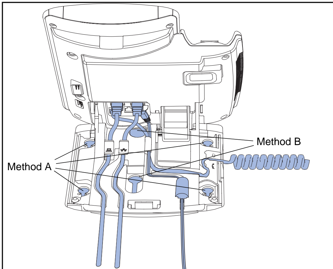
Figure 12: Cable routing tracks and mounting holes
