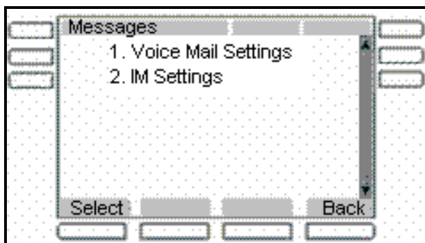
Figure 27: Messages screen
