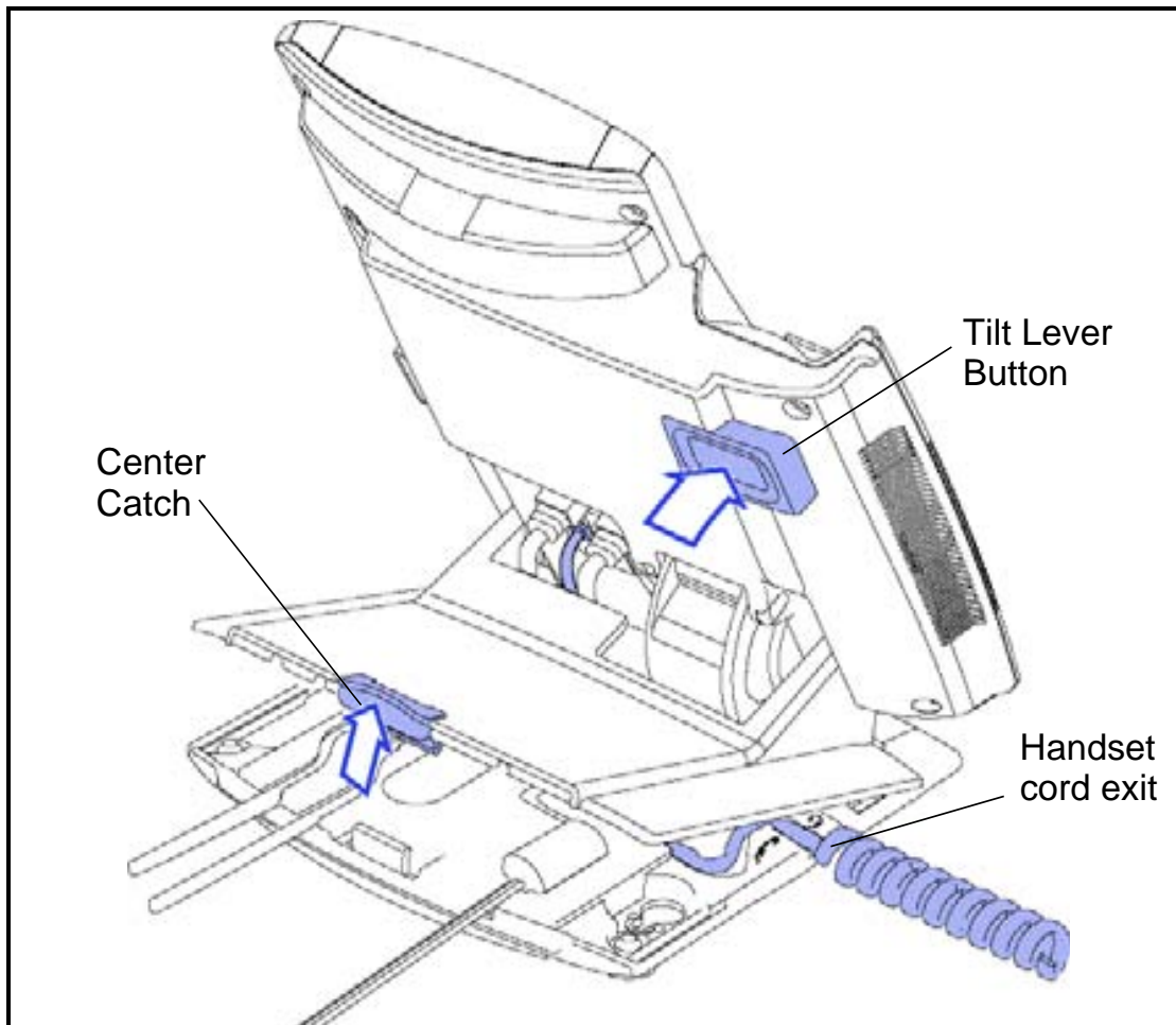
Figure 11: Remove the stand cover
