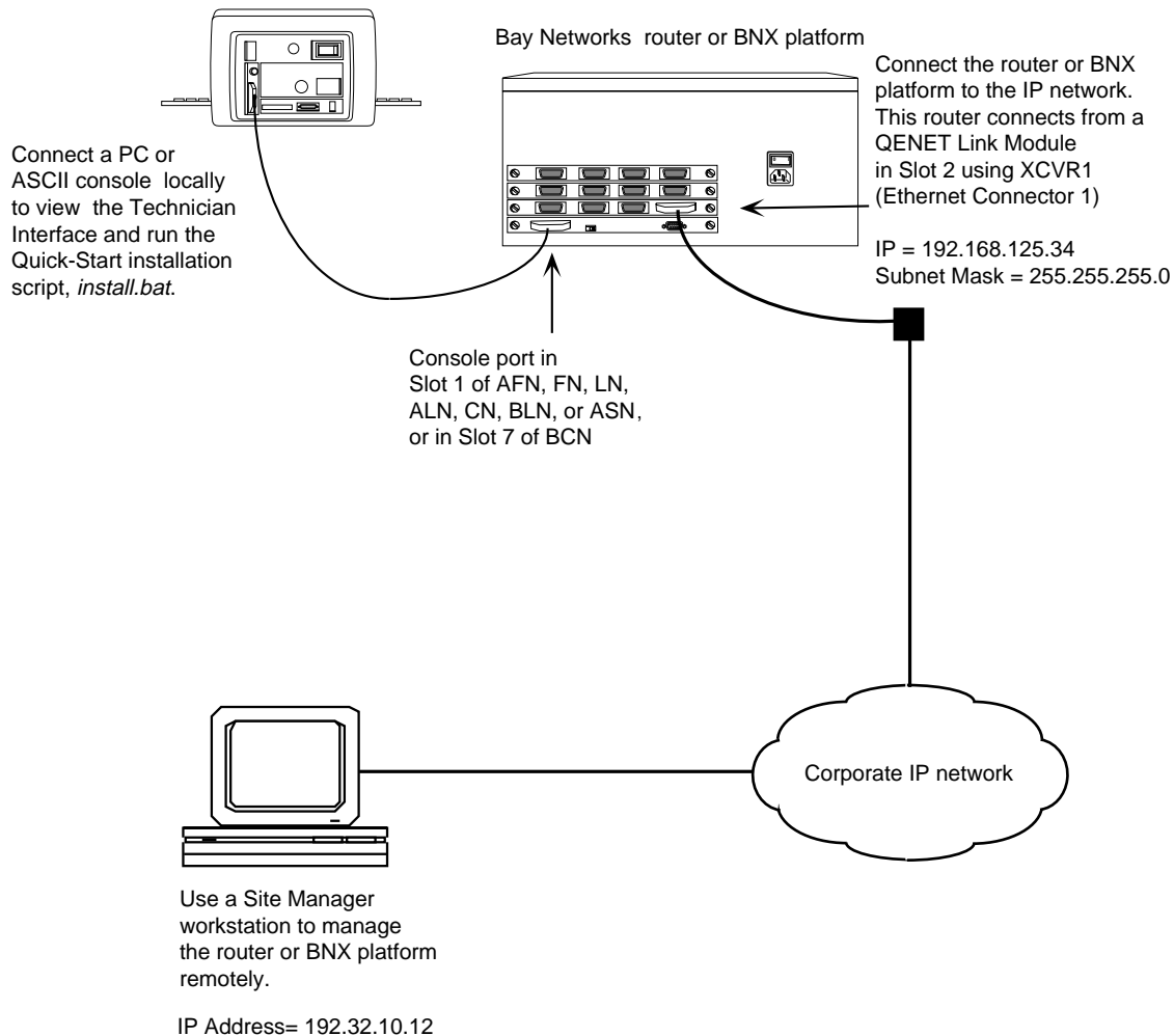
Figure 2-1. Sample Network Used In Worksheet Examples
