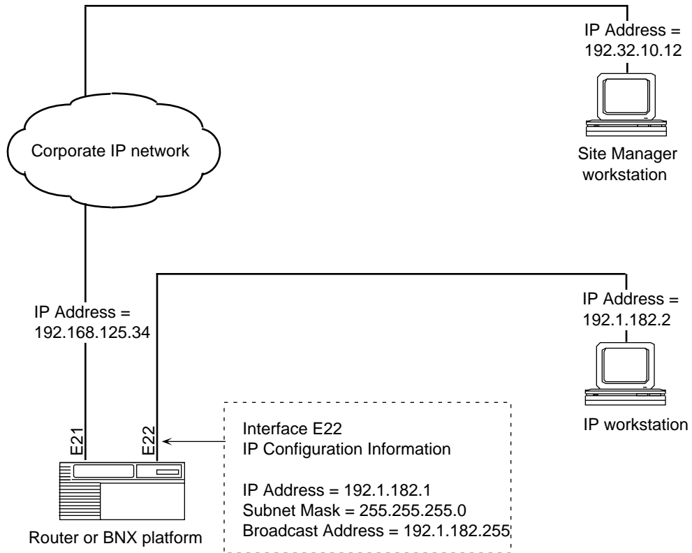
Figure 11-1. Sample Pilot Configuration
