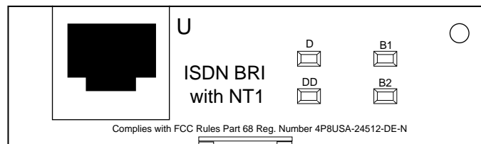
Figure 2-2. ISDN BRI Adapter Module with U Interface
