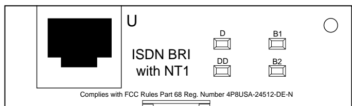
Figure 3-2. ISDN BRI Adapter Module (with U Interface) LEDs
