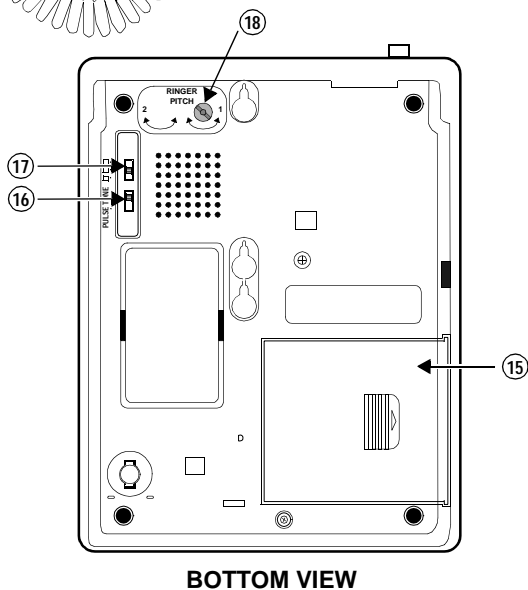
Figure 1: Lucent Technologies 9103 Telephone, Top and Bottom Views
