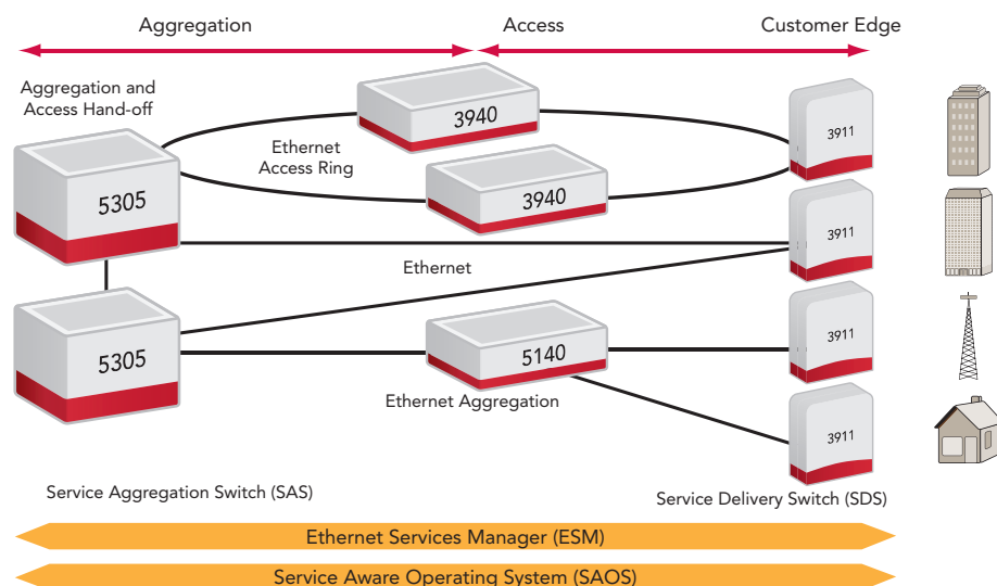
Figure 1. 3911 deployment options
