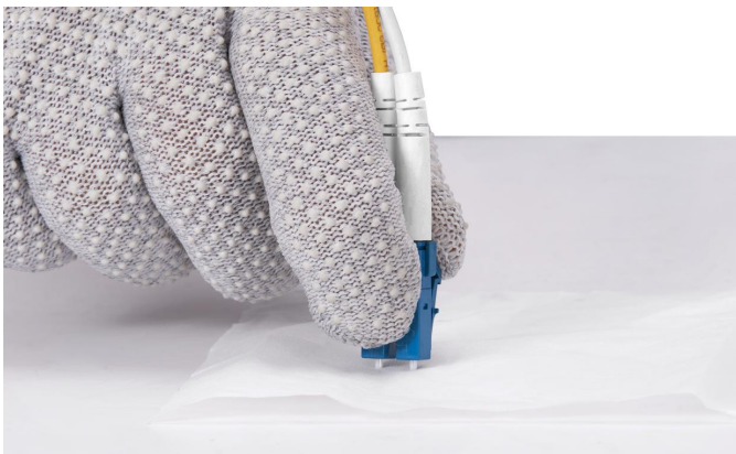
Figure 20: Cleaning Optical Fibers with Special Cleaning Tissues
