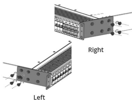
Figure 1: Mounting the Brackets
