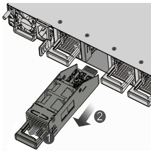
Figure 13: Removing a Fan Module
