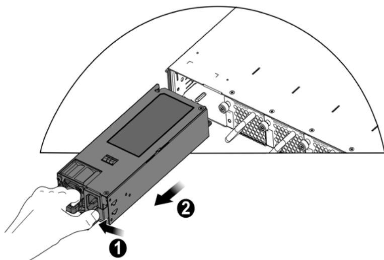
Figure 14: Removing a Power Module
