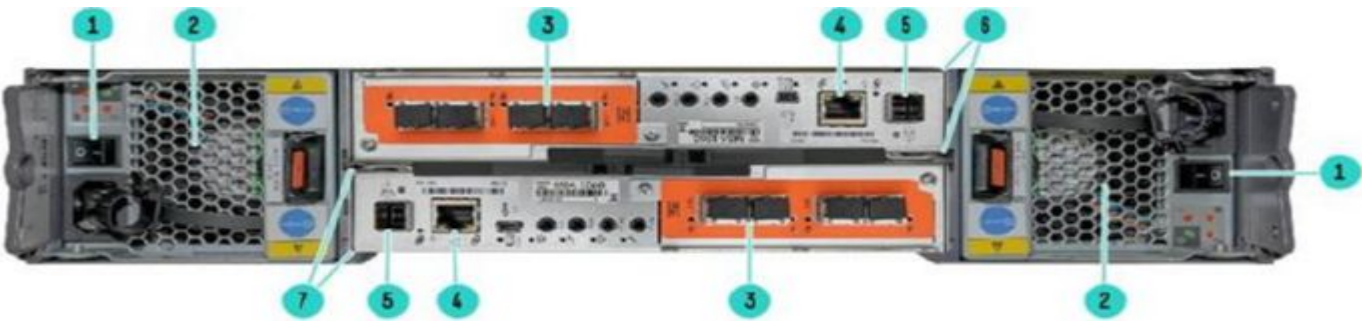
HPE MSA 2060 Storage
