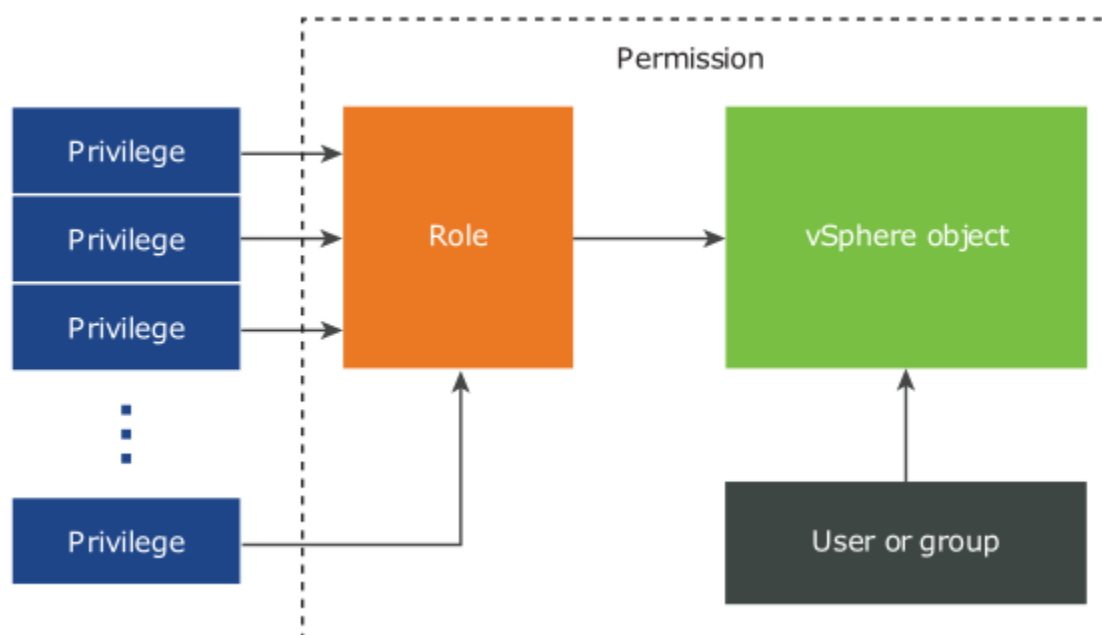
Figure 112: vSphere Permissions
