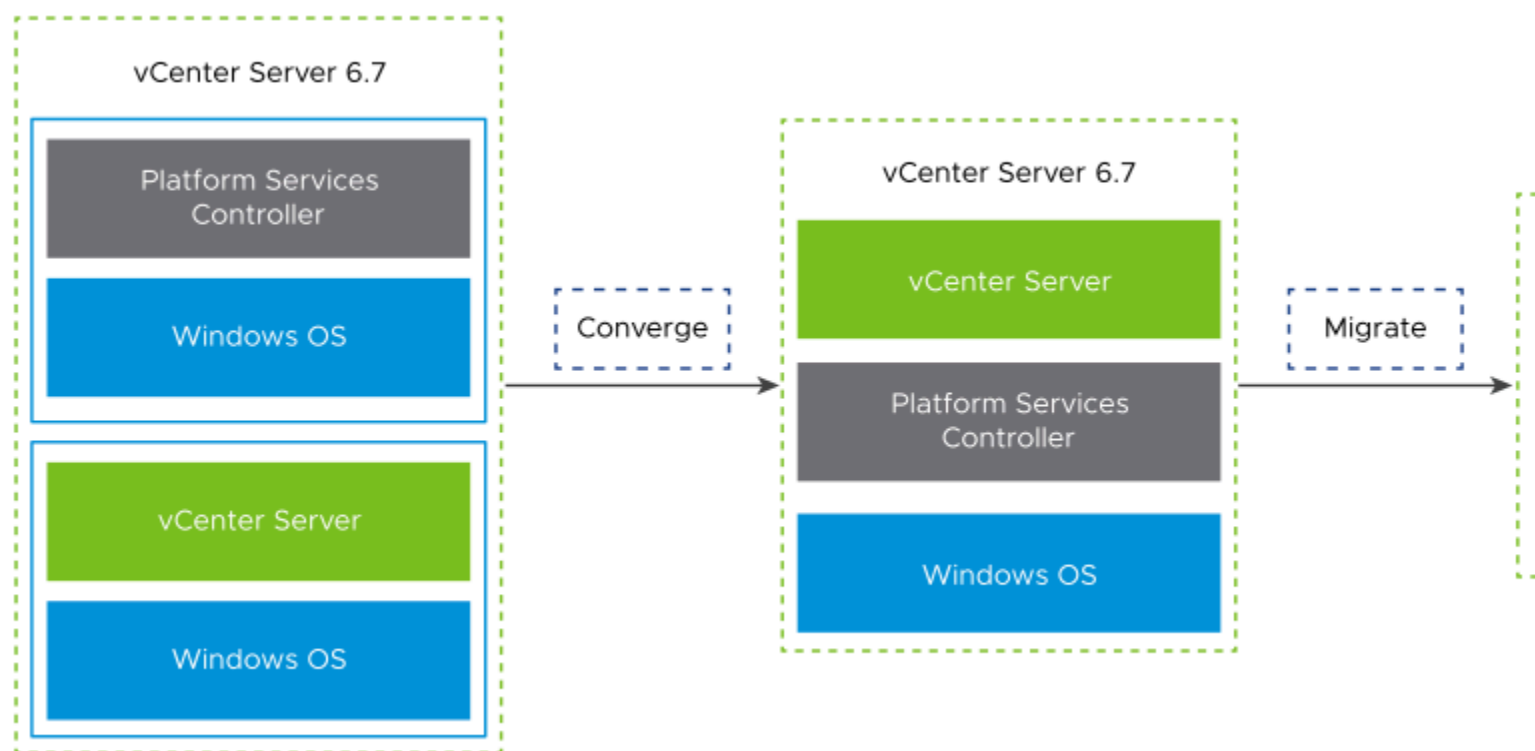
Figure 51: vCenter Server 6.7 with External Platform Services Controller Before and After Migration
