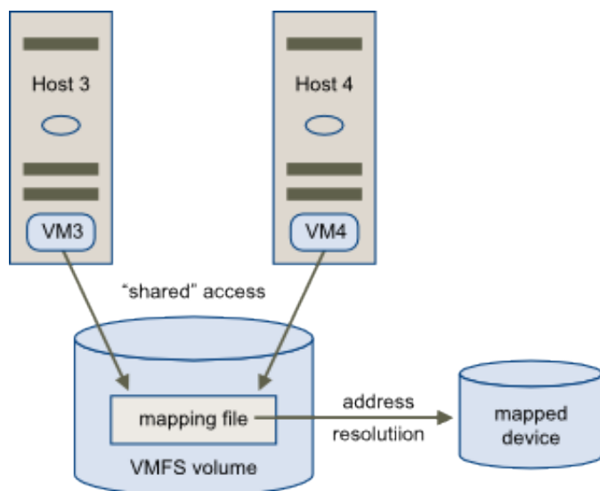
Figure 109: Access from Clustered Virtual Machines
