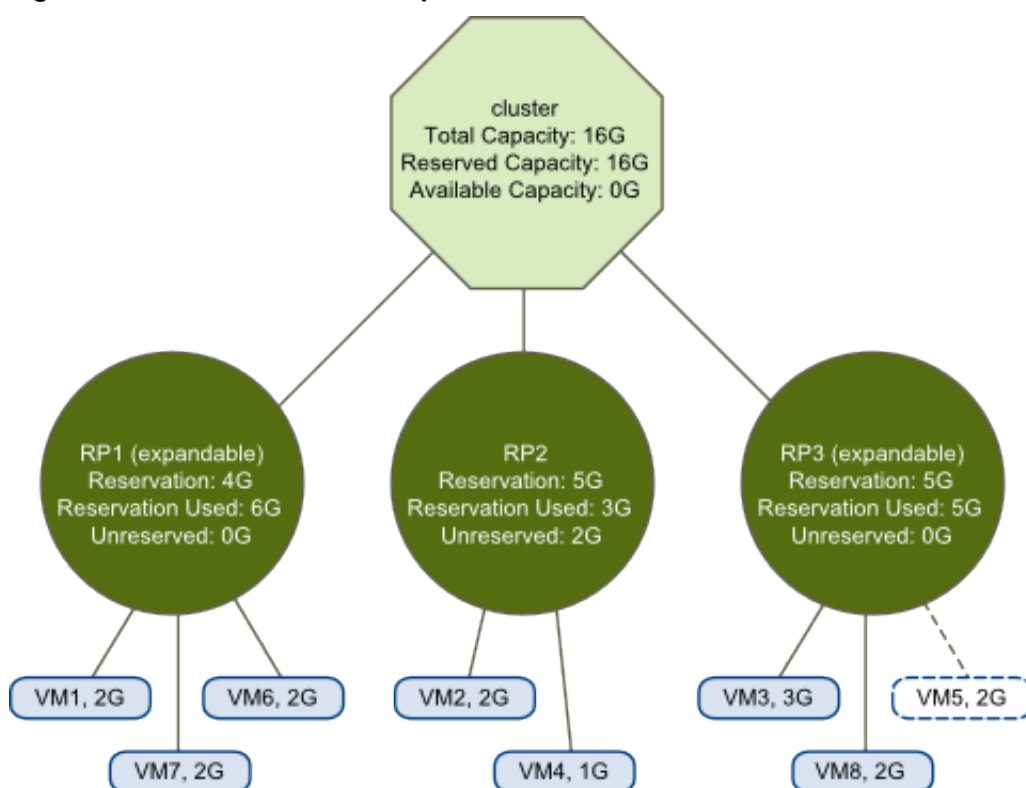
Figure 135: Valid Cluster with Expandable Resource Pools
