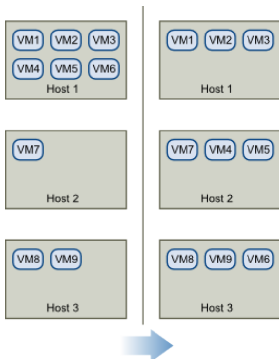
Figure 133: Load Balancing
