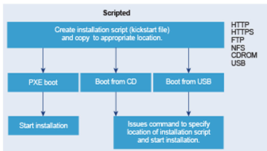
Figure 14: Scripted Installation
