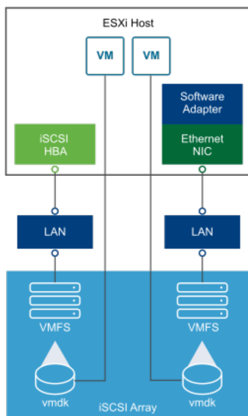
Figure 91: iSCSI Storage
