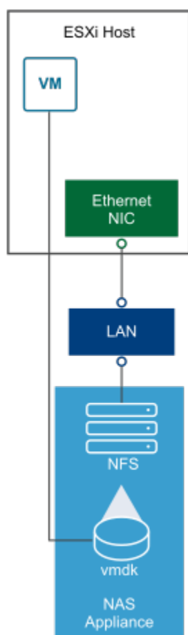
Figure 92: NFS Storage
