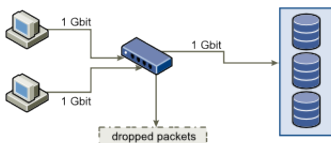
Figure 97: Dropped Packets
