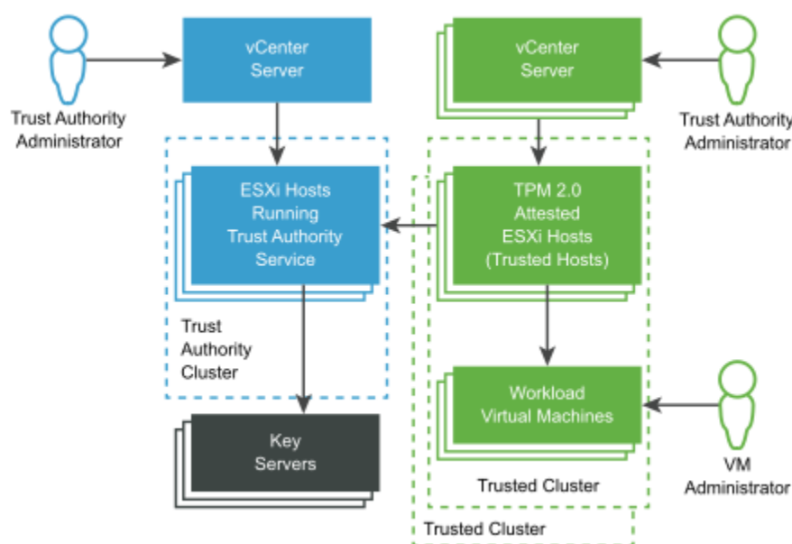
Figure 118: vSphere Trust Authority Architecture
