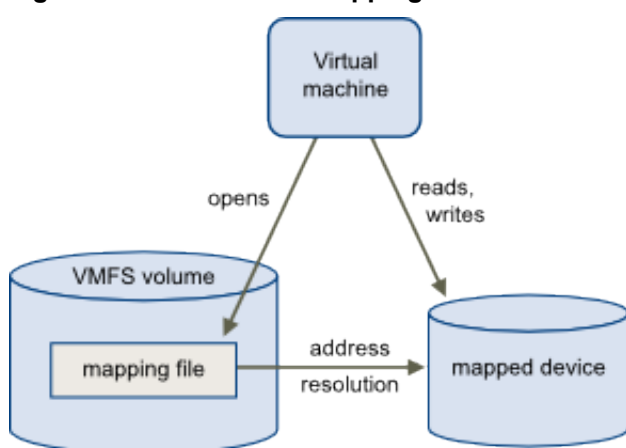
Figure 107: Raw Device Mapping
