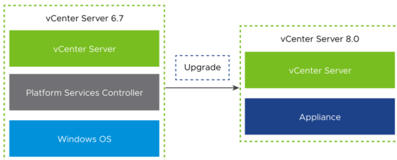
Figure 42: vCenter Server 6.7 with Embedded Platform Services Controller Before and After Upgrade
