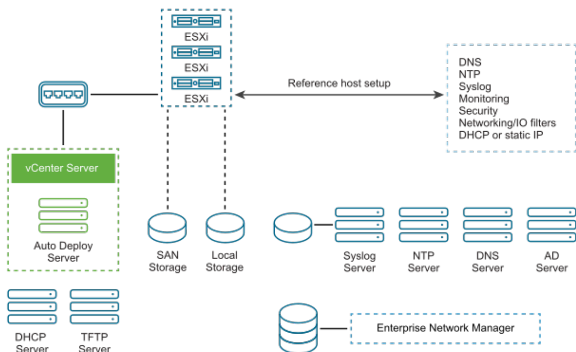
Figure 20: vSphere Auto Deploy Reference Host Setup
