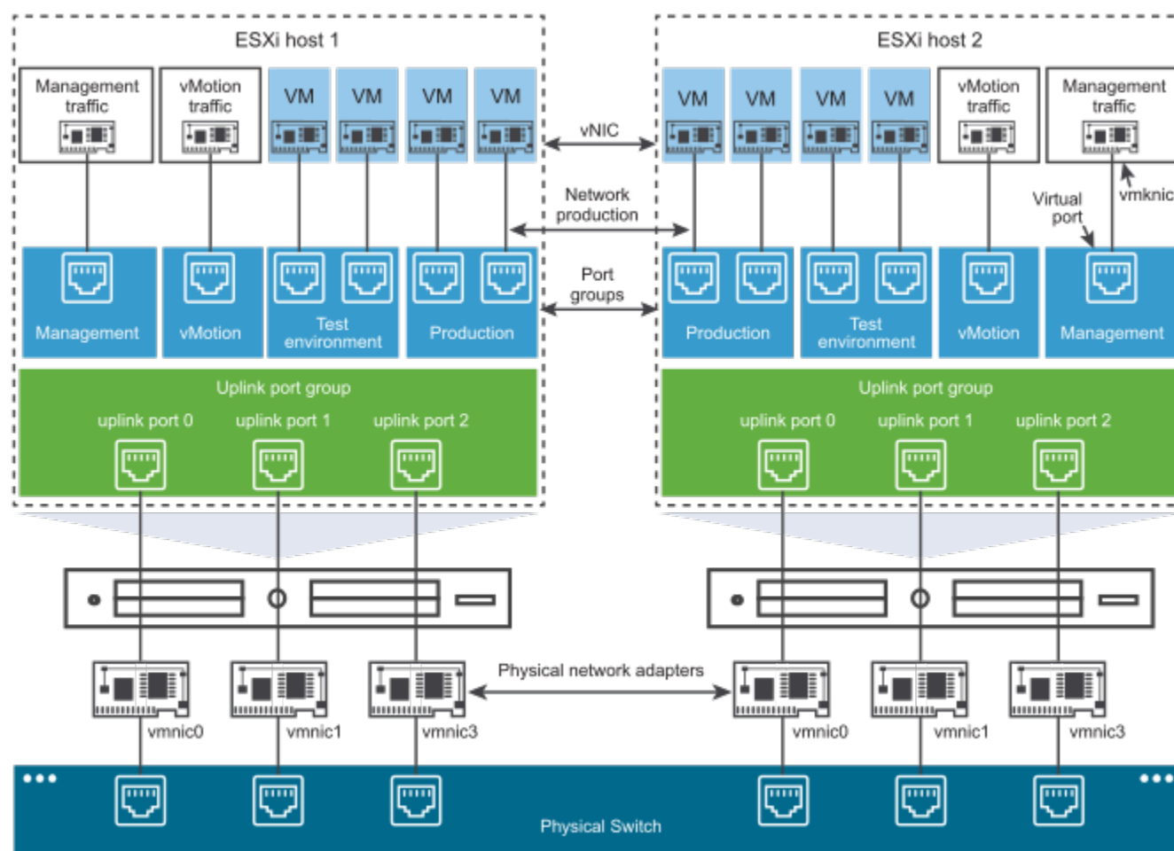
Figure 67: vSphere Standard Switch architecture
