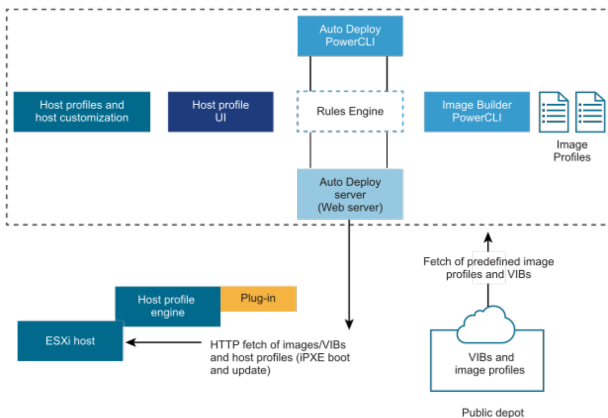
Figure 17: vSphere Auto Deploy Architecture
