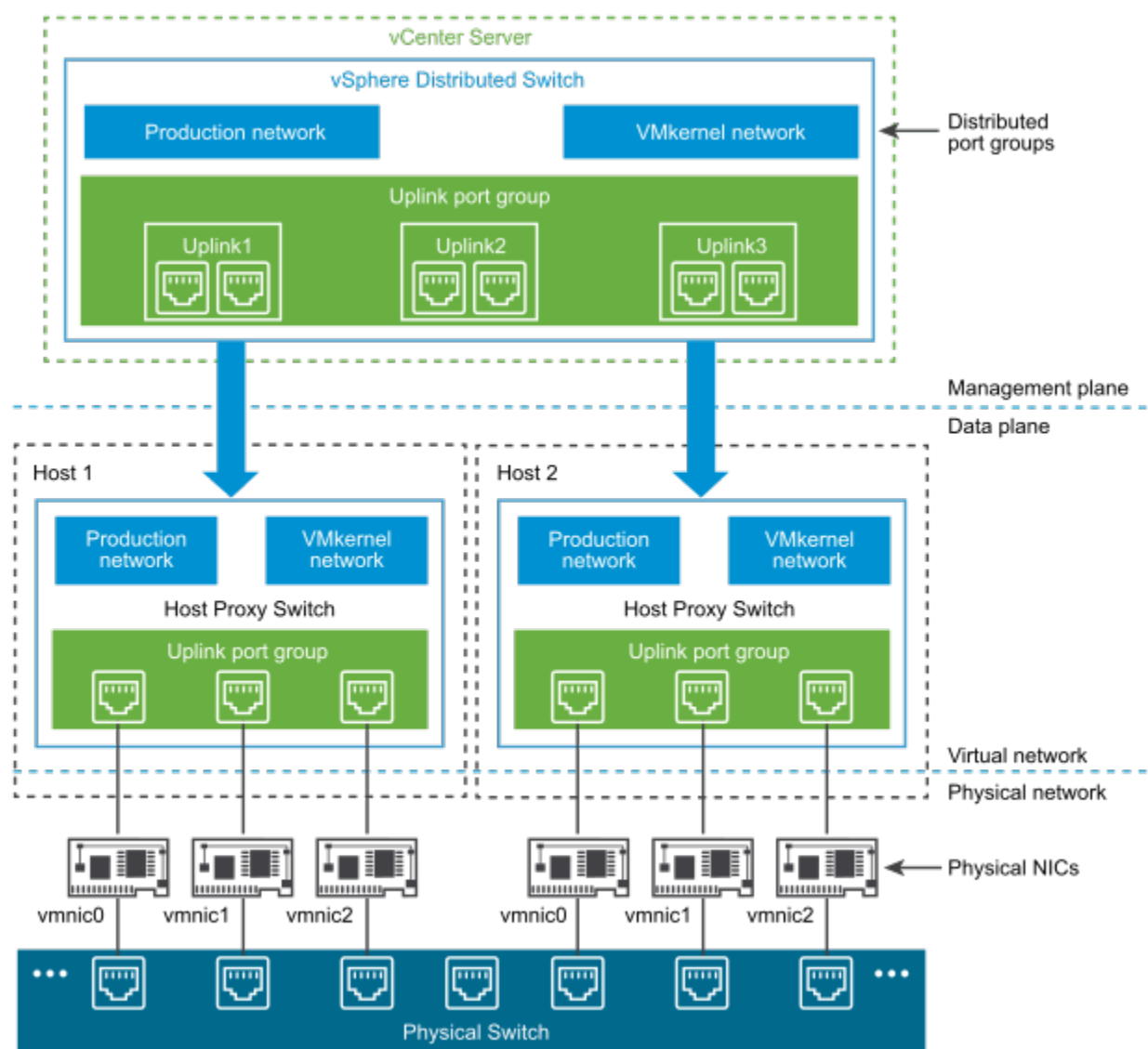
Figure 69: vSphere Distributed Switch Architecture
