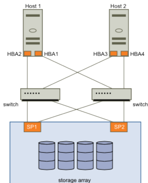
Figure 102: Multipathing and Failover with Fibre Channel
