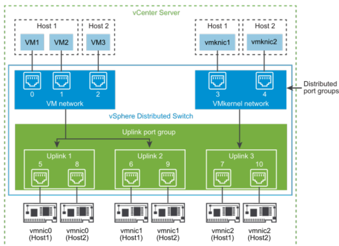
Figure 70: NIC Teaming and Port Allocation on a vSphere Distributed Switch
