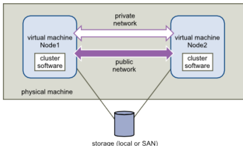
Figure 141: Virtual Machines Clustered on a Single Host
