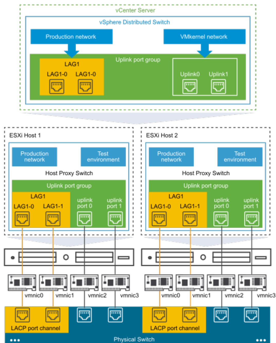
Figure 82: Enhanced LACP Support on a vSphere Distributed Switch
