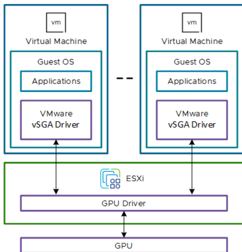
Figure 66: High-level architecture of vSGA
