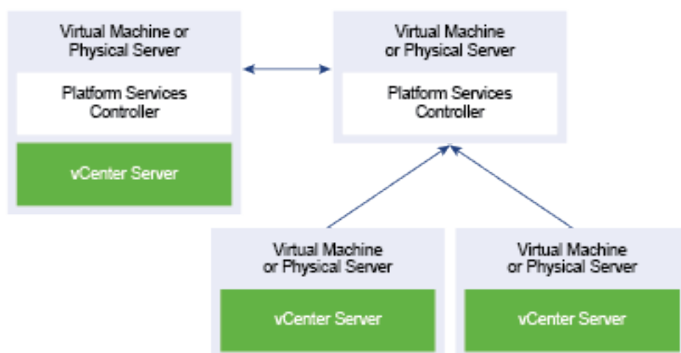
Figure 41: Deprecated Topology of an Embedded Platform Services Controller and an External Platform Services Controller in Replication
