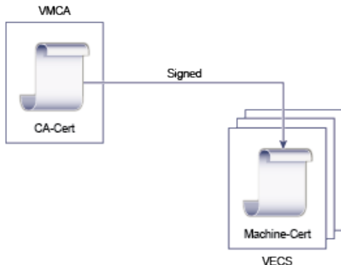
Figure 53: Certificates Signed by VMCA Are Stored in VECS
