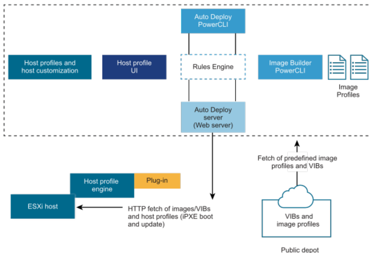
Figure 27: vSphere Auto Deploy Architecture
