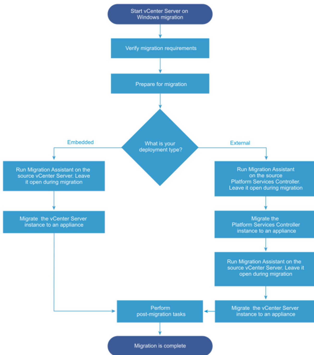
Figure 48: High-level Tasks for vCenter Server on Windows Migration to vCenter Server Appliance8.0
