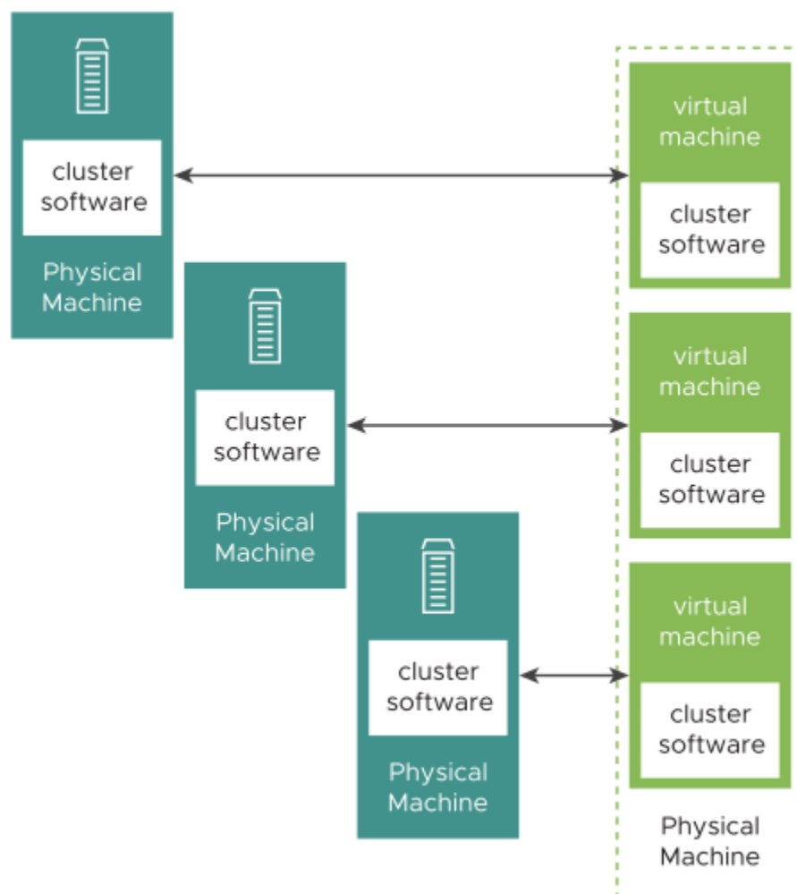
Figure 143: Clustering Physical and Virtual Machines
