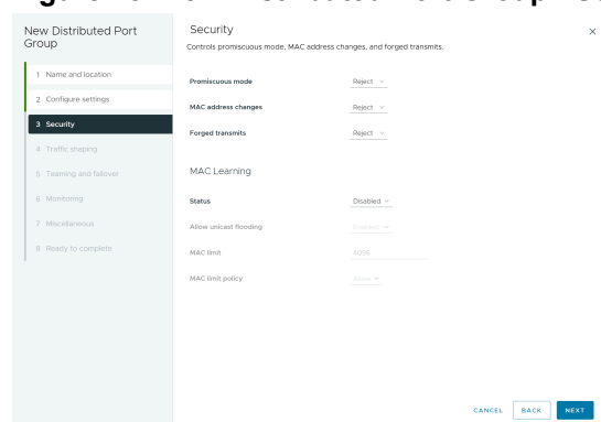
Figure 75: New Distributed Port Group - Security
