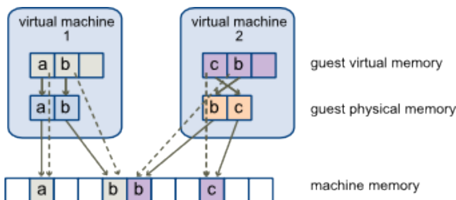
Figure 126: ESXi Memory Mapping
