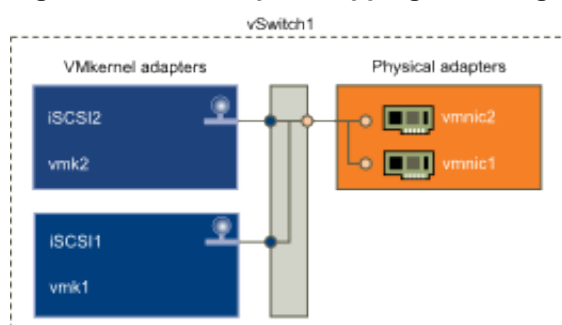
Figure 100: 1:1 Adapter Mapping on a Single vSphere Standard Switch
