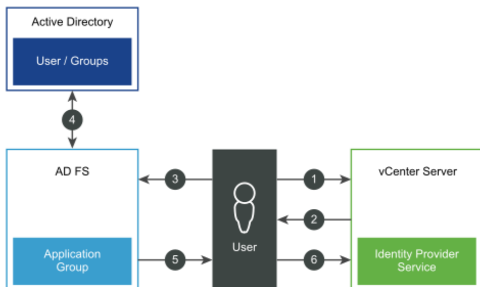
Figure 56: vCenter Server User Login Using AD FS Identity Provider Federation
