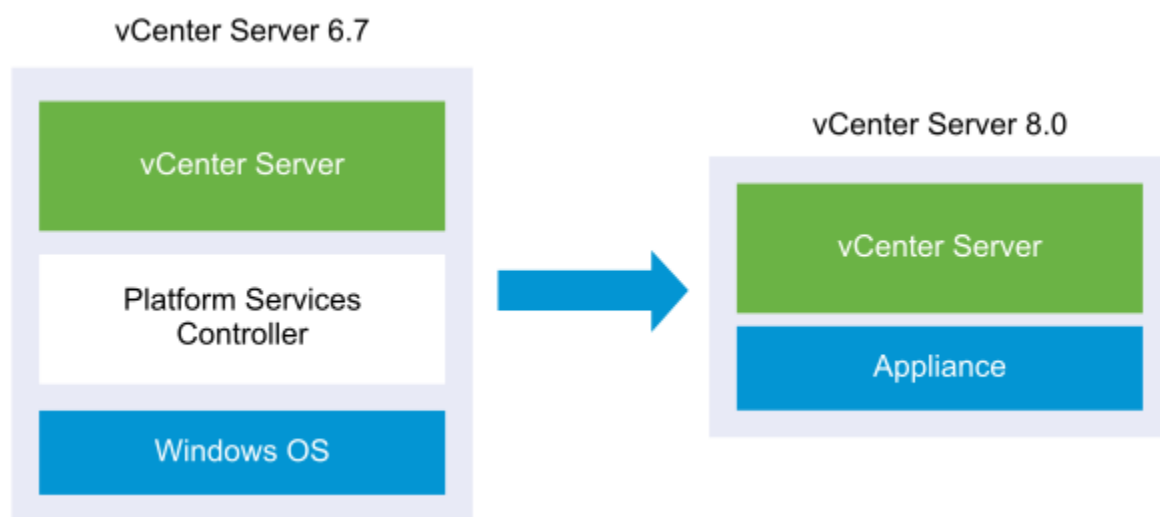
Figure 49: vCenter Server 6.7 with Embedded Platform Services Controller Deployment Before and After Migration
