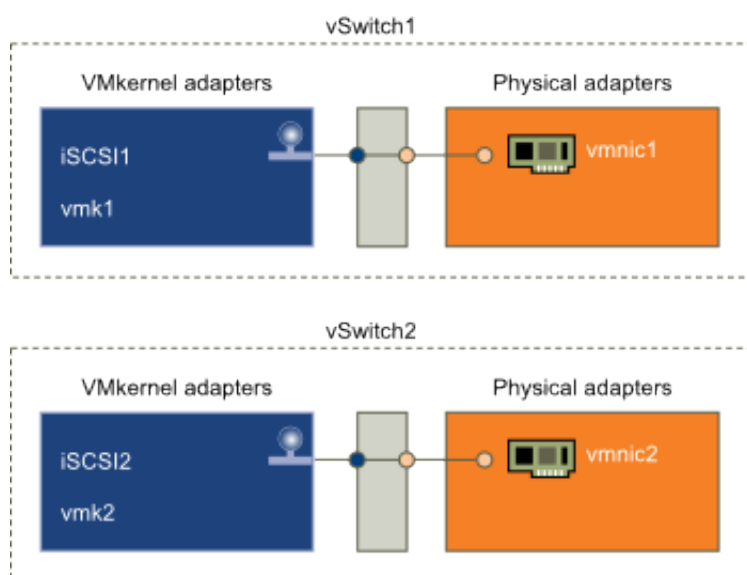
Figure 99: 1:1 Adapter Mapping on Separate vSphere Standard Switches
