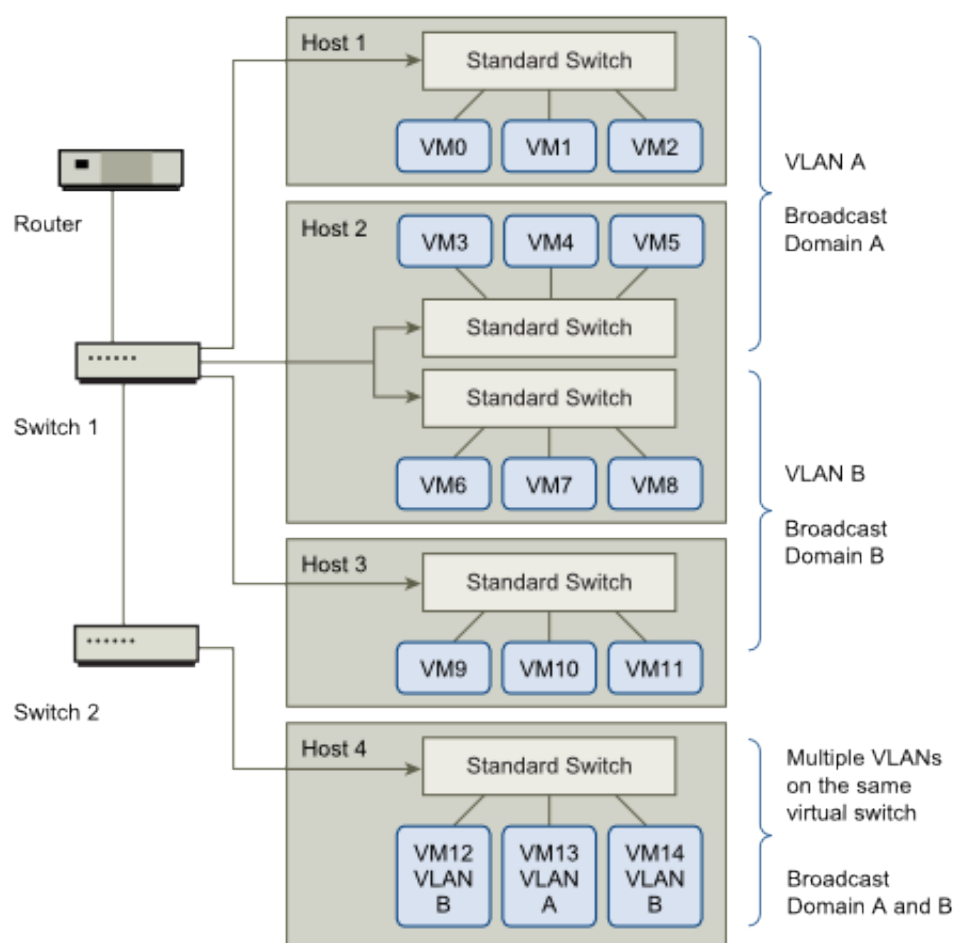
Figure 123: Sample VLAN Layout
