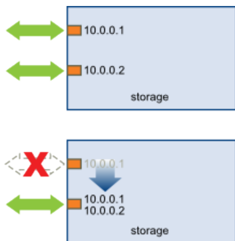
Figure 105: Port Reassignment
