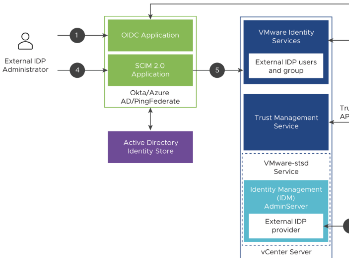
Figure 61: vCenter Server Identity Provider Federation Configuration Process Flow using VMware Identity
