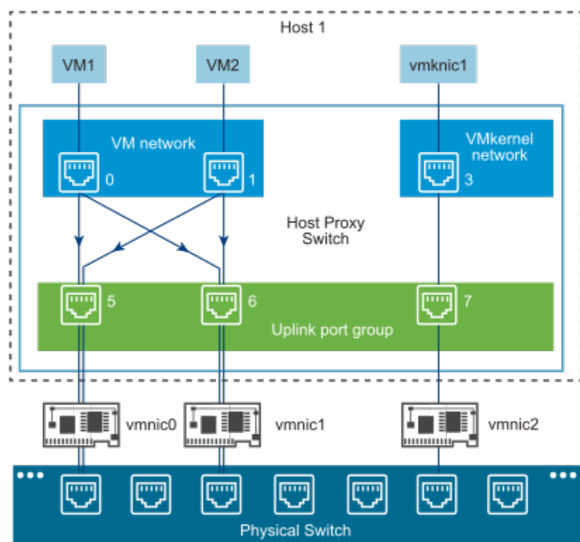
Figure 71: Packet Flow on the Host Proxy Switch
