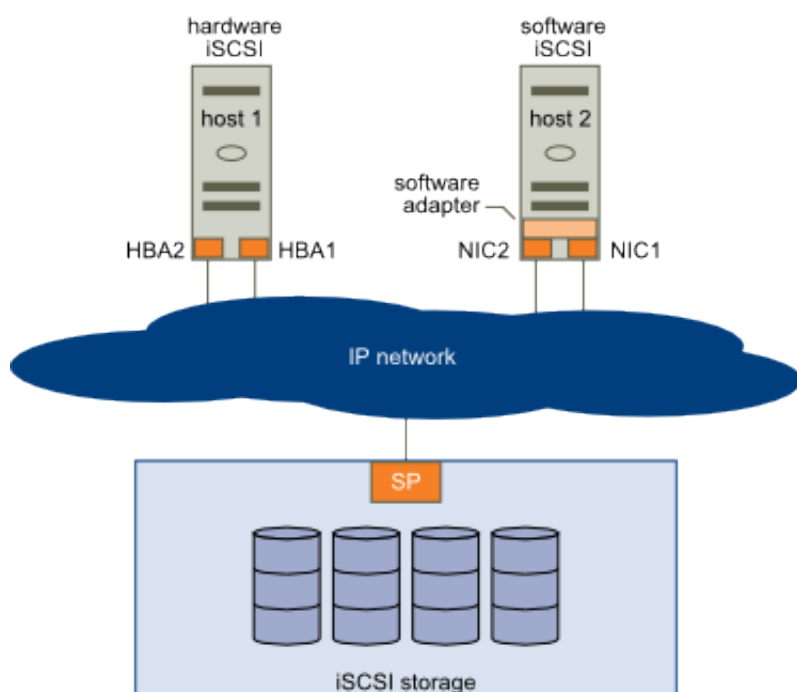
Figure 103: Host-Based Path Failover
