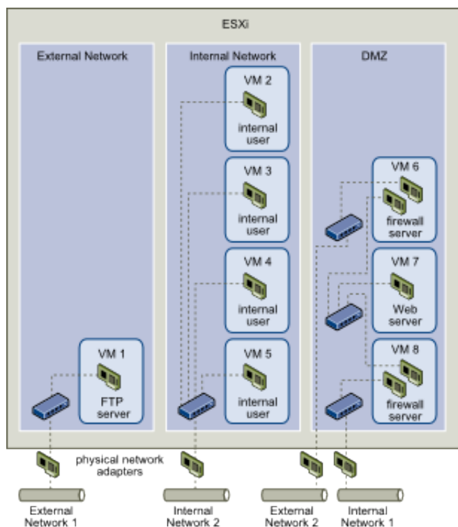
Figure 124: External Networks, Internal Networks, and a DMZ Configured on a Single ESXi Host
