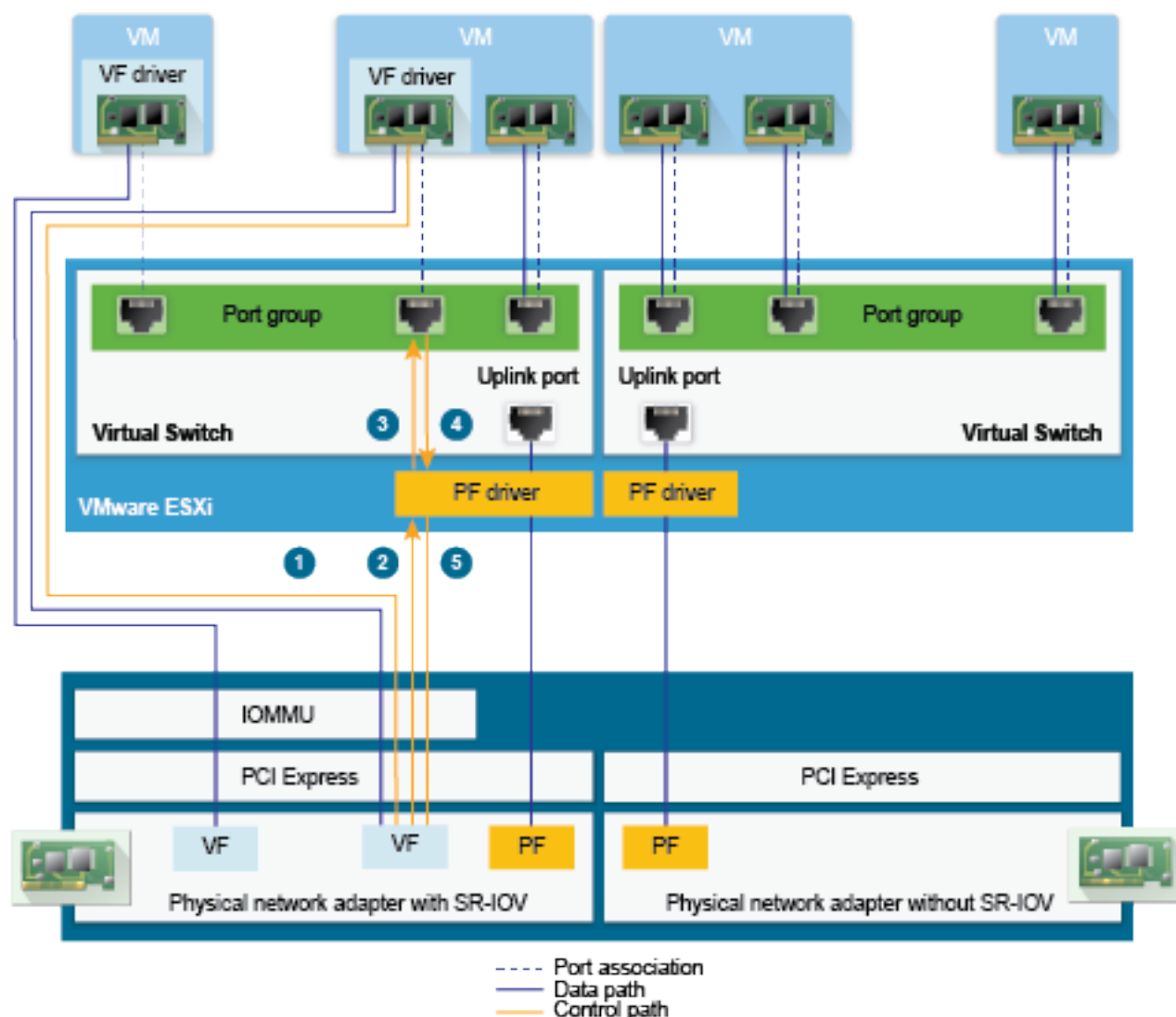
Figure 84: Data and Configuration Paths in the SR-IOV Support of vSphere
