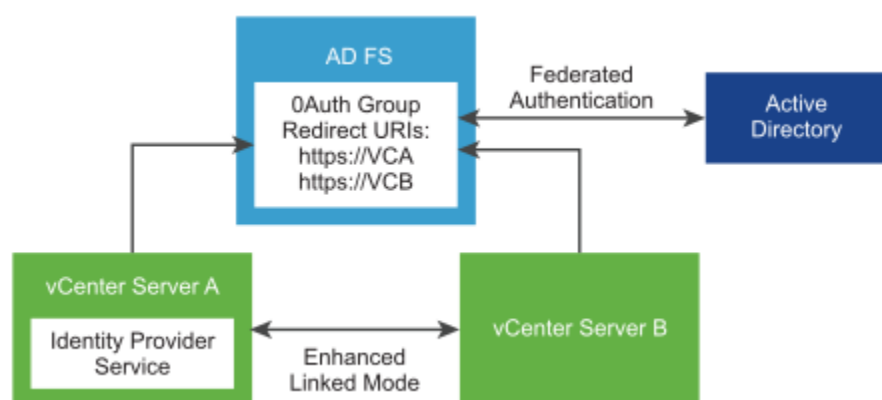
Figure 58: Enhanced Linked Mode and AD FS Identity Provider Federation
