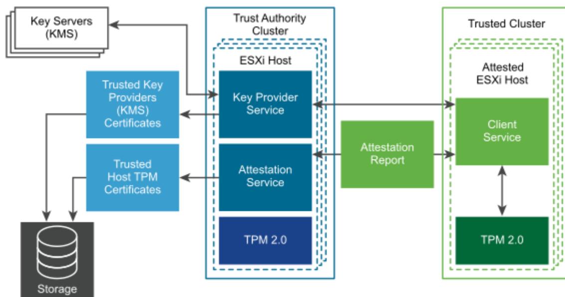
Figure 119: vSphere Trust Authority Services
