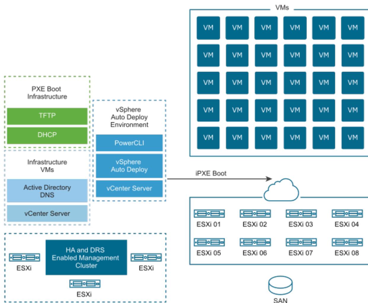
Figure 21: Highly Available vSphere Auto Deploy Infrastructure
