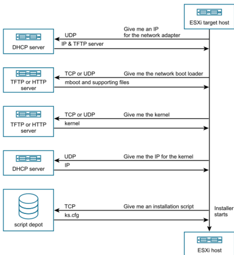
Figure 26: Overview of PXE Boot Installation Process
