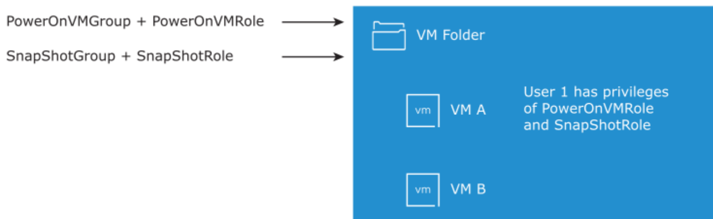
Figure 114: Example 1: Permission Inheritance from Multiple Groups
