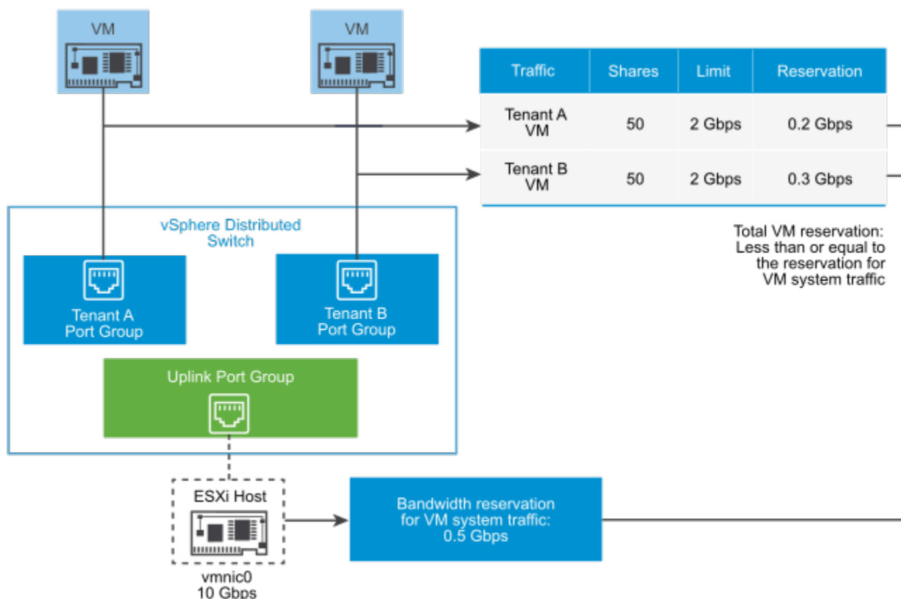
Figure 87: Configuration for Bandwidth Allocation for Individual Virtual Machines
