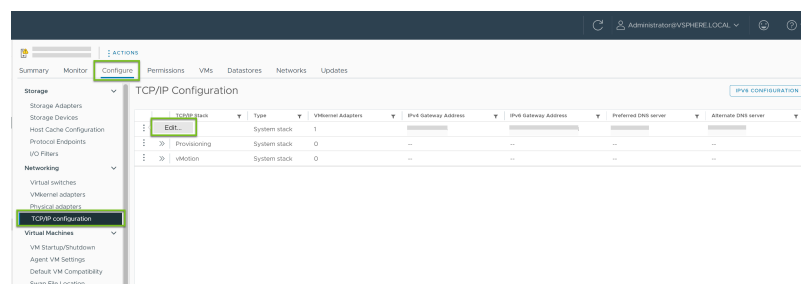
Figure 88: TCP/IP Configuration
