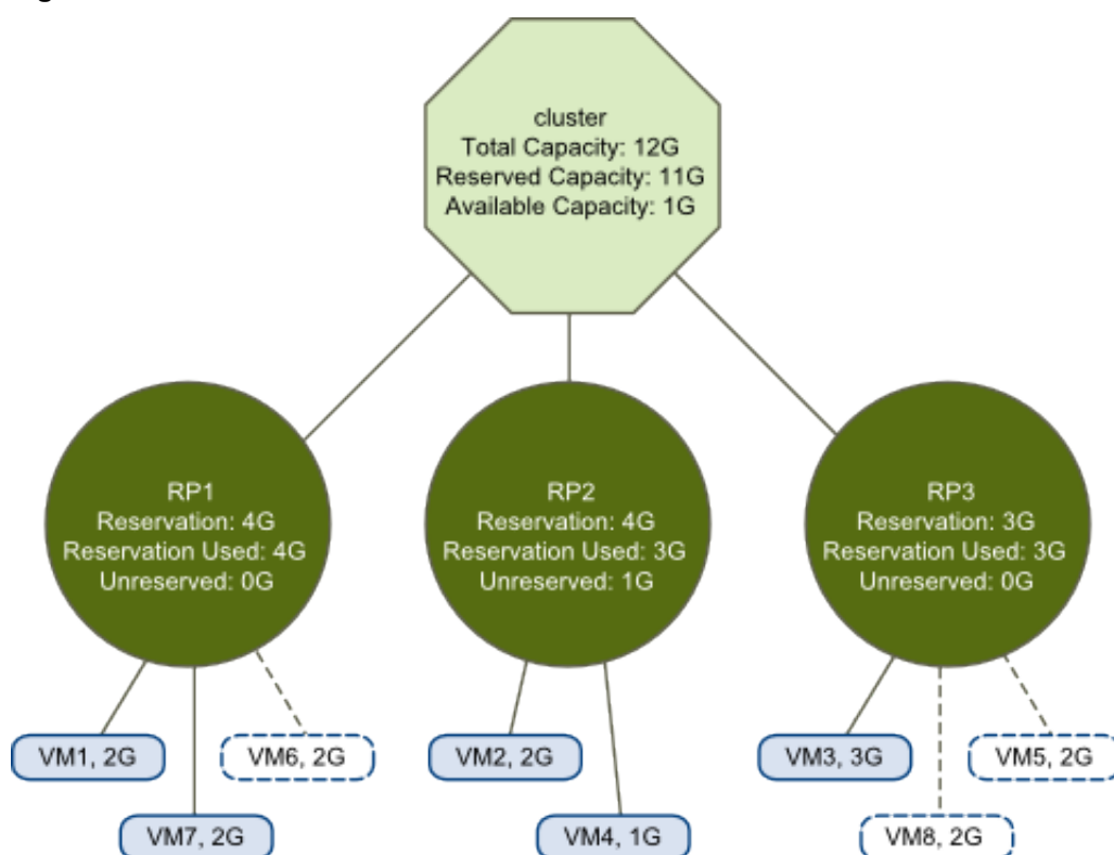
Figure 134: Valid Cluster with Fixed Resource Pools
