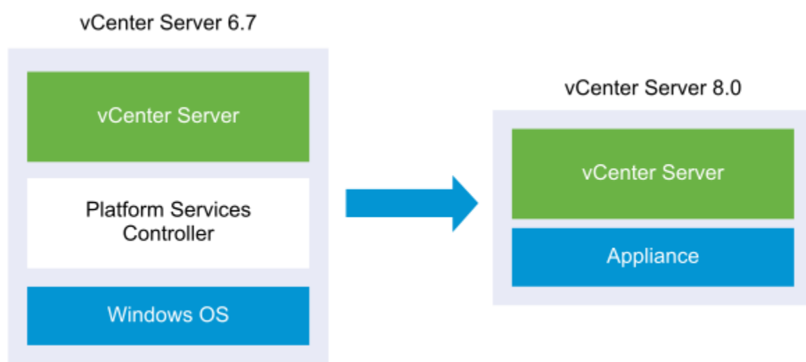
Figure 50: vCenter Server 6.7 with Embedded Platform Services Controller Deployment Before and After Migration
