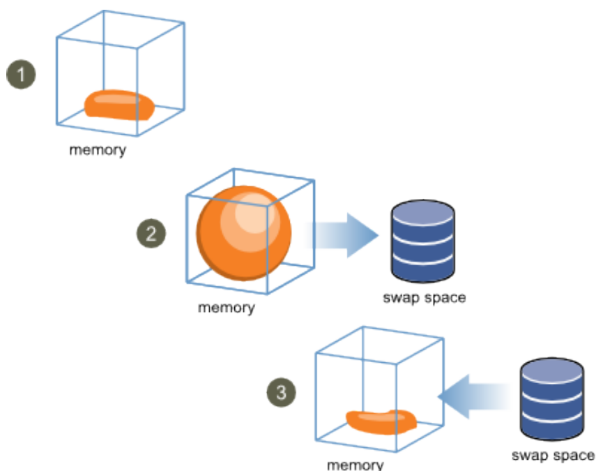
Figure 127: Memory Ballooning in the Guest Operating System
