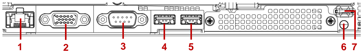
Figure 5. System Rear I/O
