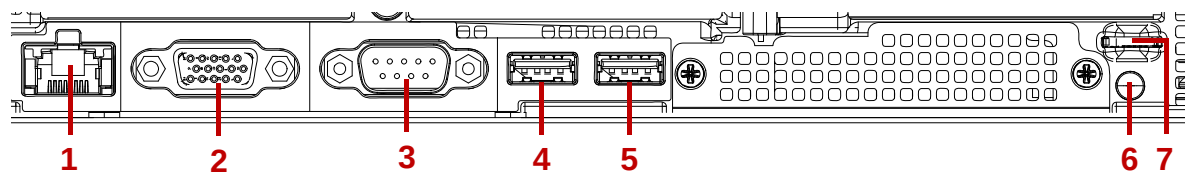
Figure 5. System Rear I/O
