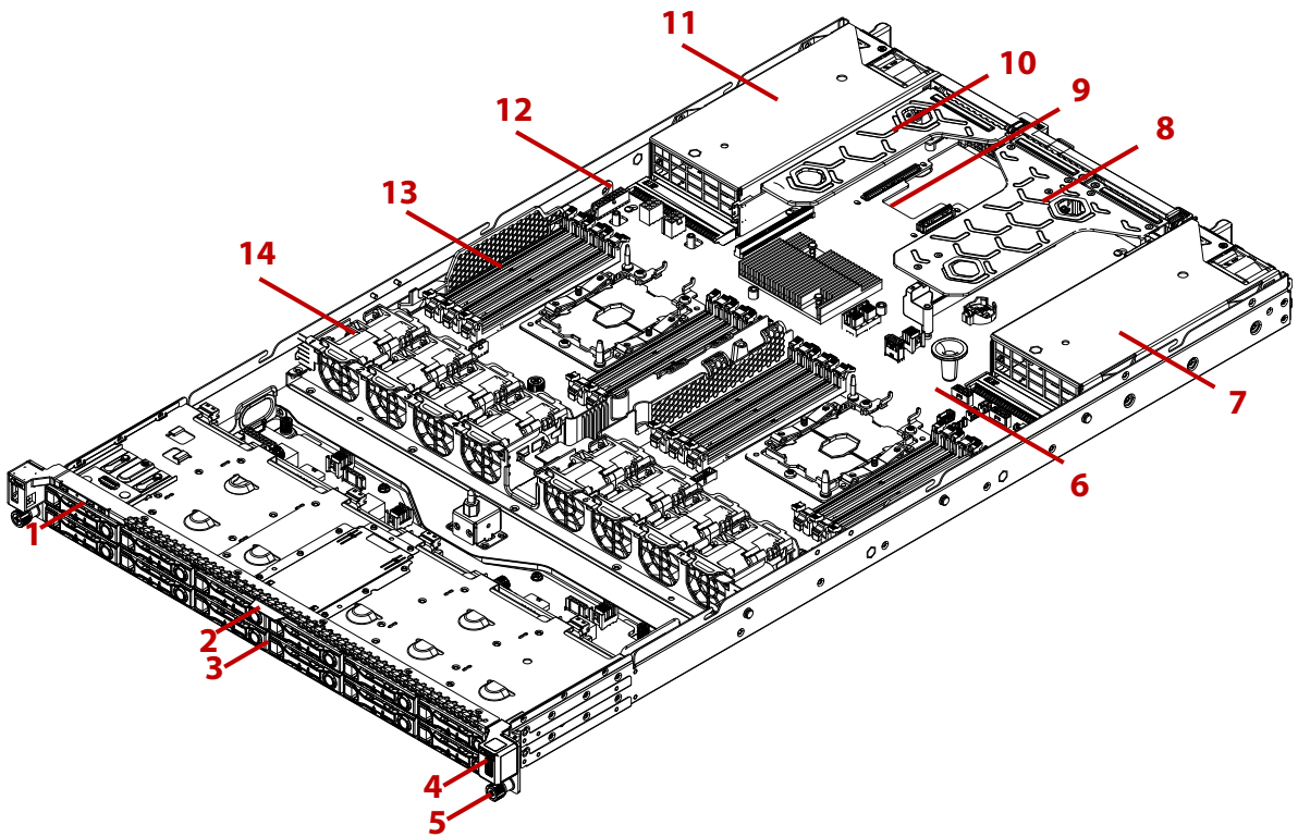
Figure 1. 2.5" Storage Drive System Component Overview
