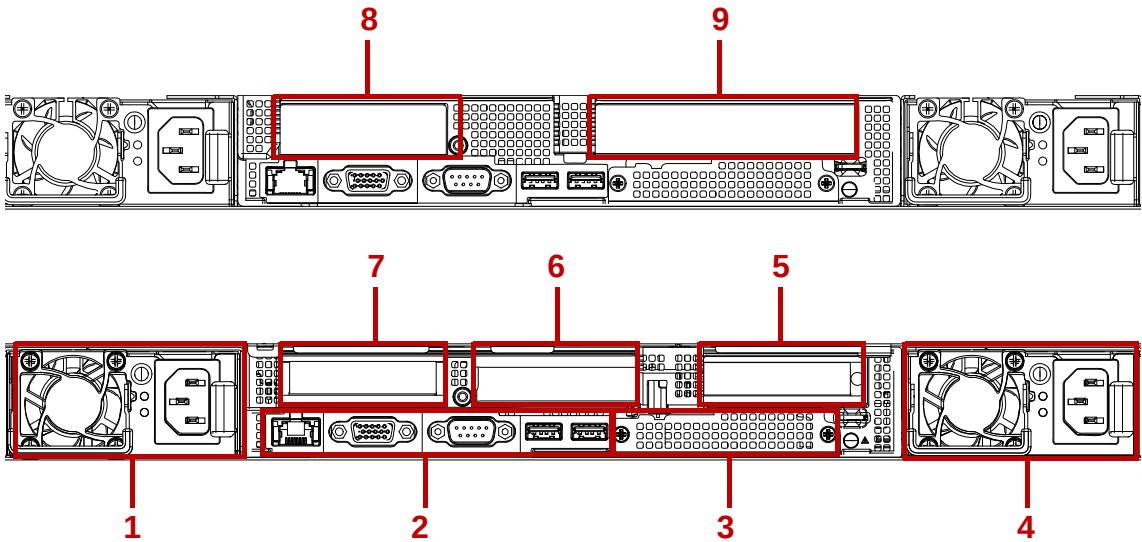
Figure 4. System Rear View
