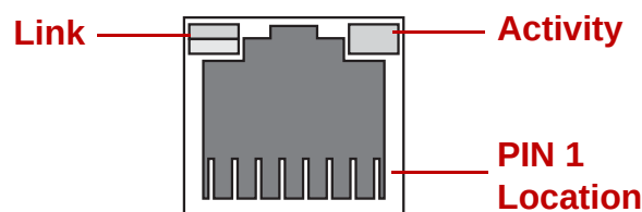
Figure 10. GbE RJ45 Management Port
