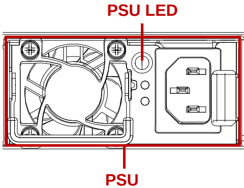
Figure 6. PSU to Mainboard Module Description
