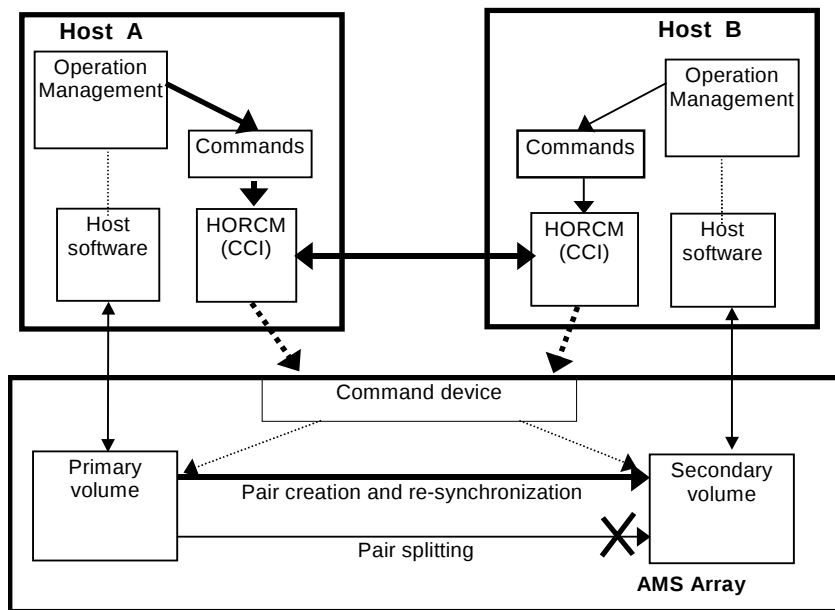
Figure 2-5: SnapShot System Configuration
