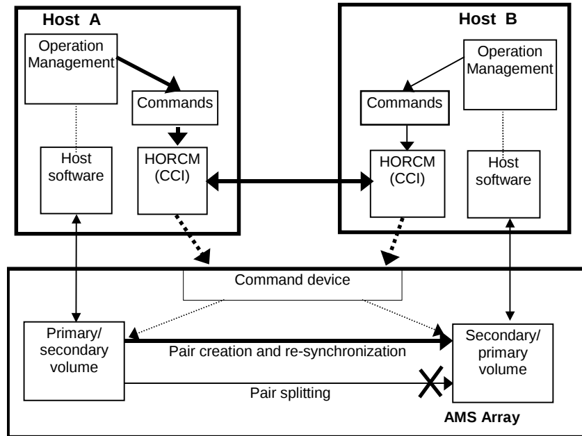
Figure 2-4: ShadowImage System Configuration
