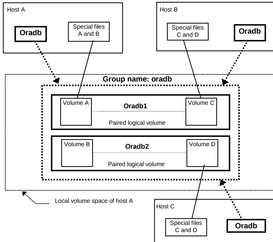
Figure 2-1: Paired Volumes
