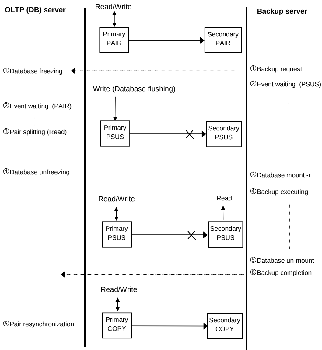
Figure 2-11: Backing Up S-VOL in Paired Status using TrueCopy/TCE
