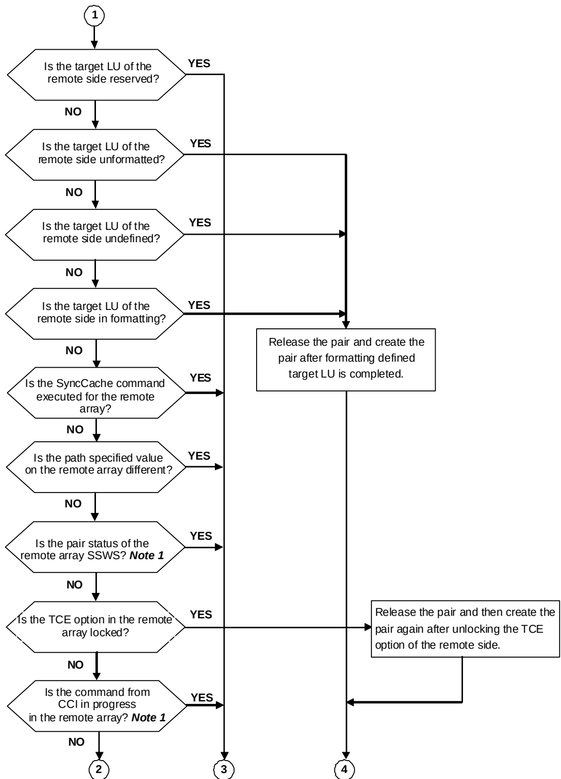
Figure 2-5: Pair Status Information Example Using TCE (continued)
