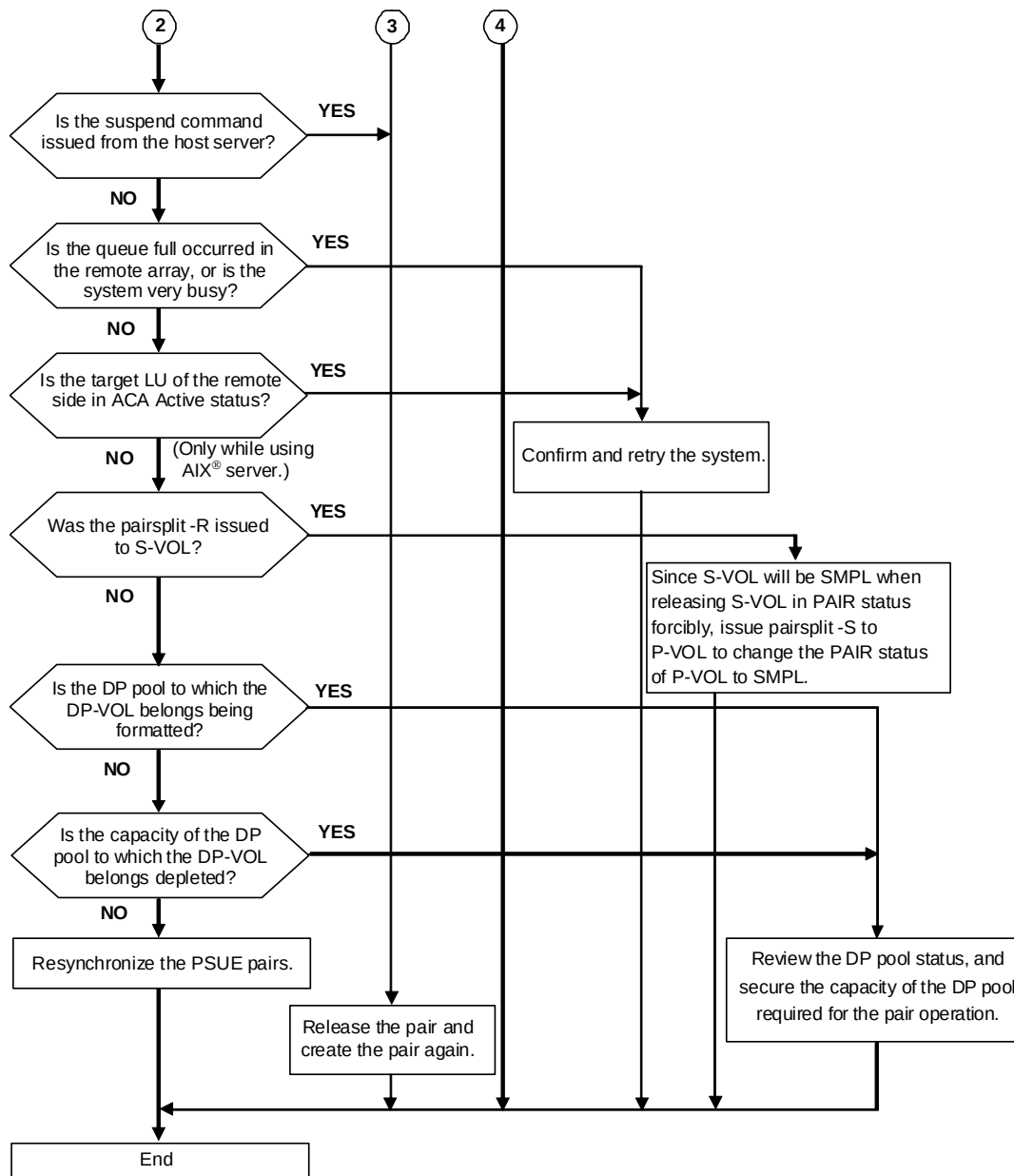
Figure 2-5: Pair Status Information Example Using TCE (continued)
