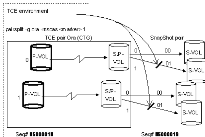
Figure 1-9: Example of -mscas Option for Pairsplit
