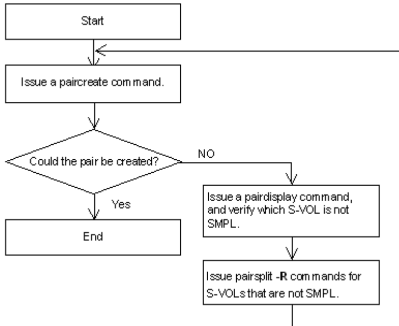
Figure 1-2: Pair Creation Operation
