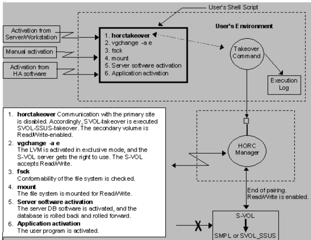
Figure 1-36: TrueCopy/TCE Takeover Example (UNIX® System)
