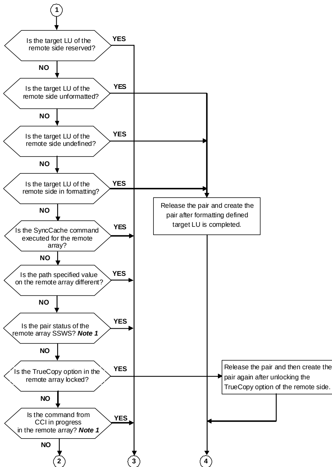
Figure 2-3: Pair Status Information Example Using TrueCopy (continued)
