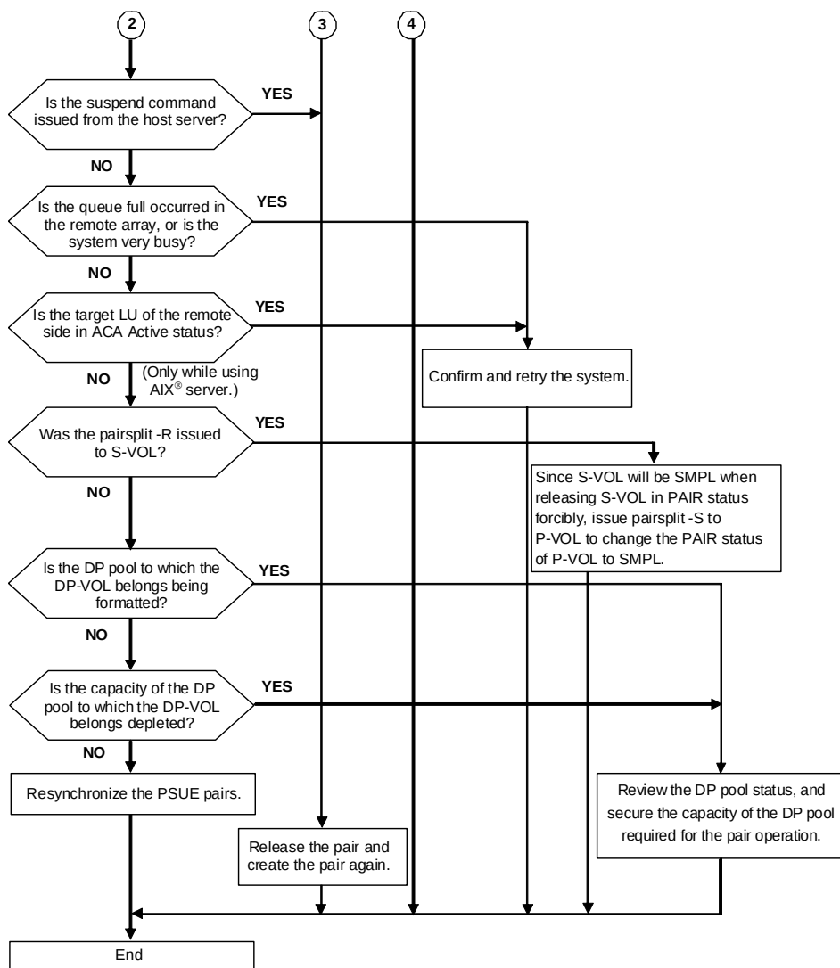
Figure 2-3: Pair Status Information Example Using TrueCopy (continued)
