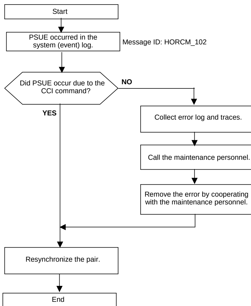
Figure 2-2: Pair Status Information Example Using SnapShot
