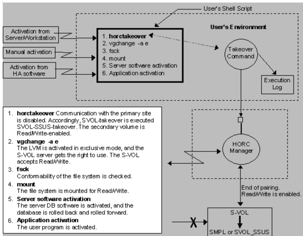
Figure 1-37: TrueCopy/TCE Takeover Example (Windows System)
