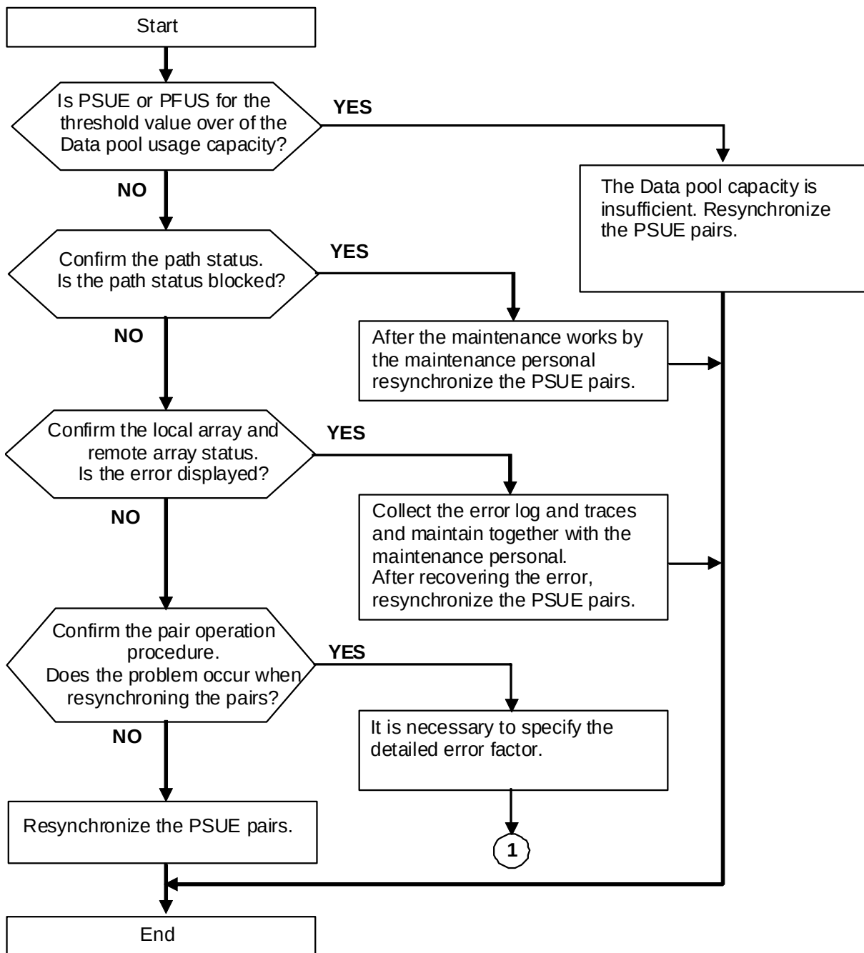
Figure 2-5: Pair Status Information Example Using TCE
