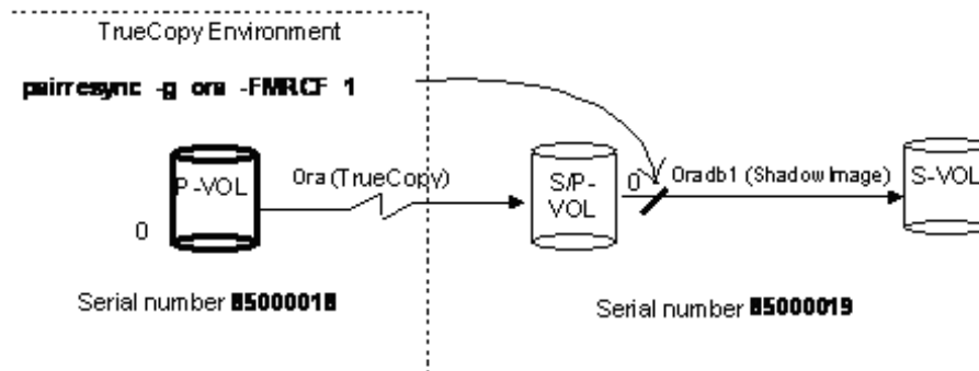
Figure 1-17: Example of -FMRCF Option for Pairresync
