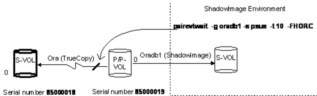
Figure 1-21: Example of -FHORC Option for Pairevtwait
