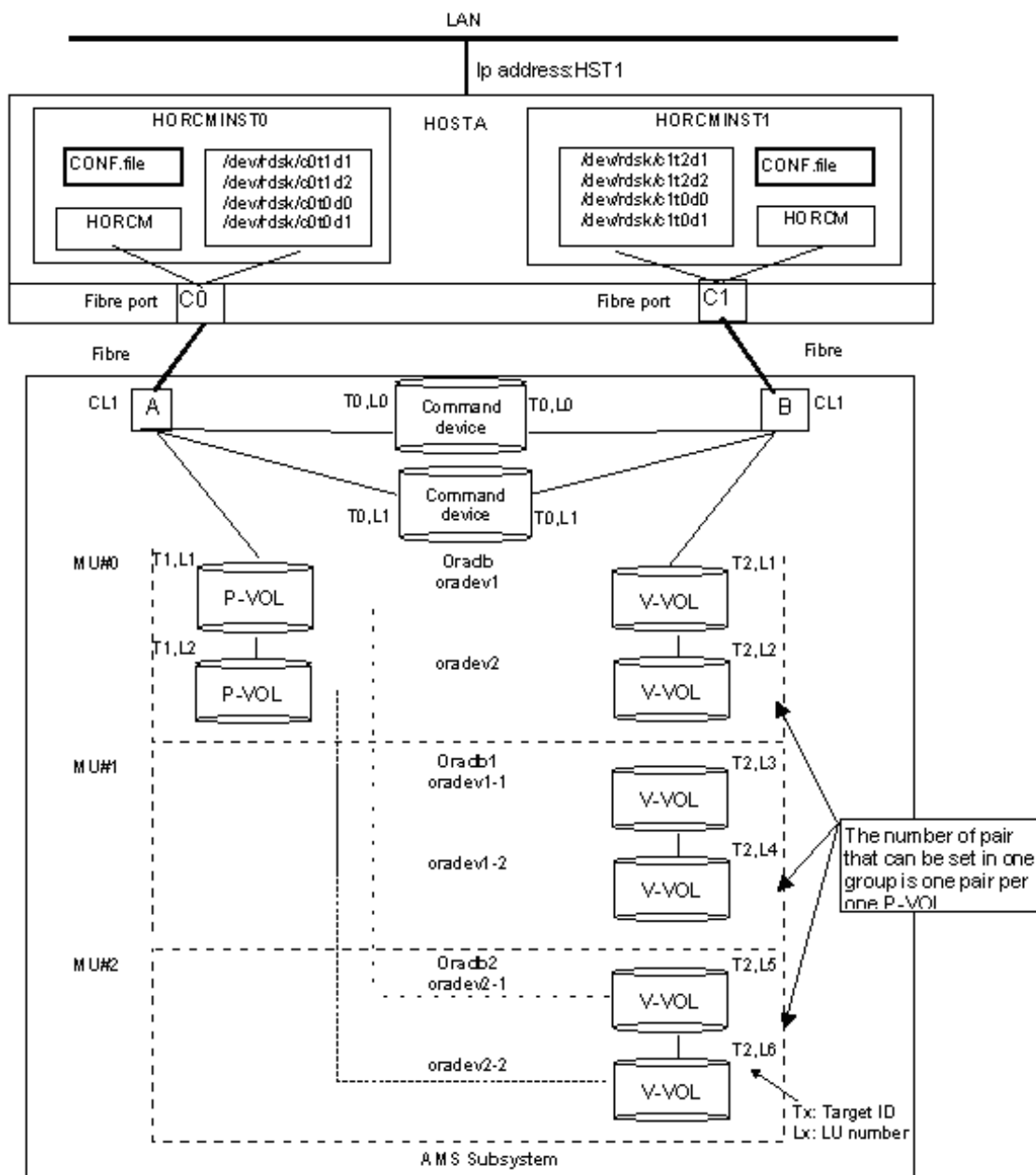
Figure 1-4: Paircreate Command -m Option (Correct Example)
