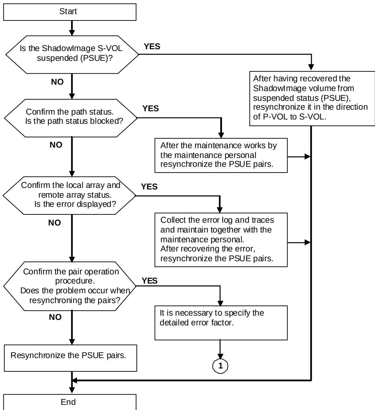
Figure 2-3: Pair Status Information Example Using TrueCopy
