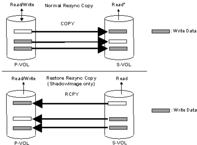
Figure 1-13: Pair Resynchronization
