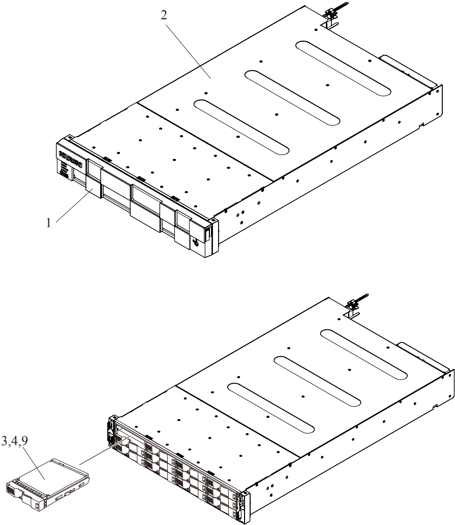
Figure 2-22 CBXSL (1/2)
