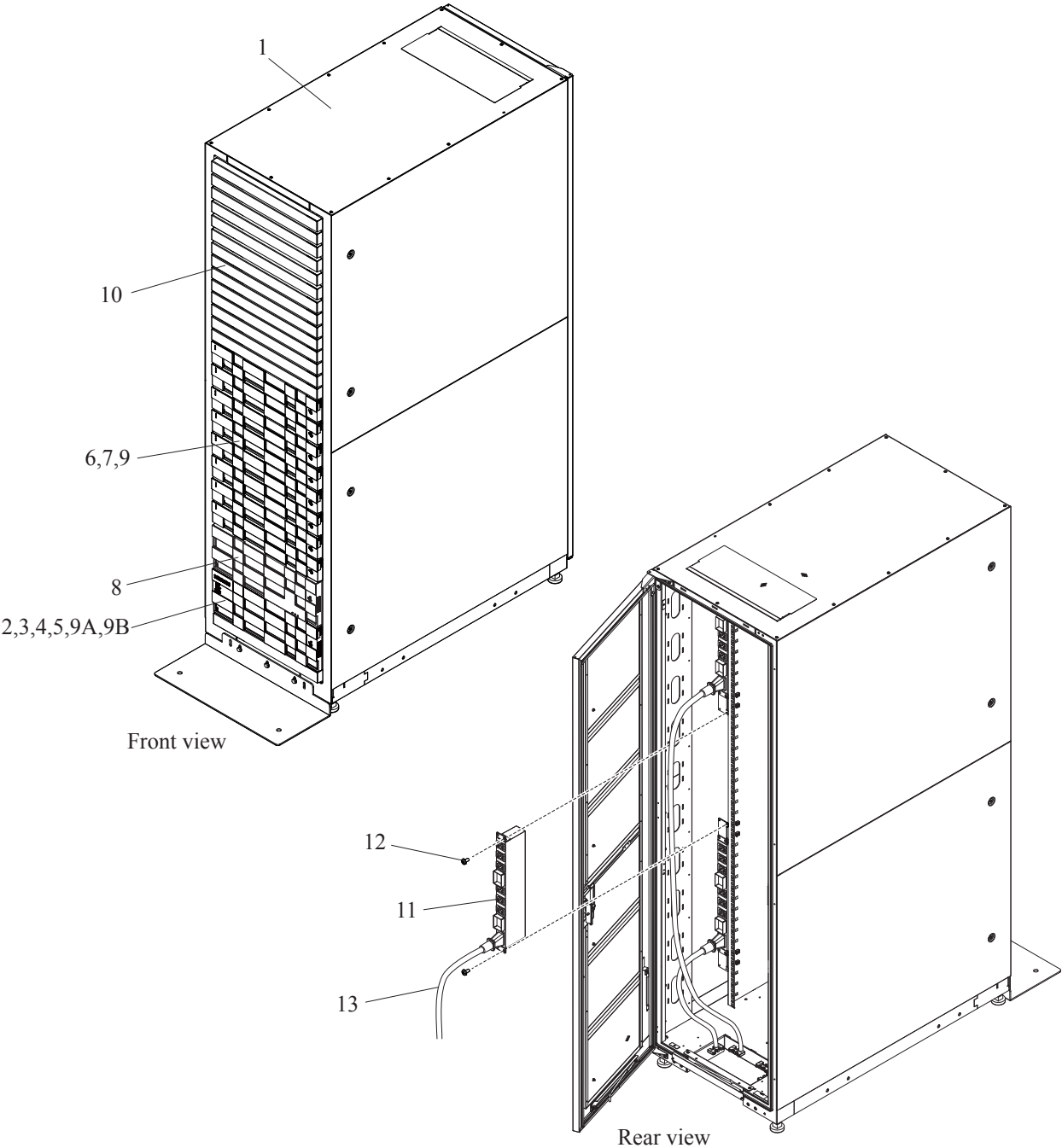
Figure 2-17 RKU Rack Frame
