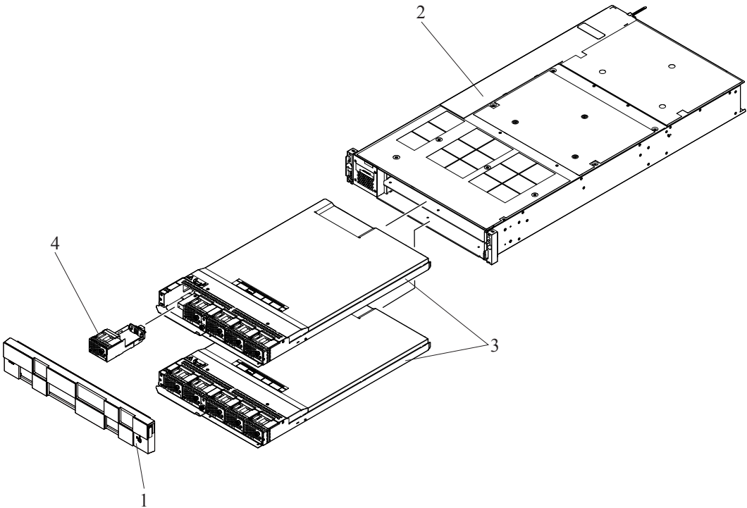
Figure 2-19 CHBB (2/2)
