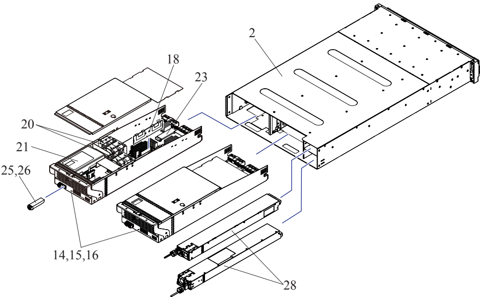
Figure 2-21 CBXSS (2/2)
