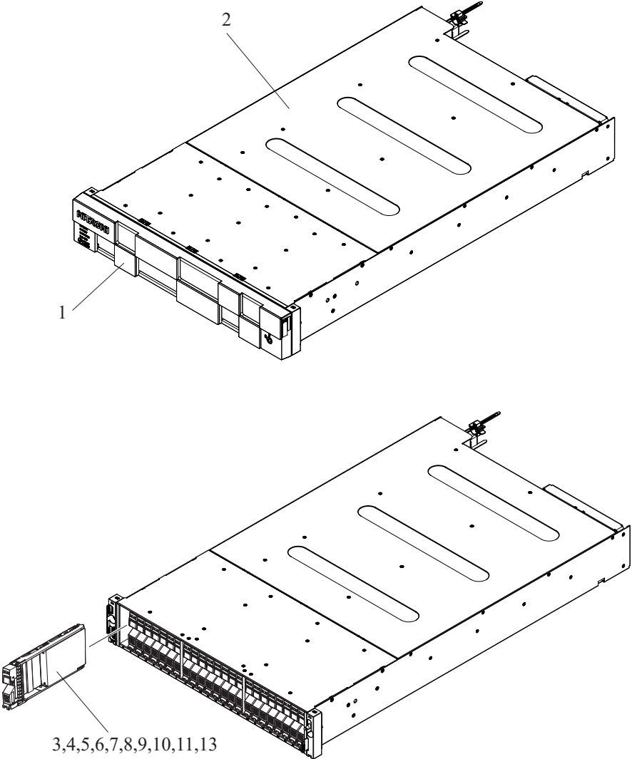
Figure 2-20 CBXSS (1/2)
