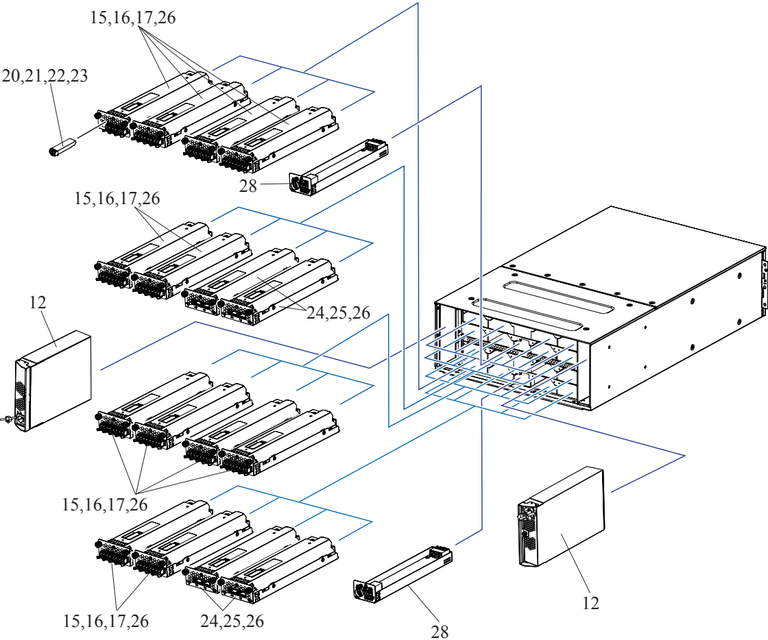
Figure 2-6 CBLH1 (2/2)
