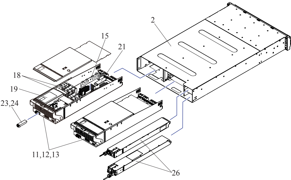
Figure 2-23 CBXSL (2/2)
