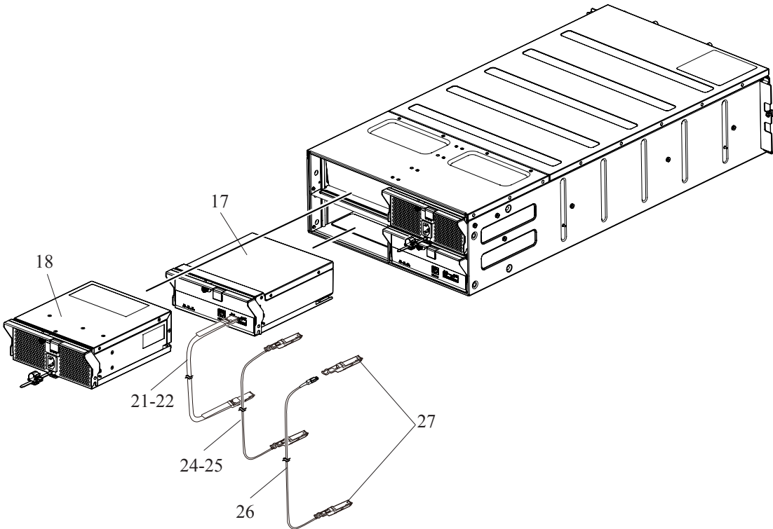
Figure 2-28 DB60 (2/2)
