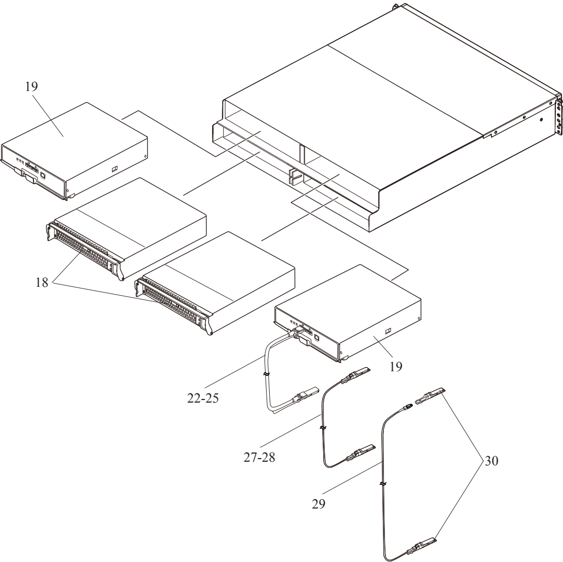
Figure 2-24 DBSC (2/2)
