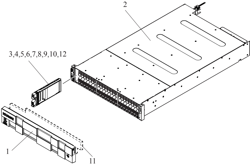
Figure 2-3 CBSSD (1/2)
