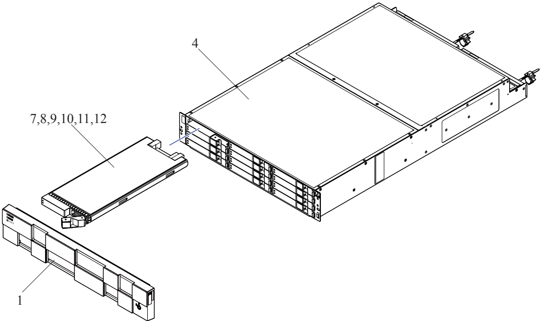
Figure 2-31 DBF (1/2)
