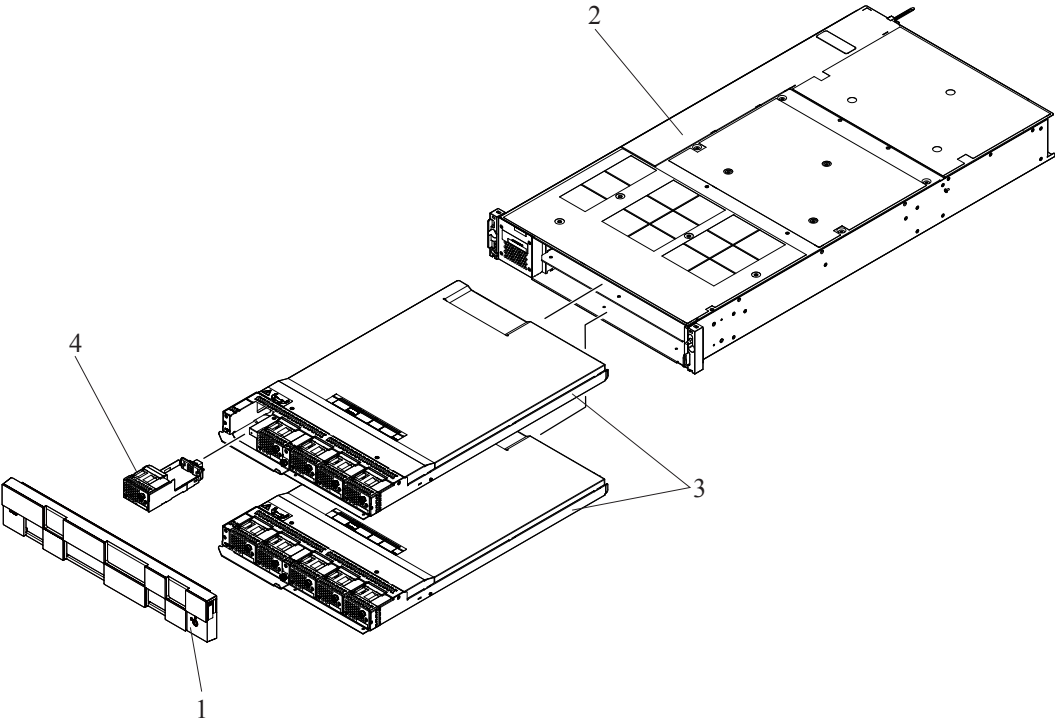
Figure 2-36 CHBB (2/2)
