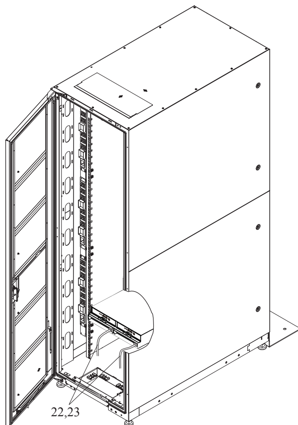
Figure 2-34 RKU Rack Frame (2/2)
