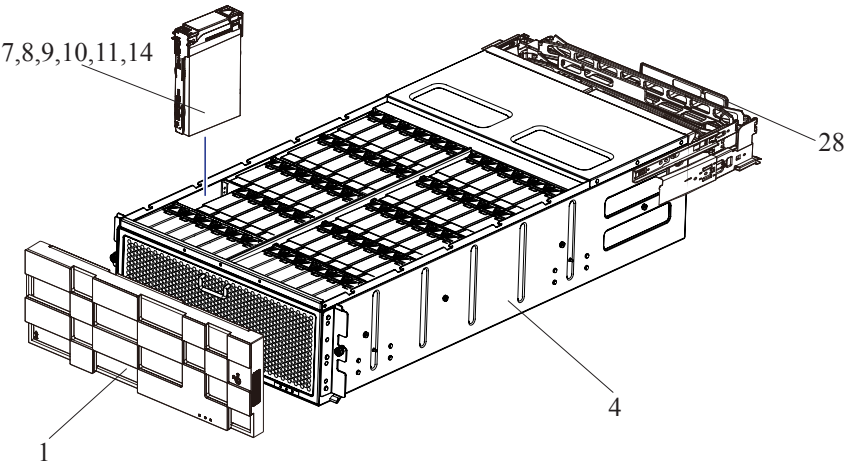
Figure 2-29 DB60C (1/2)
