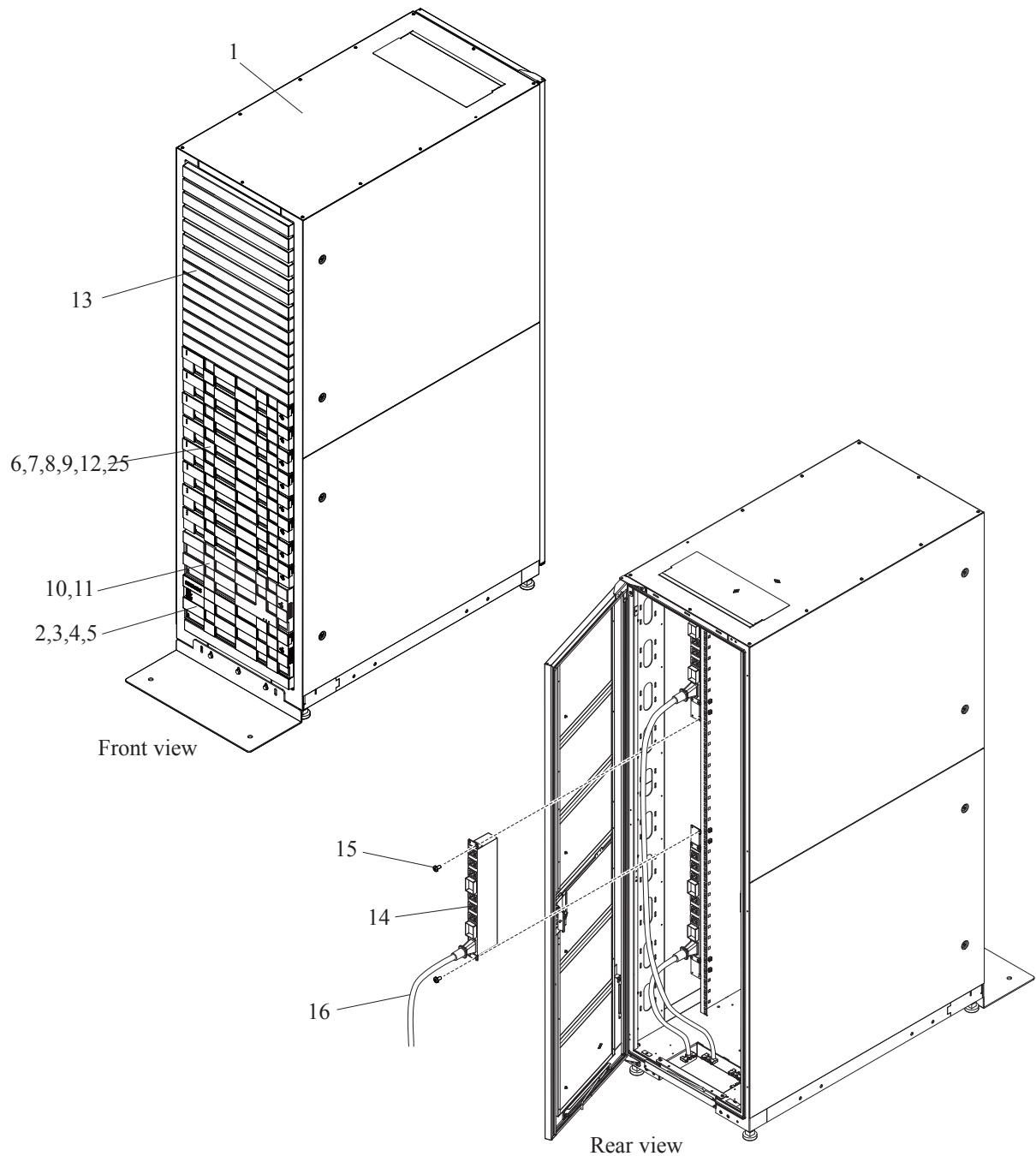
Figure 2-33 RKU Rack Frame (1/2)
