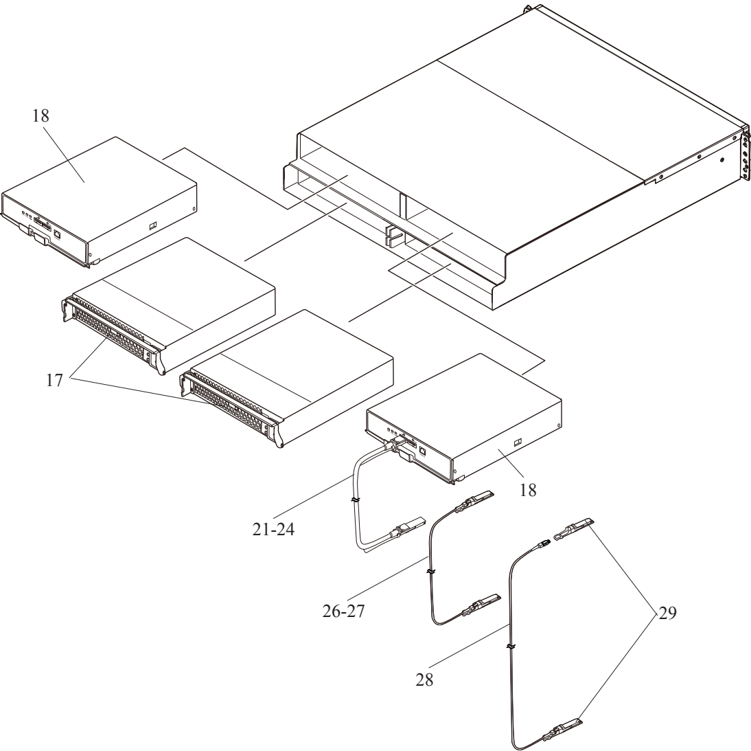
Figure 2-18 DBLC (2/2)
