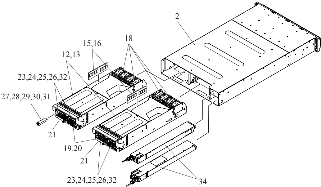
Figure 2-6 CBSL (2/2)
