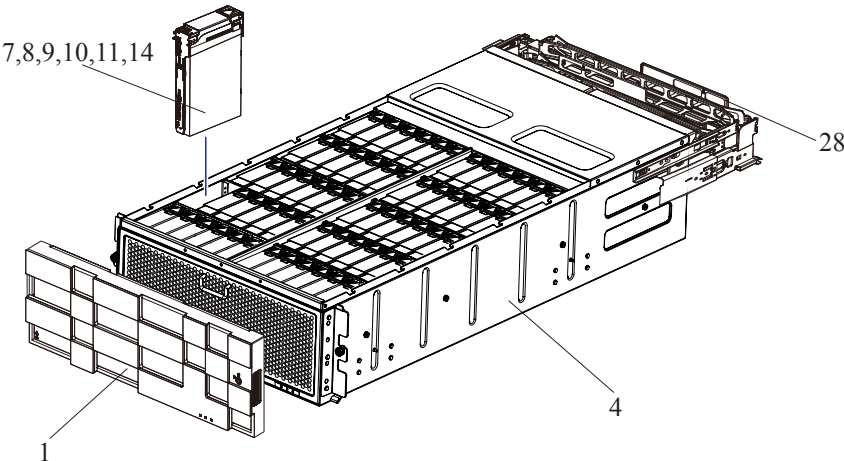
Figure 2-27 DB60 (1/2)
