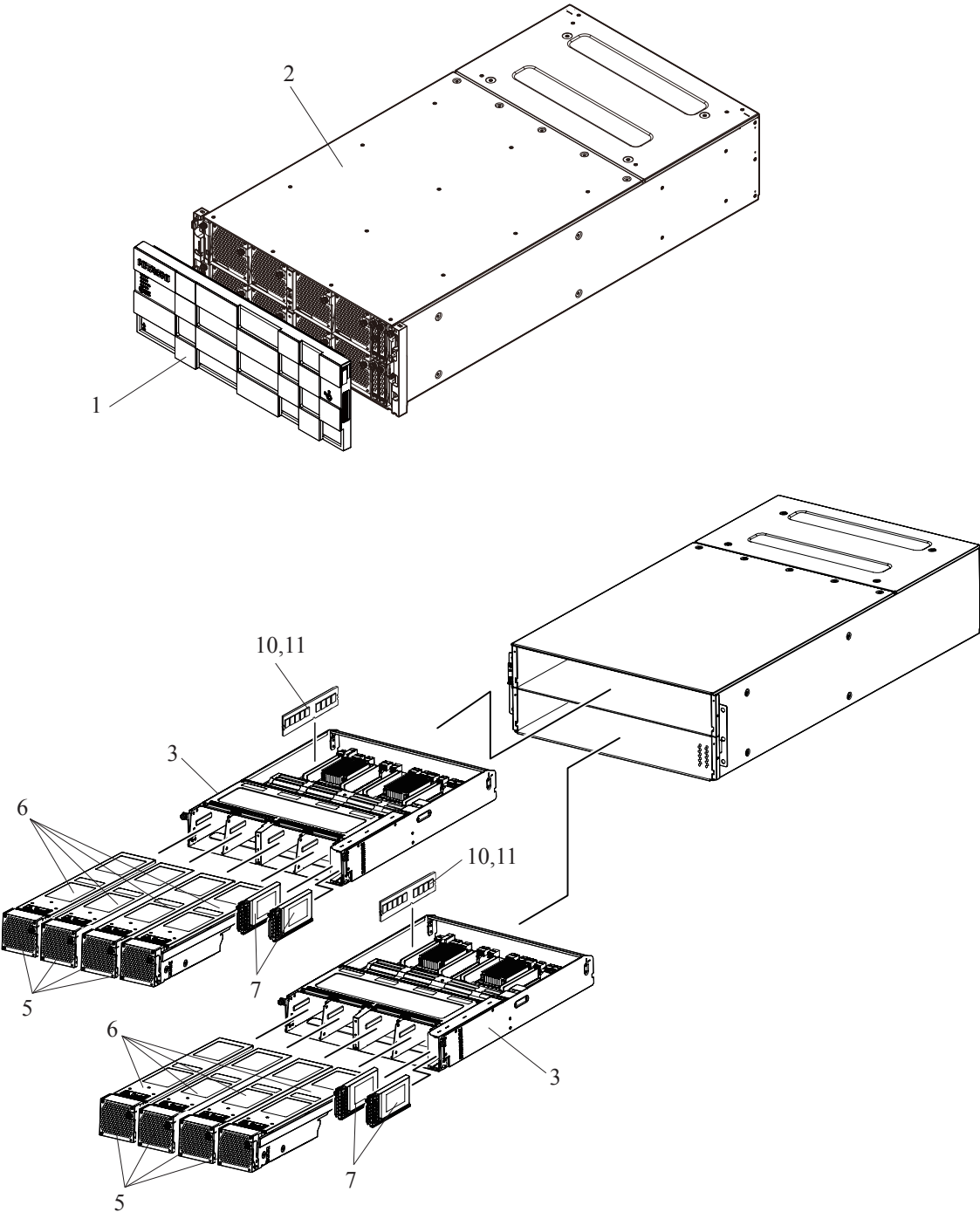
Figure 2-9 CBLM (1/3)
