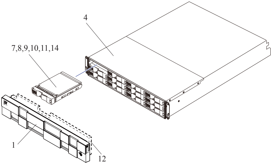
Figure 2-19 DBLD (1/2)
