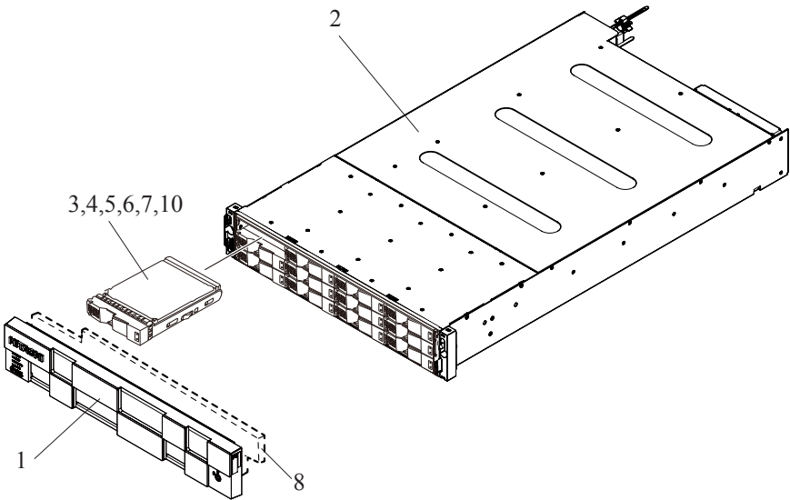
Figure 2-7 CBSLD (1/2)
