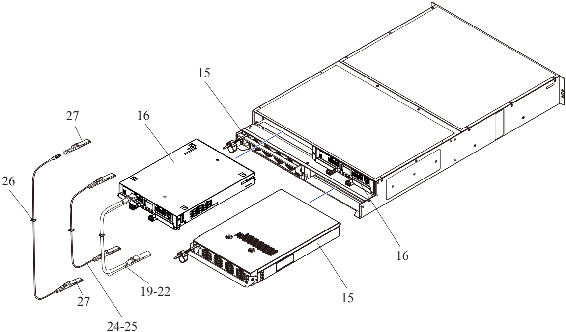
Figure 2-38 DBF2 (2/2)
