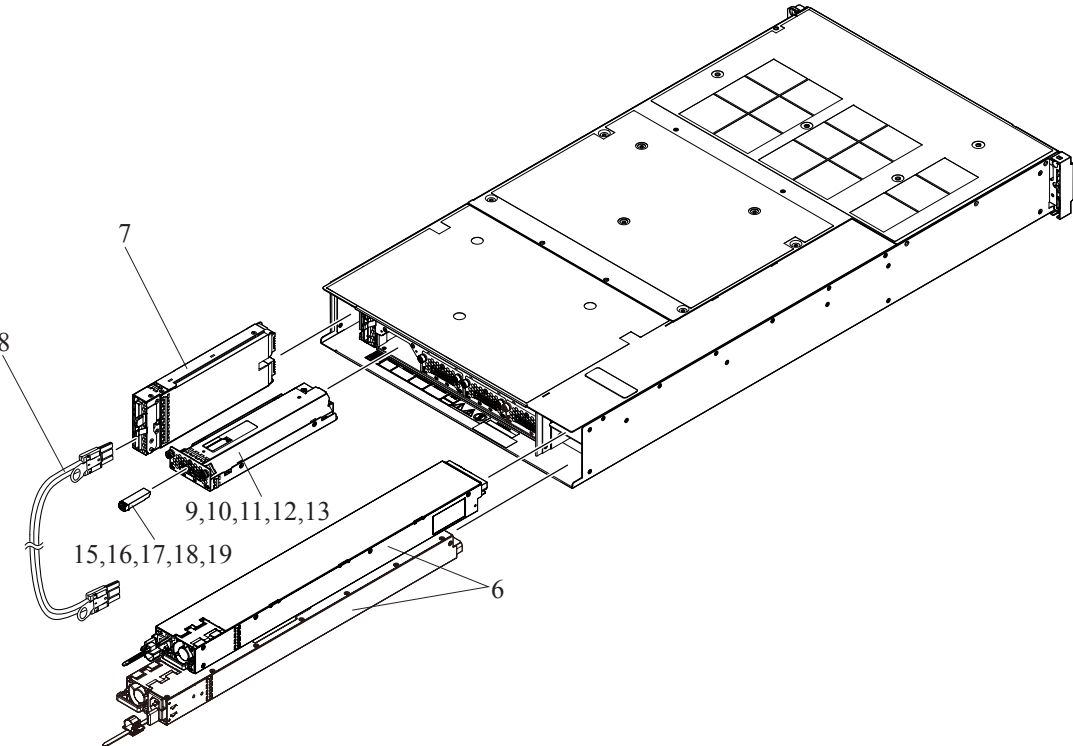
Figure 2-36 CHBB (2/2)
