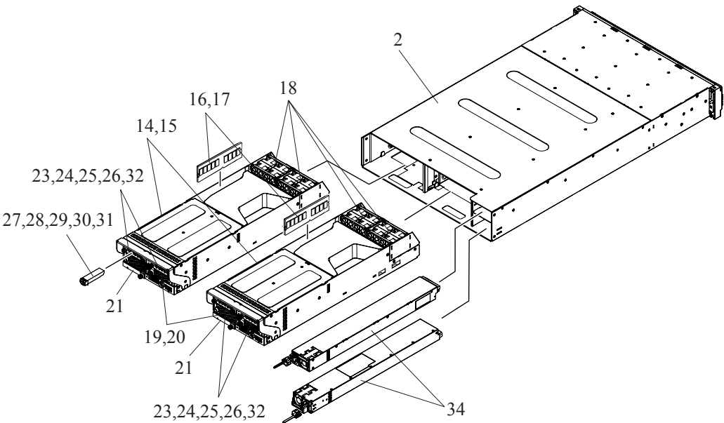
Figure 2-2 CBSS (2/2)
