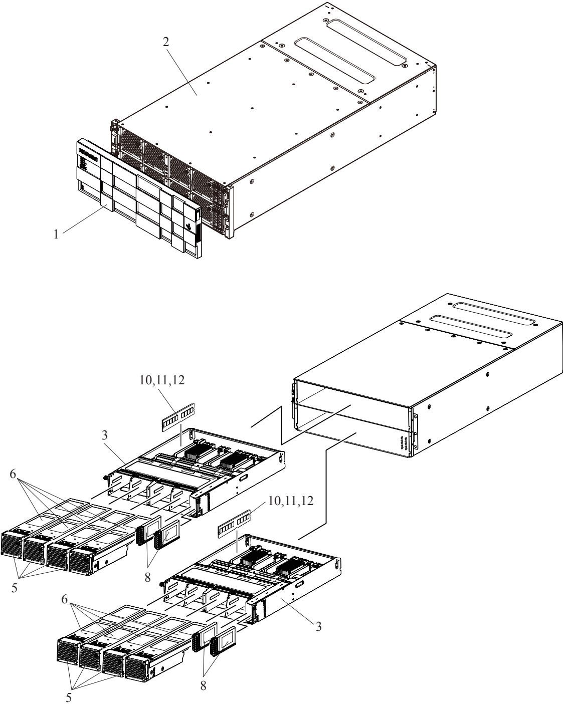
Figure 2-12 CBLH (1/3)
