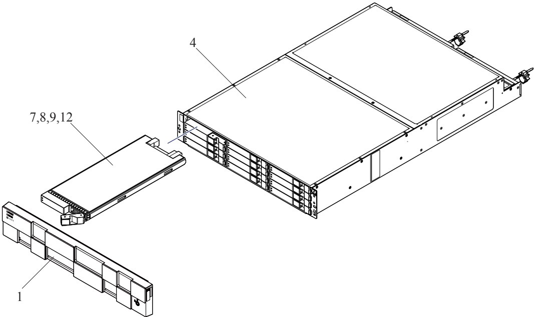
Figure 2-37 DBF2 (1/2)
