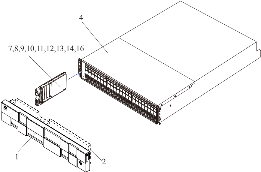
Figure 2-25 DBSD (1/2)
