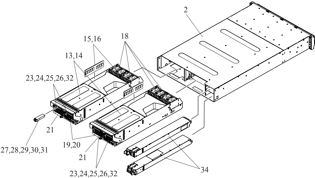
Figure 2-4 CBSSD (2/2)
