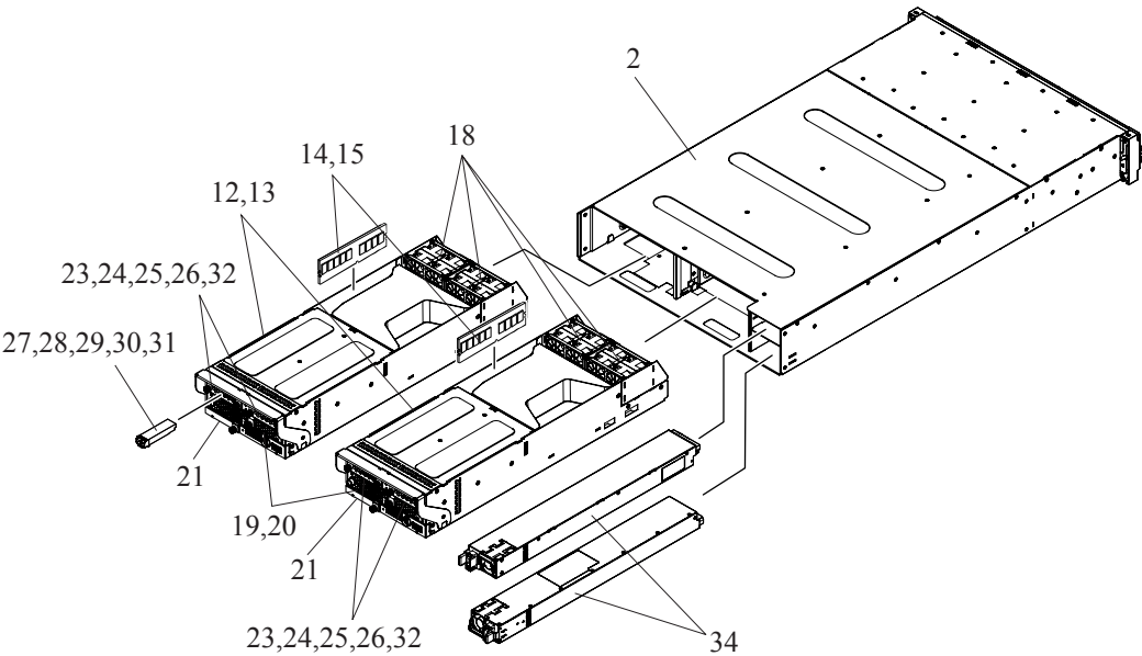
Figure 2-8 CBSLD (2/2)
