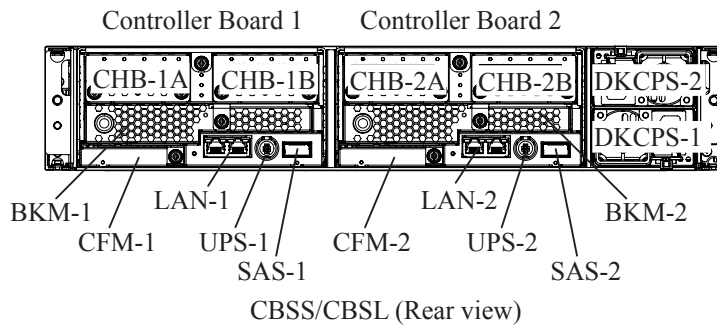
Figure 3-1 Parts Location of CBSS/CBSL/CBSSD/CBSLD
