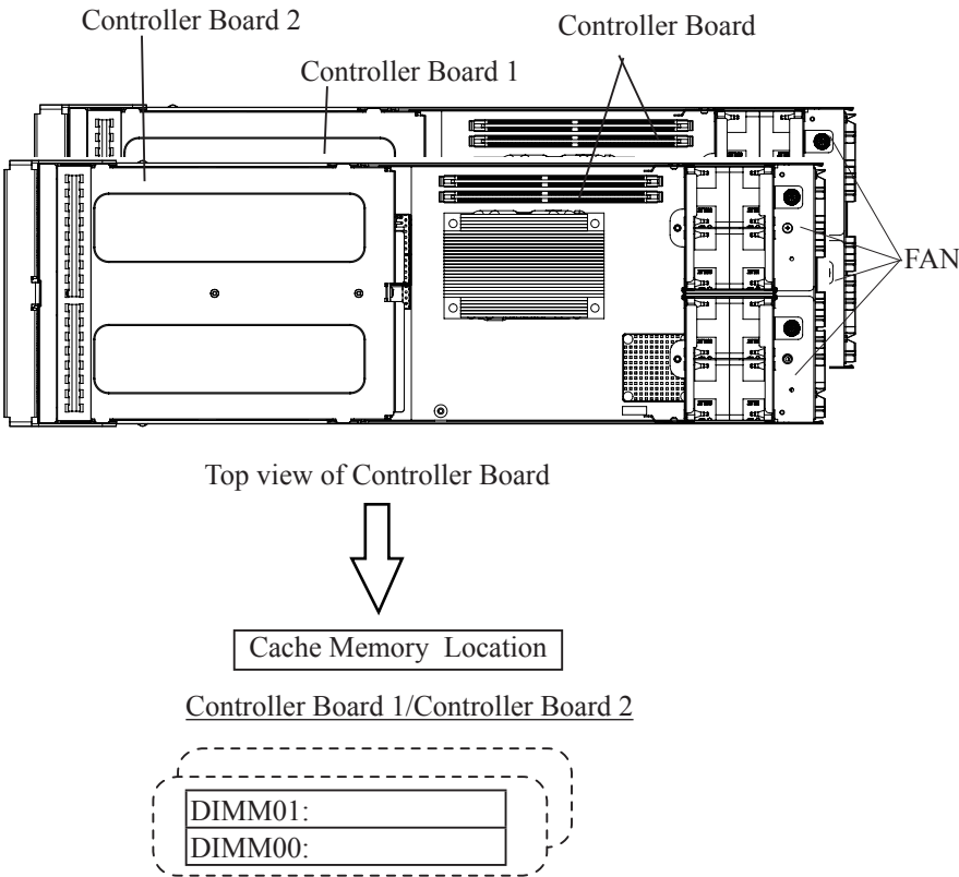
Figure 3-3 Cache Memory (CM) Location (CBSS/CBSL)
