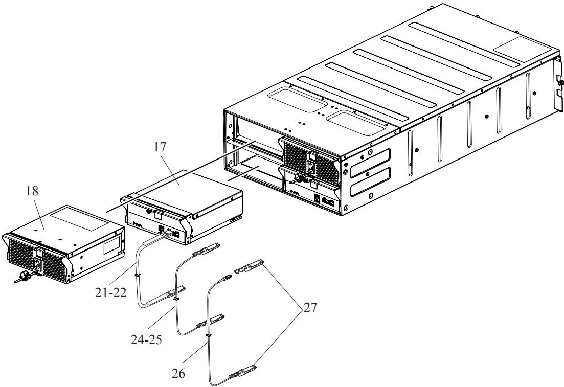
Figure 2-30 DB60C (2/2)
