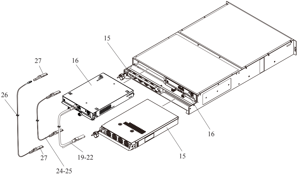
Figure 2-32 DBF (2/2)
