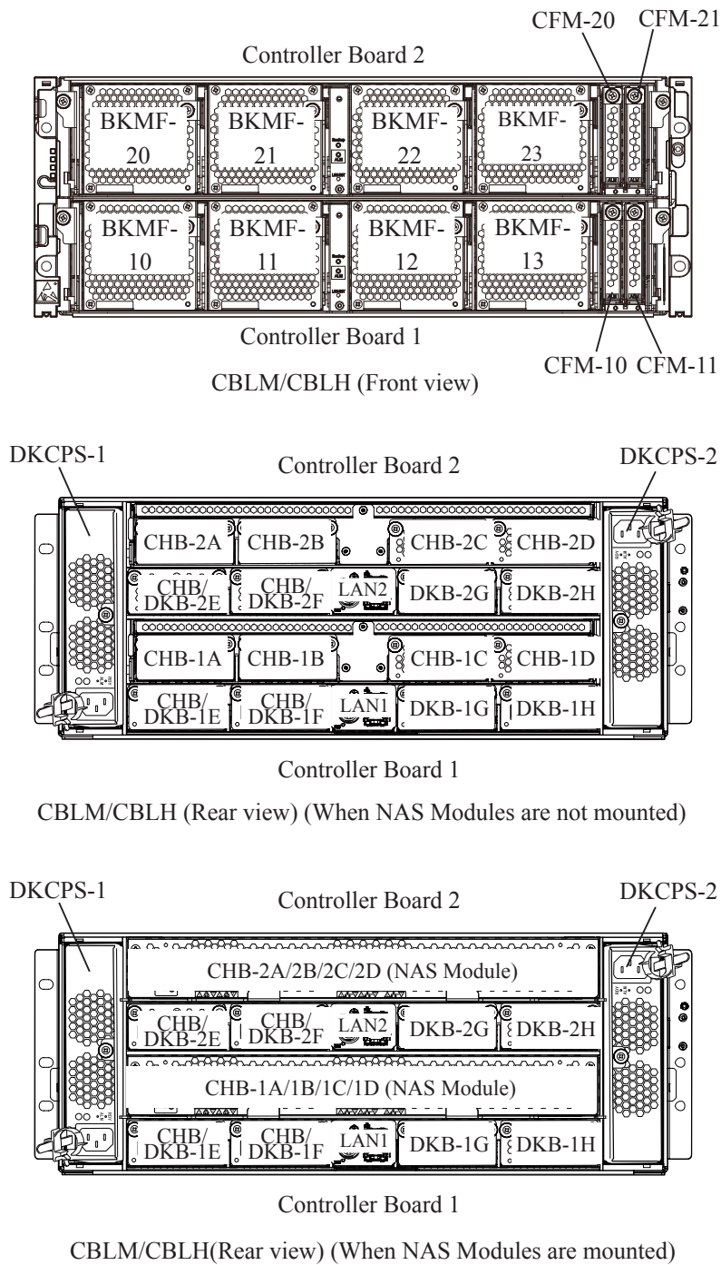
Figure 3-2 Parts Location of CBLM/CBLH
