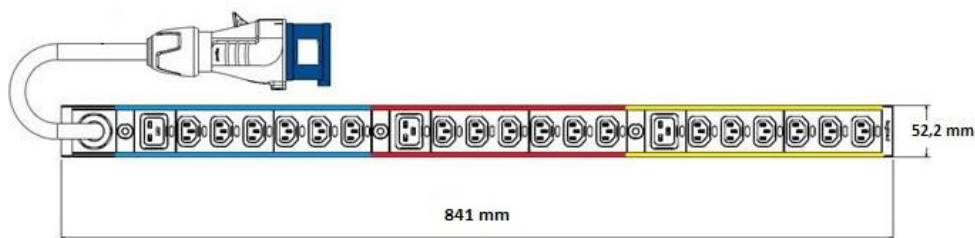
Figure 7 APAC and EMEA PDU for the Hitachi Universal V2 Rack (Single-phase 1P32A-18C13-3C19CE.P)
