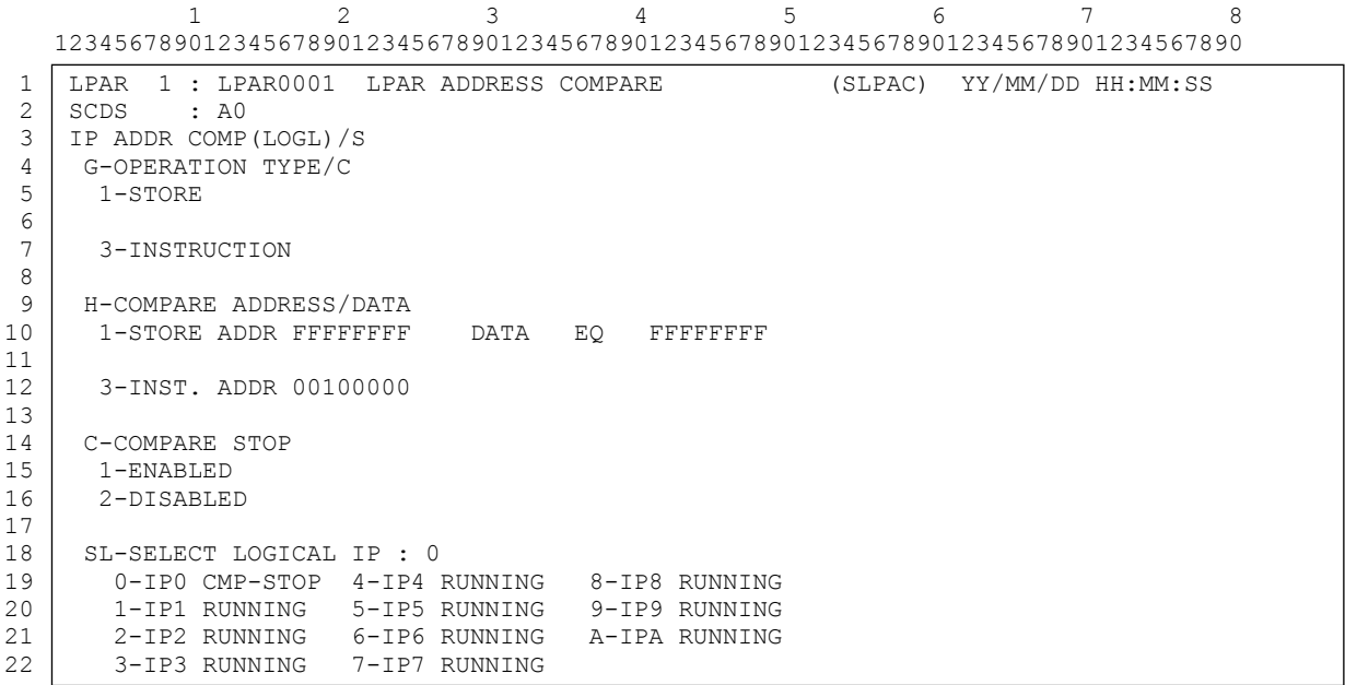
Figure 7-50 SLPAC Frame on C2000-xxA and C2000-xxB
