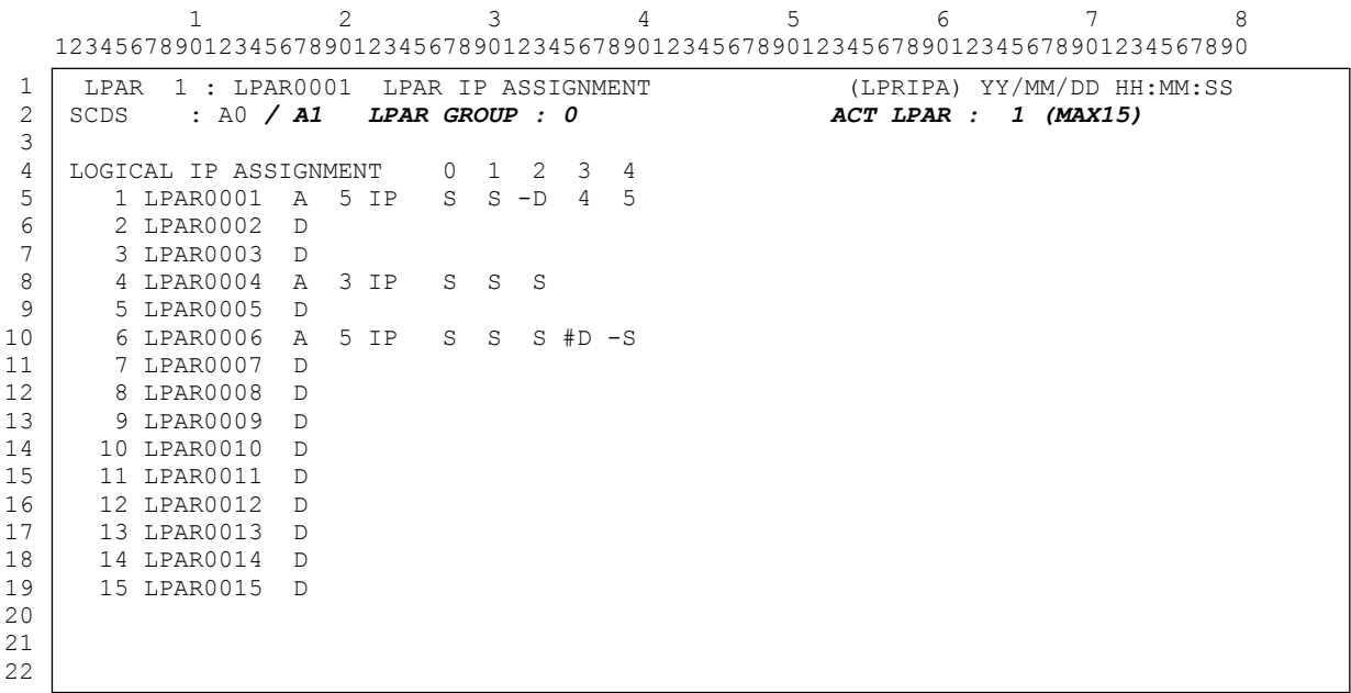
Figure 7-20 LPRIPA Frame on M3000 and C2000-xxC in MLPF 3.5.1
