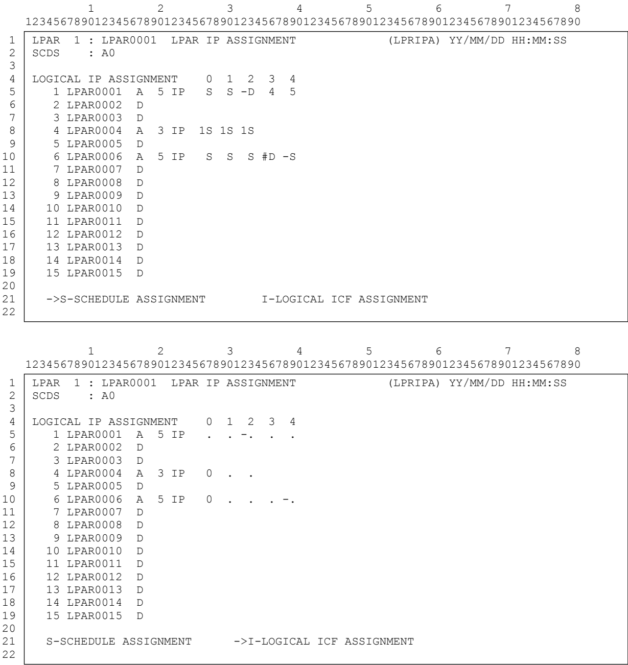
Figure 7-21 LPRIPA Frame on M3000 and C2000-xxC in MLPF 3.5.2, C2000-xxA and C2000-xxB
