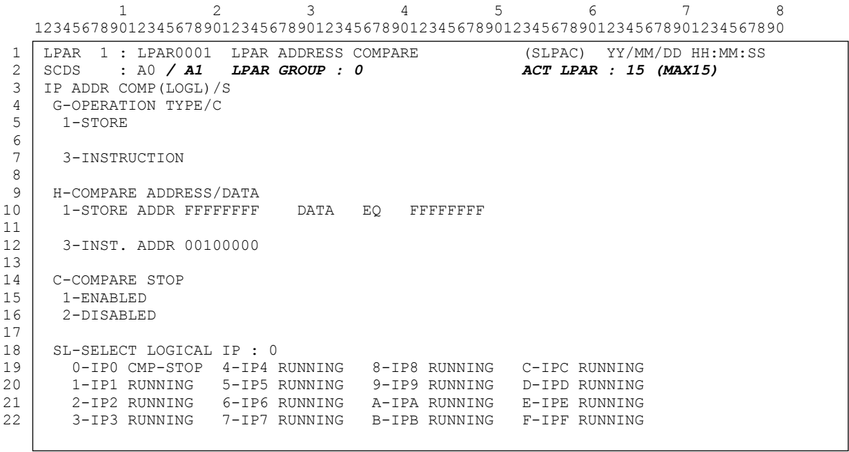
Figure 7-49 SLPAC Frame on M3000
