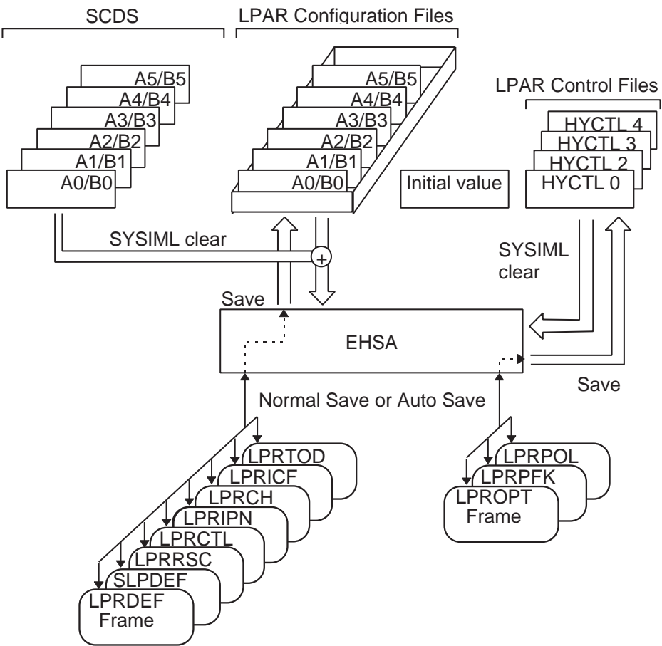
Figure 4-30 SYSIML Clear and Save without Updating SCDS
