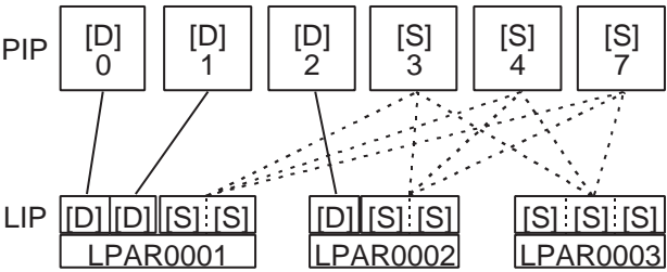
Figure 4-16 Combinations of PIPs and LIPs with PIPGSF Disabled
