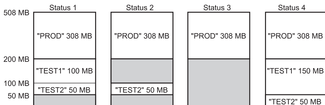
Figure 6-5 Example of Static Reconfiguration of MS
