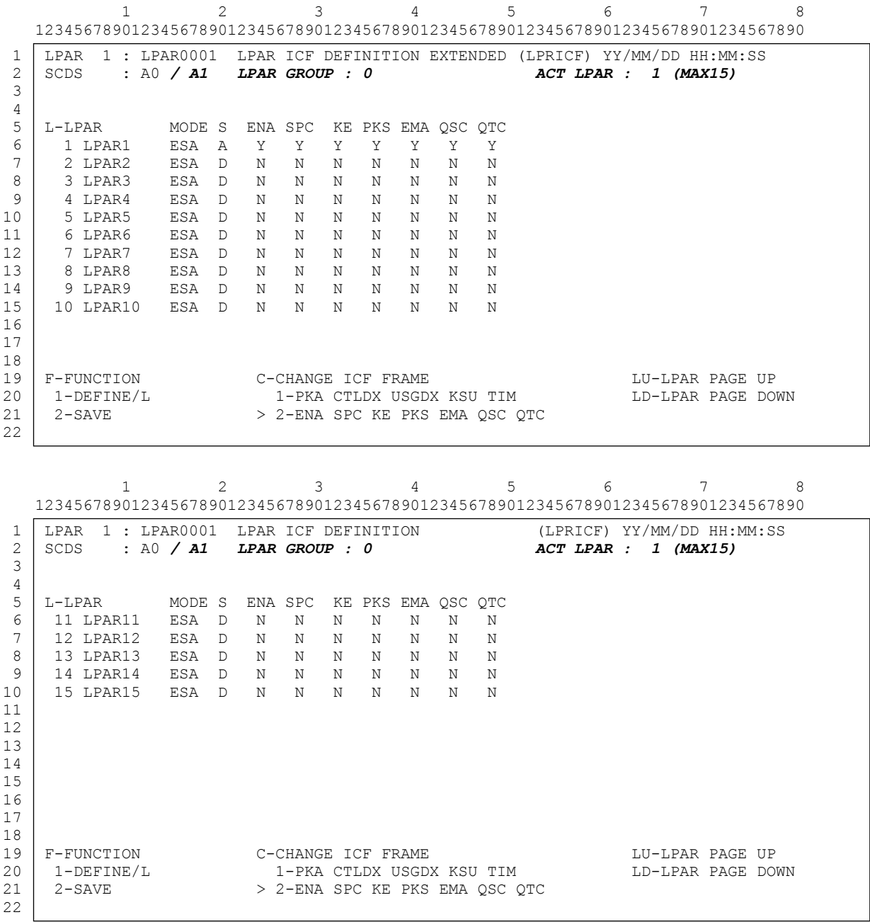
Figure 7-14 LPRICF Frame in MLPF 3.5.2—ENA to QTC
