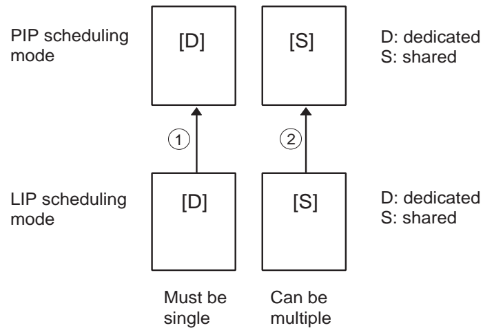
Figure 4-18 Restrictions in Assignment of Logical IPs to Physical IPs
