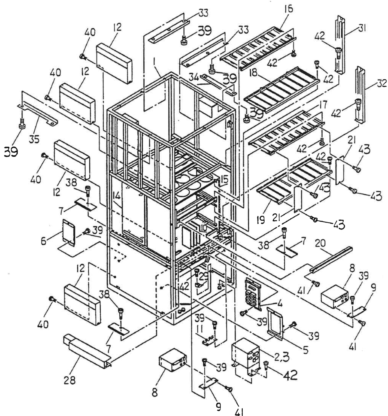
Fig. 2-4 SUB MAIN ASSY
