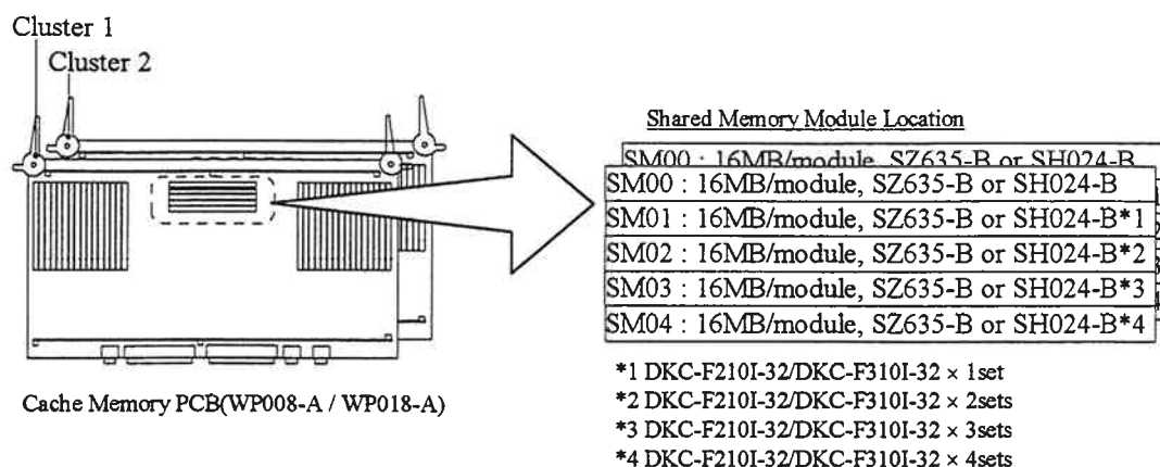
Fig. 3-2 Shared Memory Module Location
