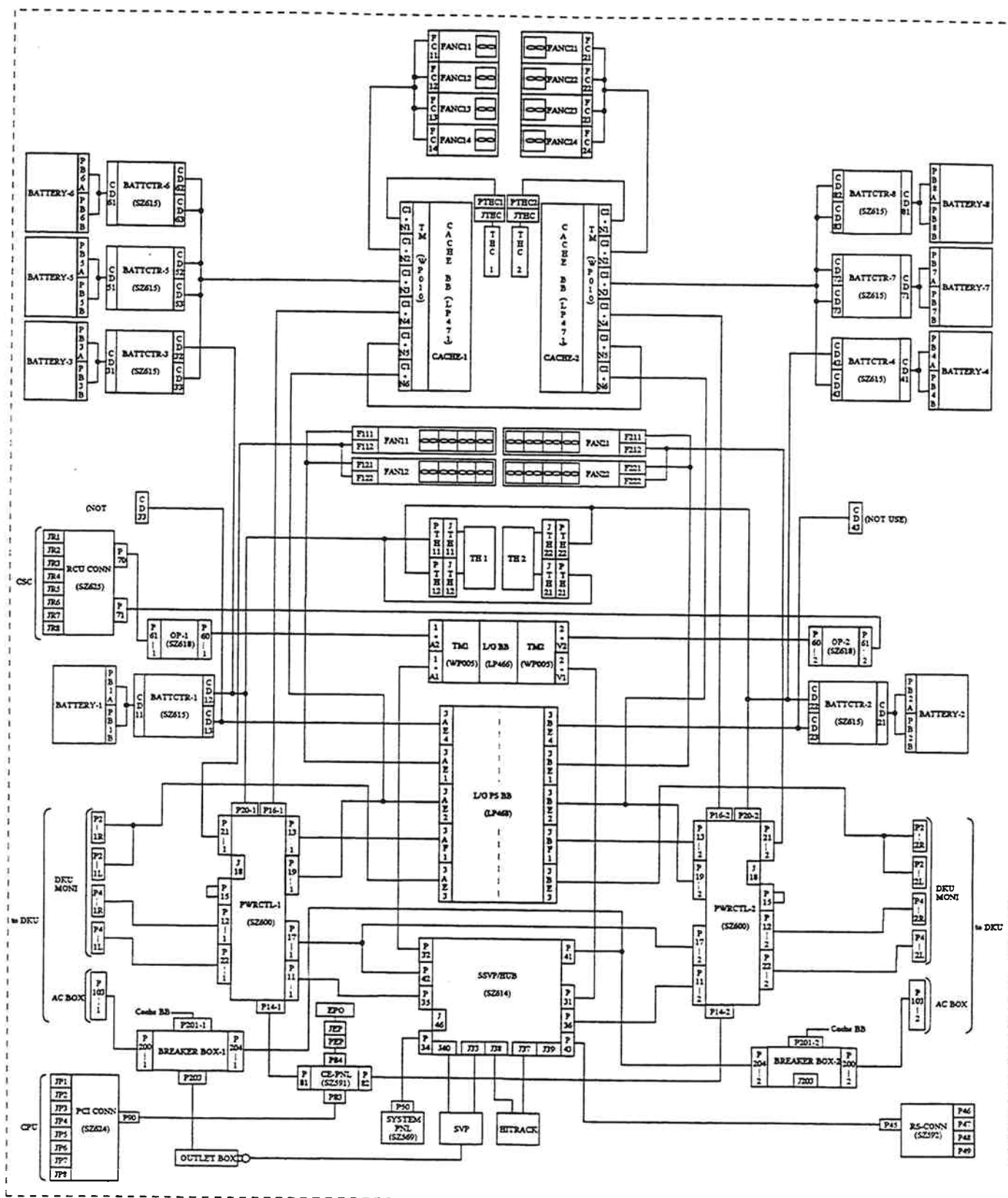
DKC210I and DKU205I Internal Cabling Diagram (1/7)
