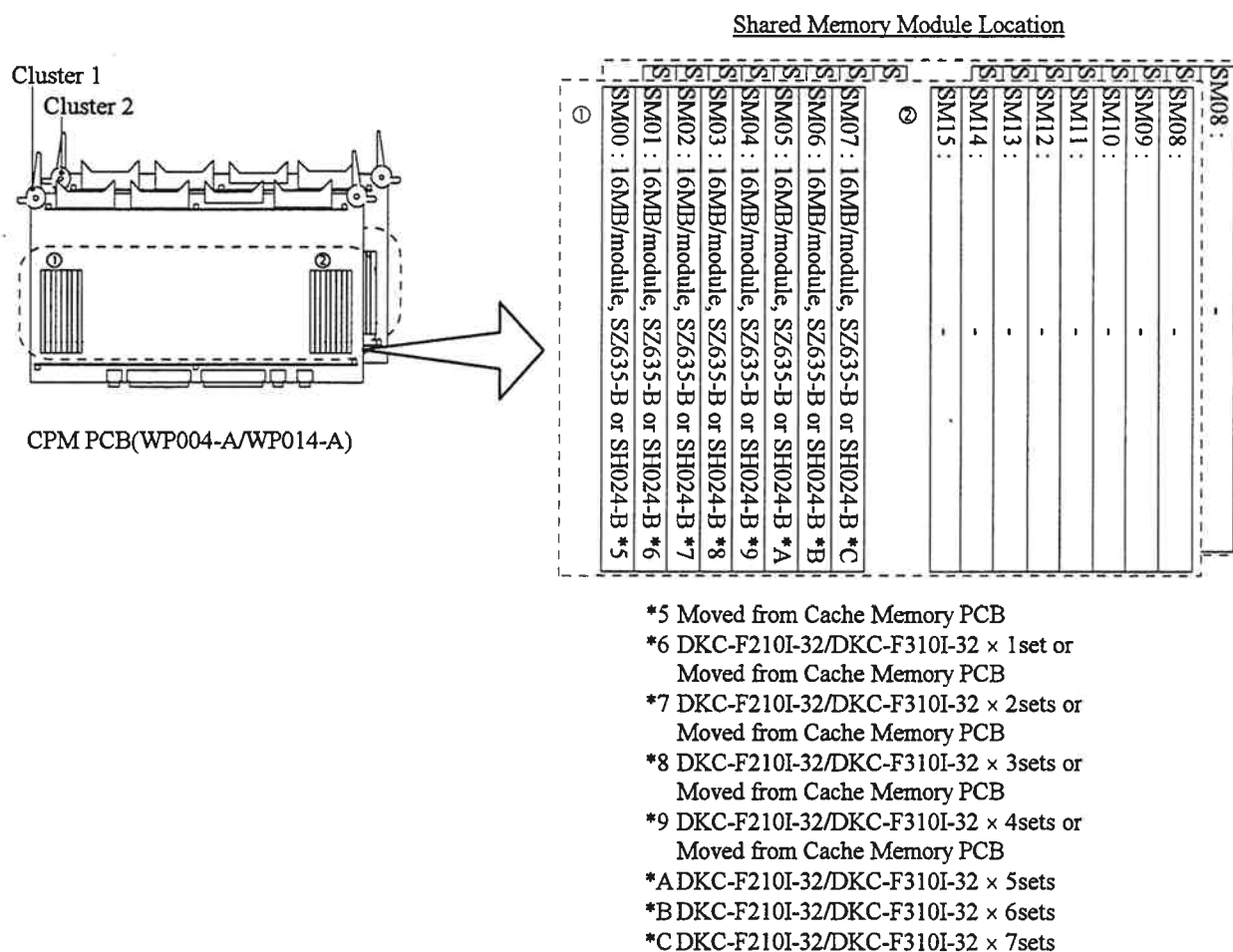
Fig. 3-3 Shared Memory Module Location
