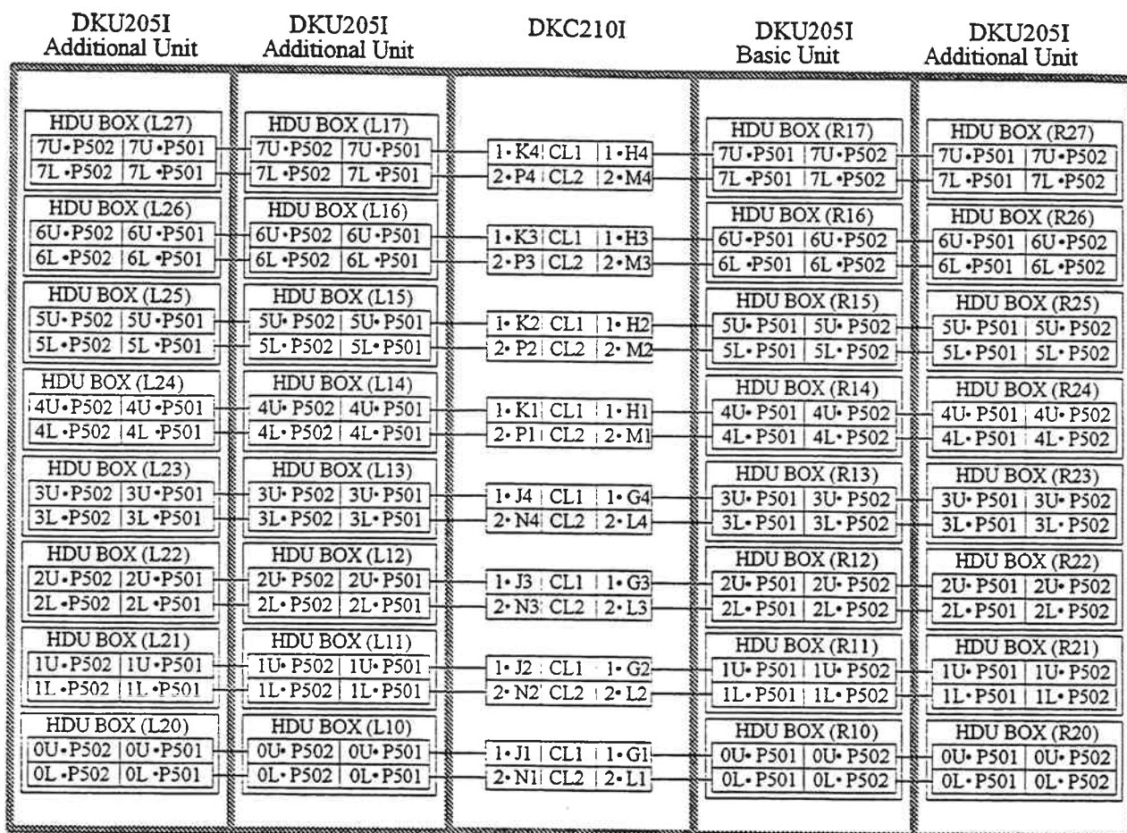
DKC210I and DKU205I Internal Cabling Diagram (6/7)
