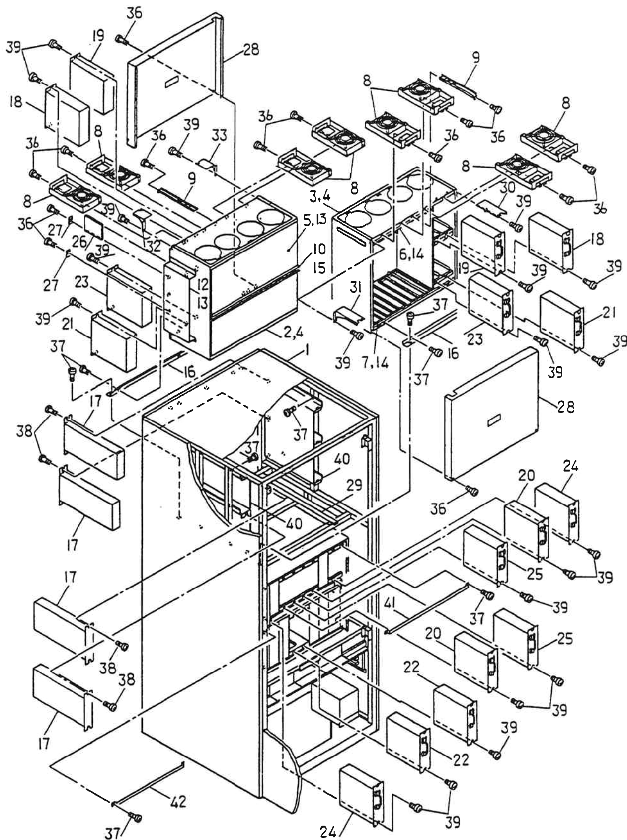
Fig. 2-5 CACHE BOX ASSY
