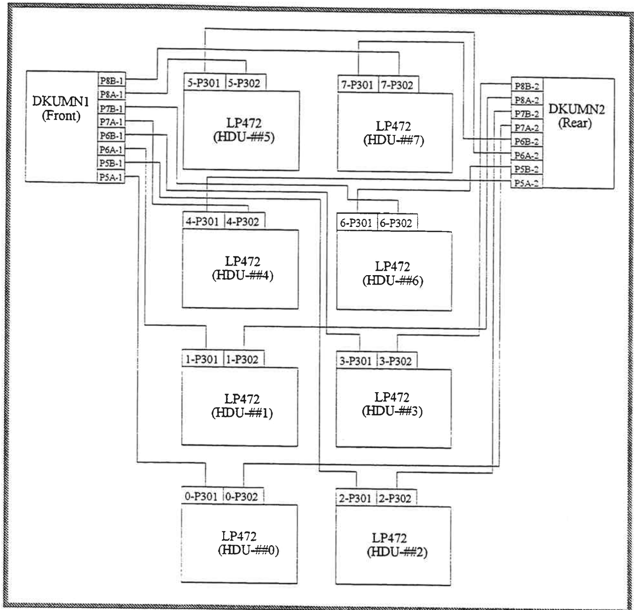
DKC210I and DKU205I Internal Cabling Diagram (3/7)
