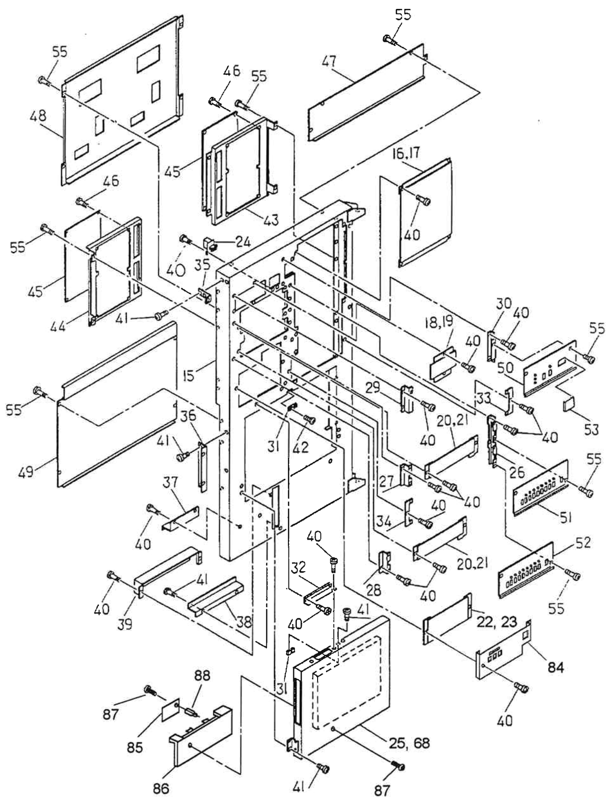
Fig. 2-3 MAIN ASSY (2/2)
