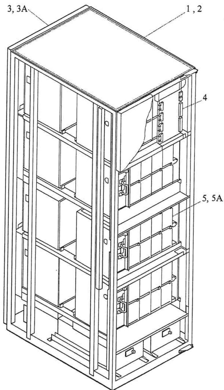
Fig. 1-1 DKU ASSY
