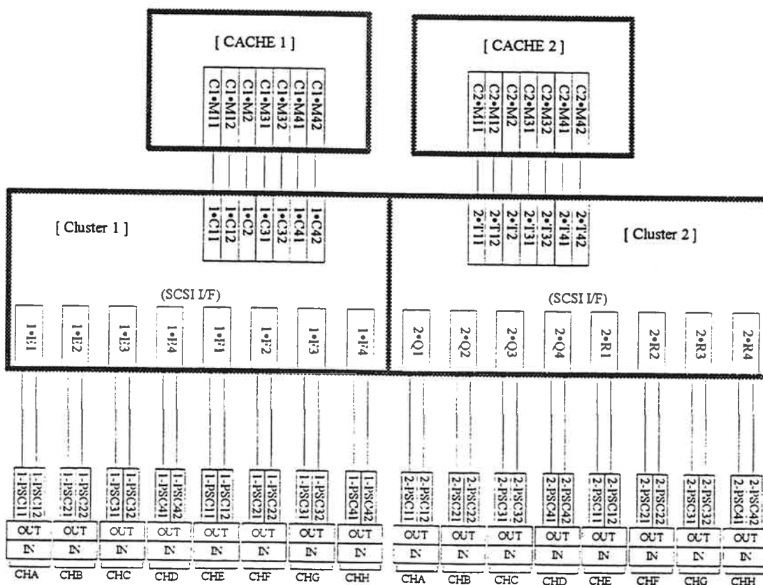
DKC210I and DKU205I Internal Cabling Diagram (2/7)
