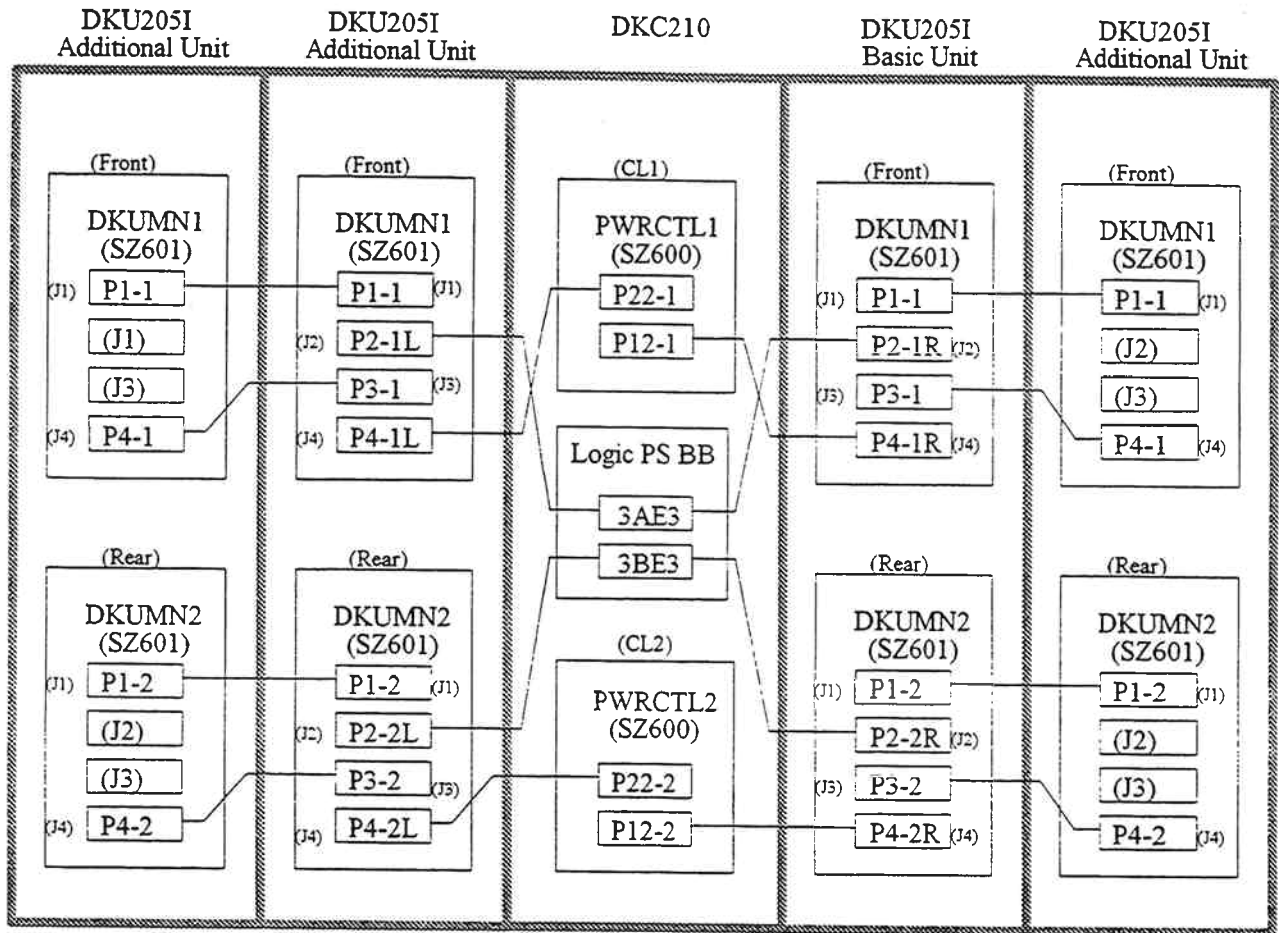
DKC210I and DKU205I Internal Cabling Diagram (7/7)
