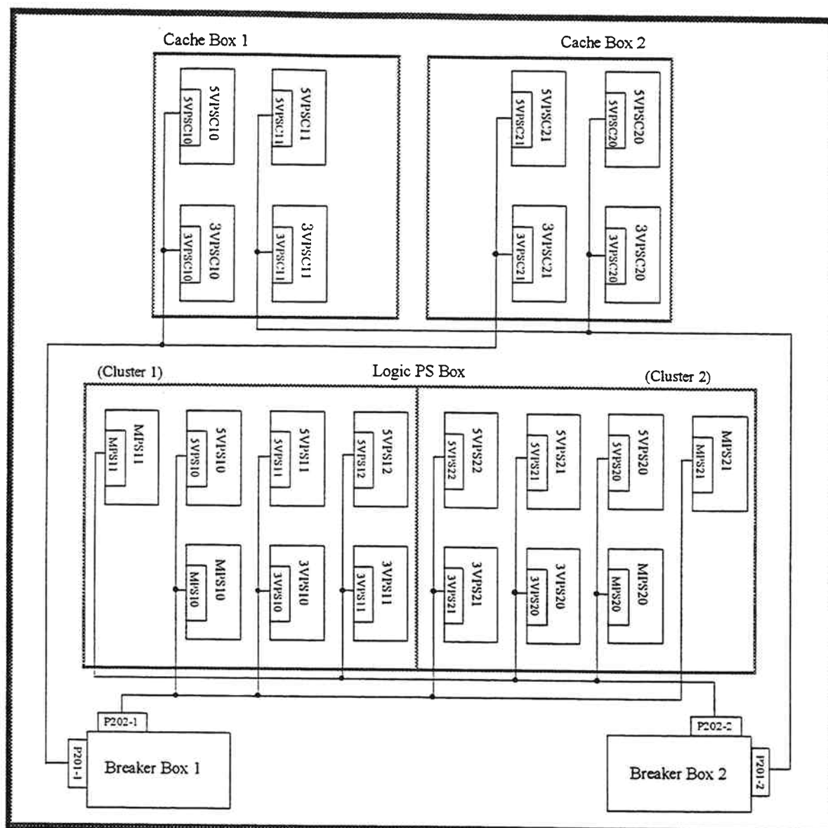
DKC210I and DKU205I Internal Cabling Diagram (4/7)
