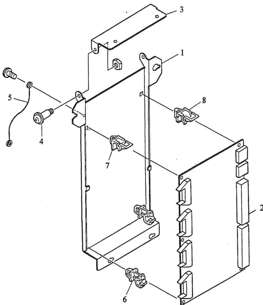
Fig. 1-5 DKU MONITOR ASSY
