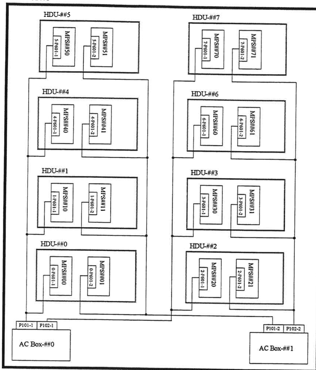
DKC210I and DKU205I Internal Cabling Diagram (5/7)
