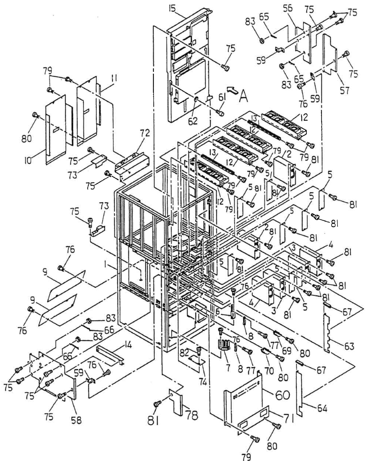
Fig. 2-2 MAIN ASSY (1/2)
