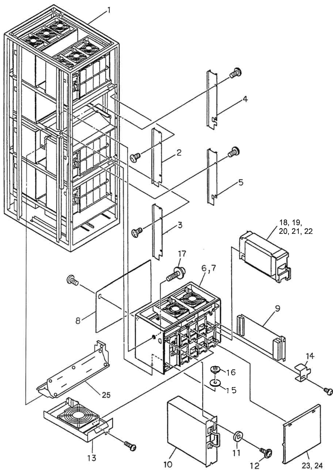
Fig. 1-3 DKU SUB ASSY
