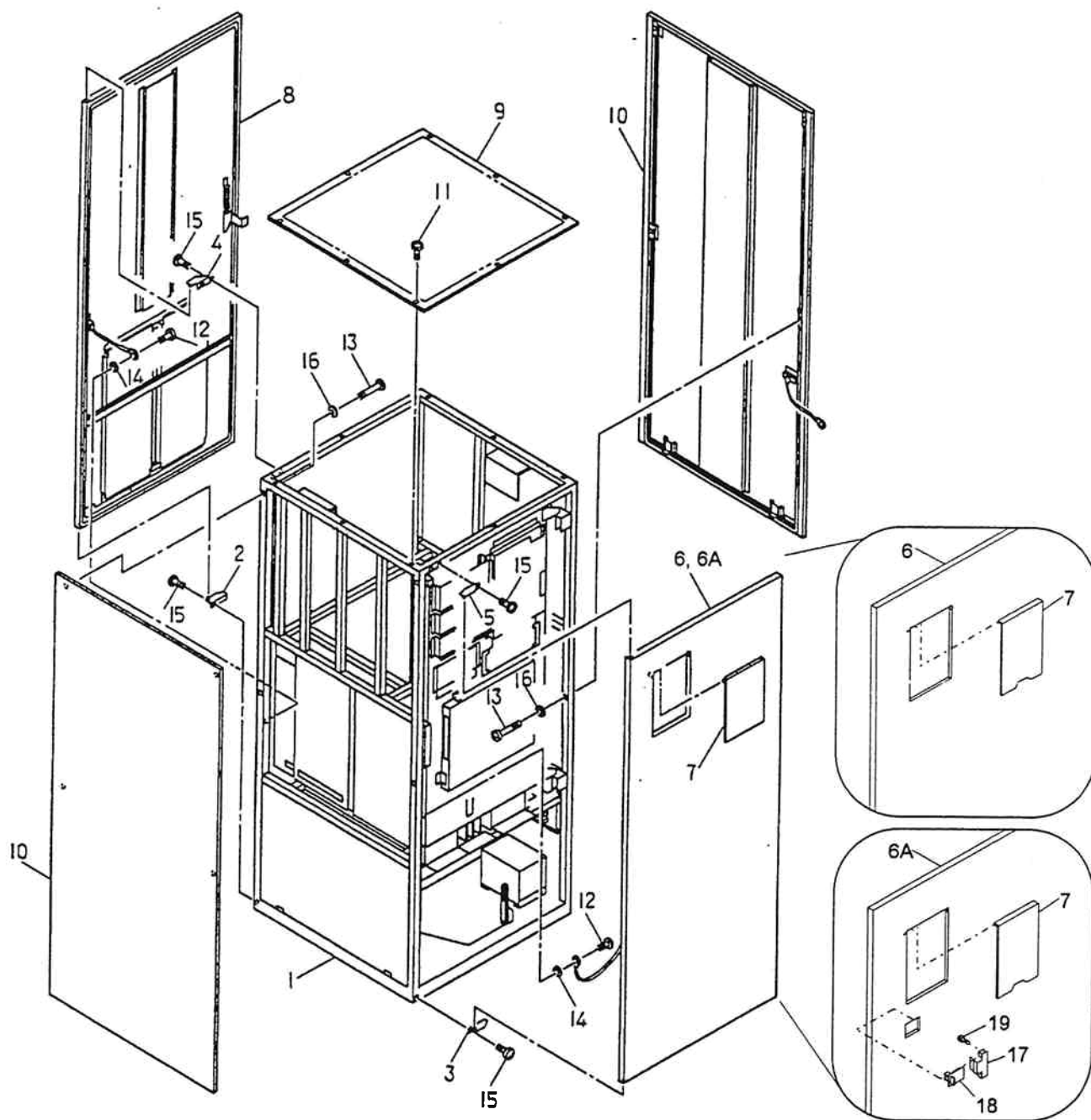
Fig. 2-1 DKC ASSY
