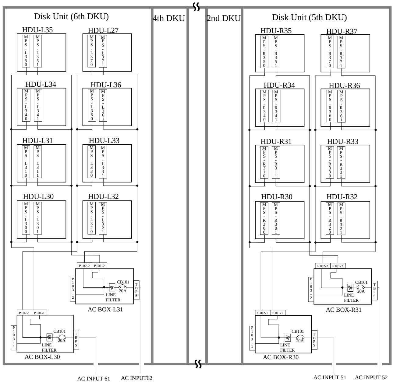
Fig. 3.3.2-5 Connection of POWER SUPPLIES (4/4)
