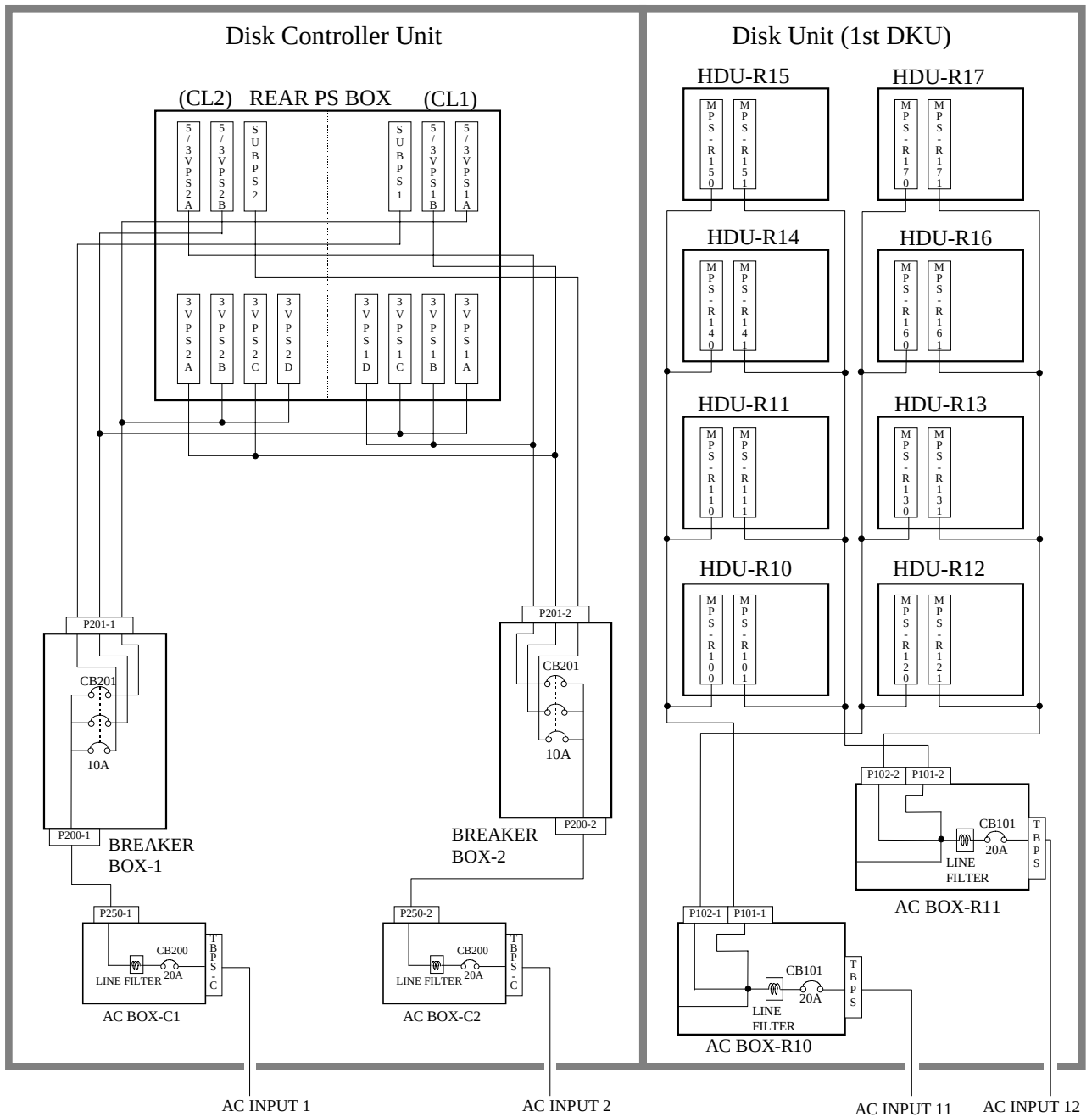
Fig. 3.3.2-2 Connection of POWER SUPPLIES (1/4)
