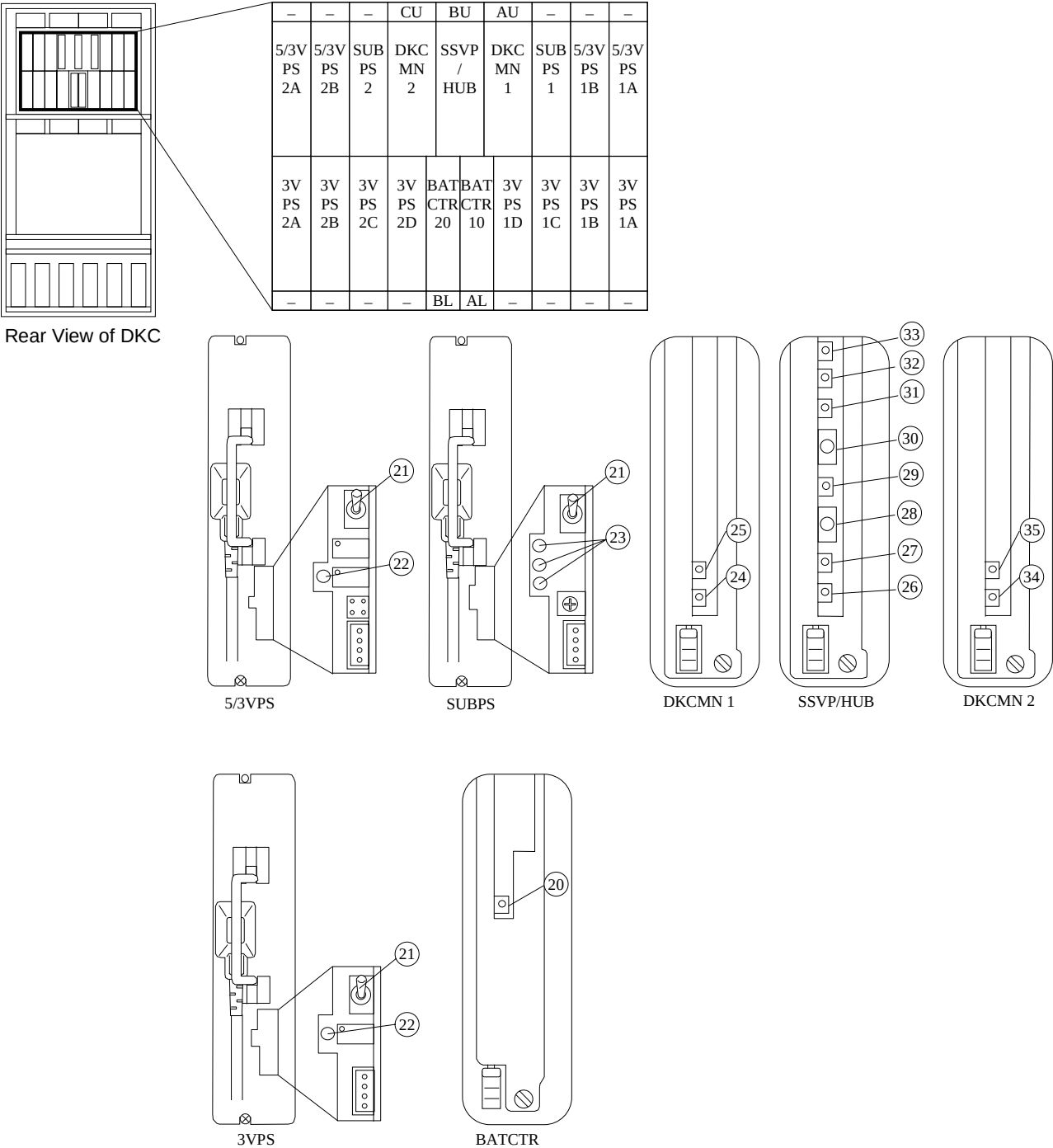
Fig 3.2-1 Other Switches and LEDs (2/3)
