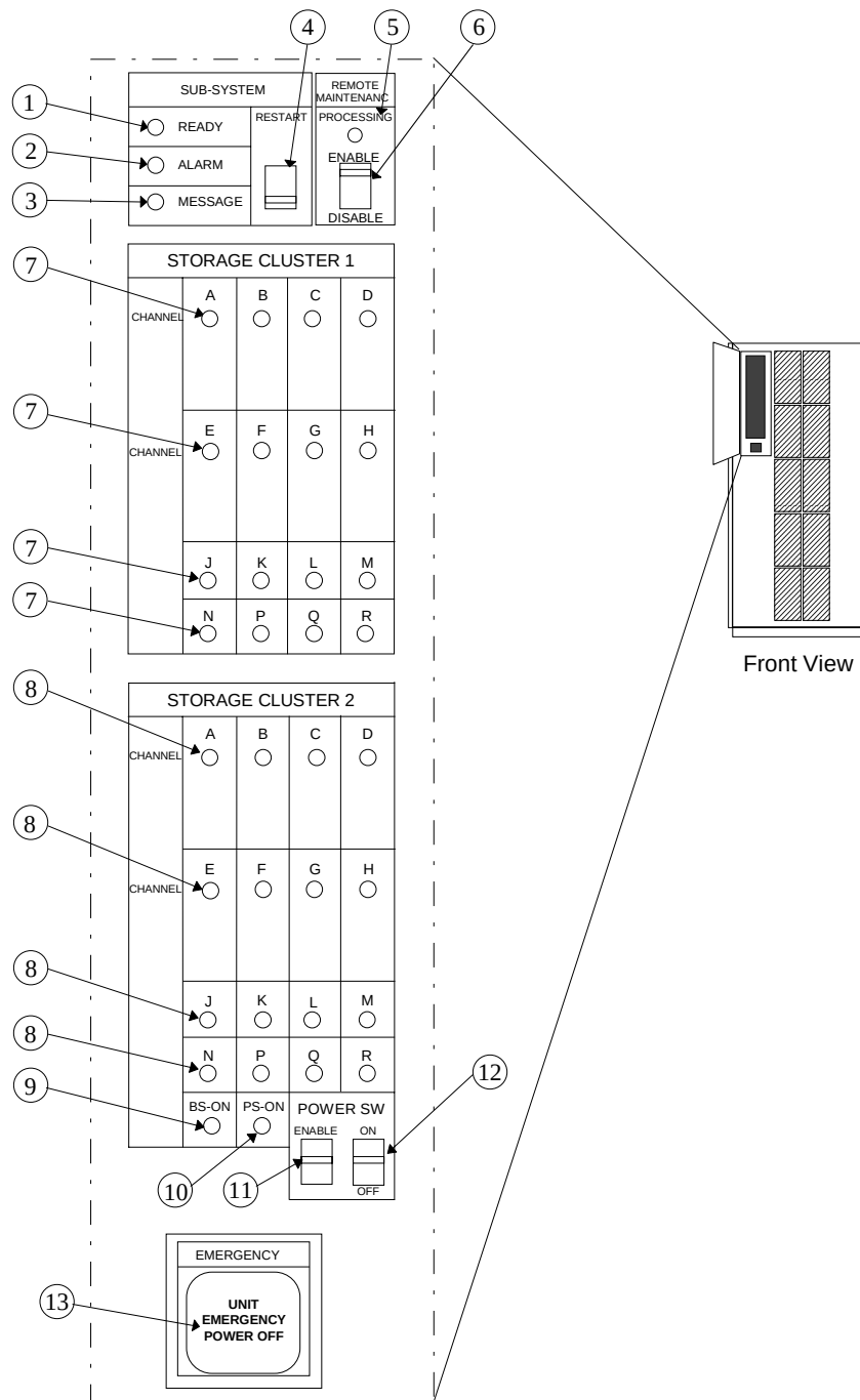
Fig. 3.1-1 Operator Panel
