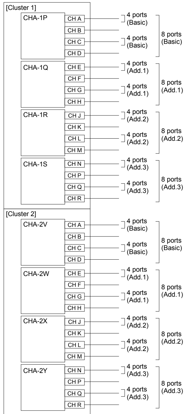
Fig. 5-5 Subsystem Internal Cabling Diagram ⑤
