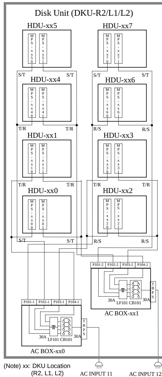
Fig. 3.3.3-3 Connection of POWER SUPPLIES (2/2)
