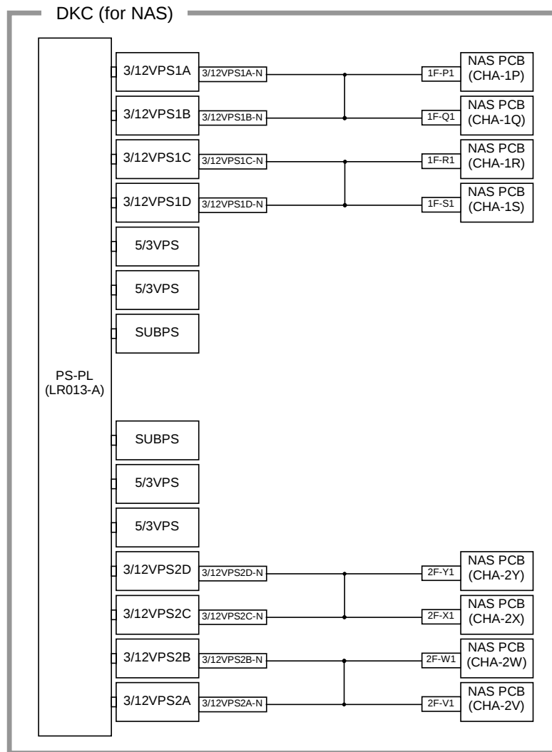
Fig. 5-1 Subsystem Internal Cabling Diagram ②
