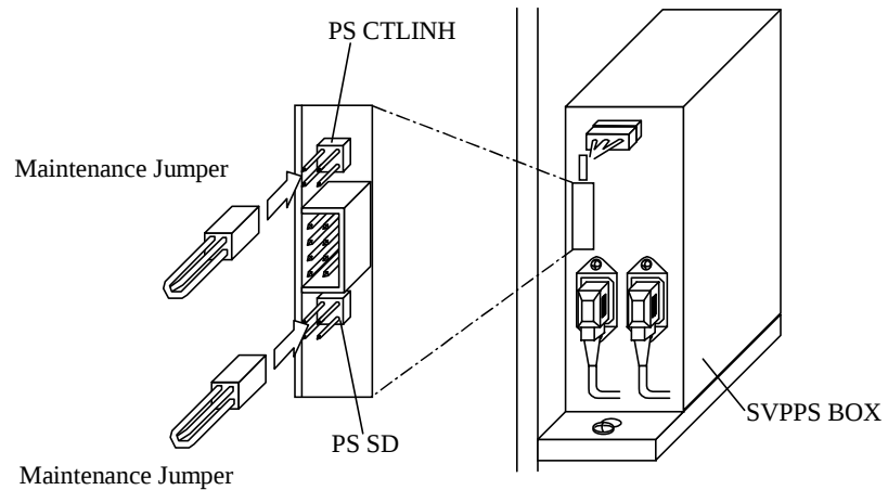
Front View of DKC
