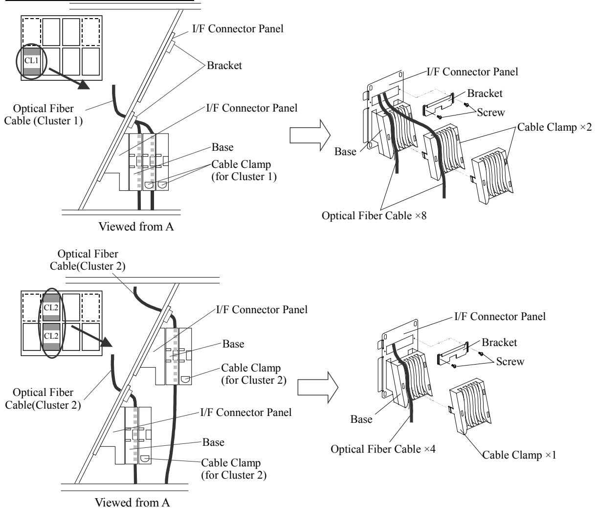
Fig. 4.2-1 The Mounting Location of Channel Options (2/7)
