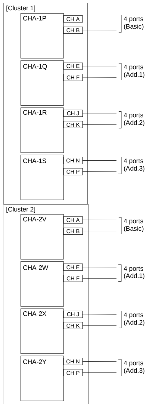
Fig. 5-4 Channel Interface Cabling Diagram ④
