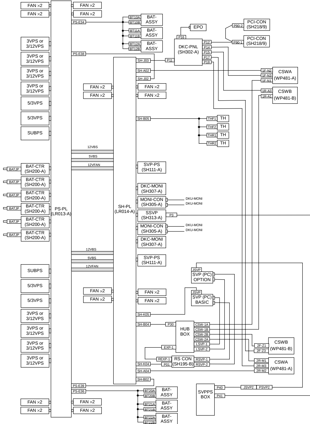
Fig. 5-1 DKC Internal Cabling Diagram ①
