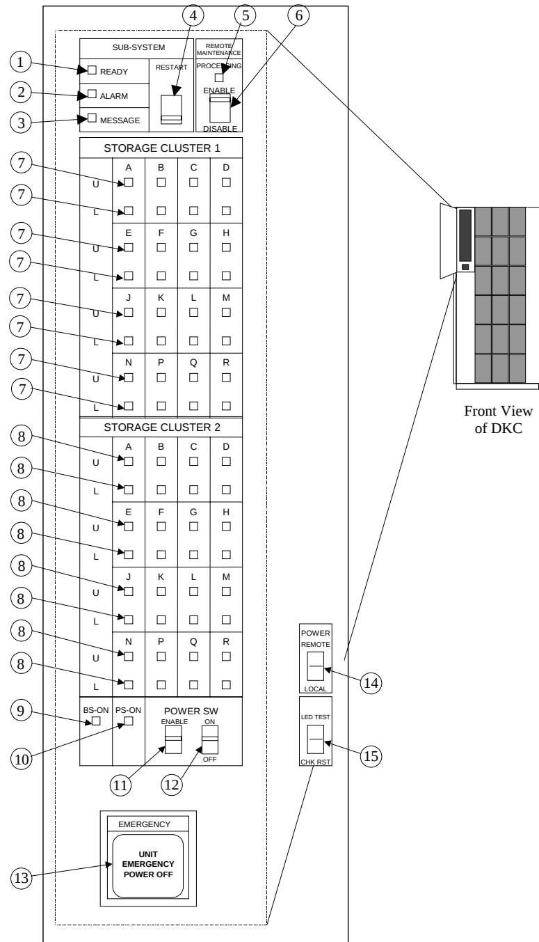
Fig. 3.1-1 Operator Panel
