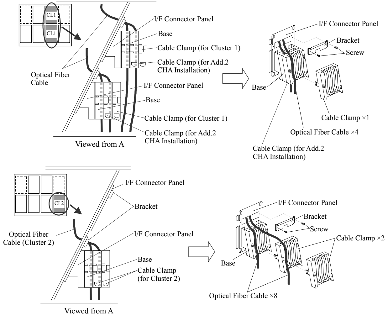
Fig. 4.2-1 The Mounting Location of Channel Options (4/7)
