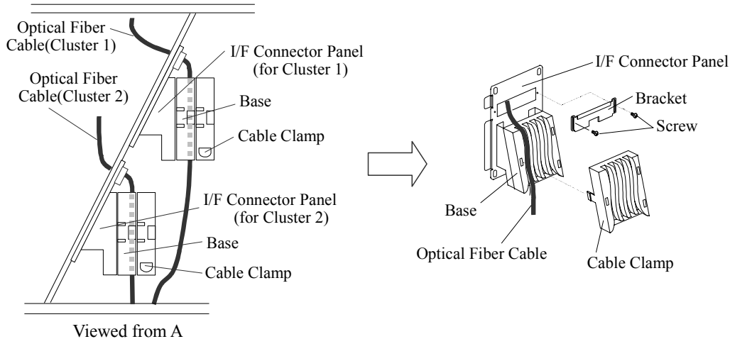
Fig. 4.2-1 The Mounting Location of Channel Options (1/7)
