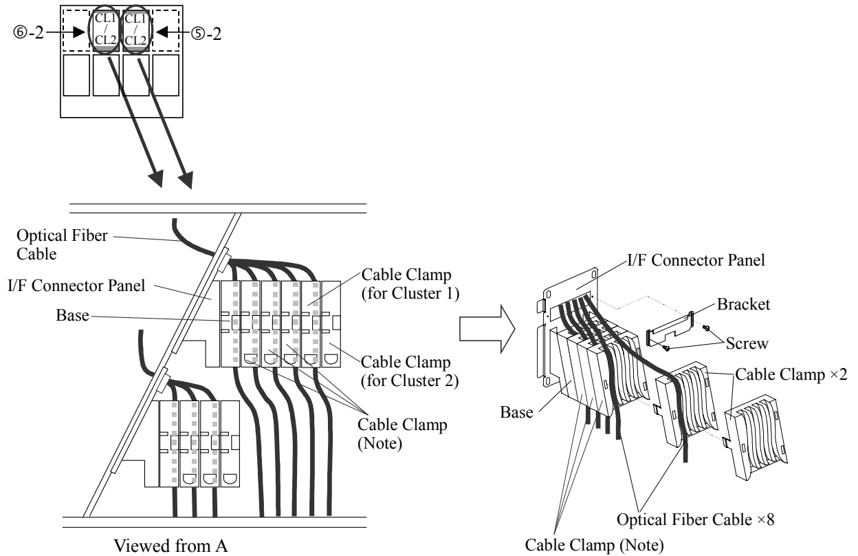
Fig. 4.2-1 The Mounting Location of Channel Options (7/7)
