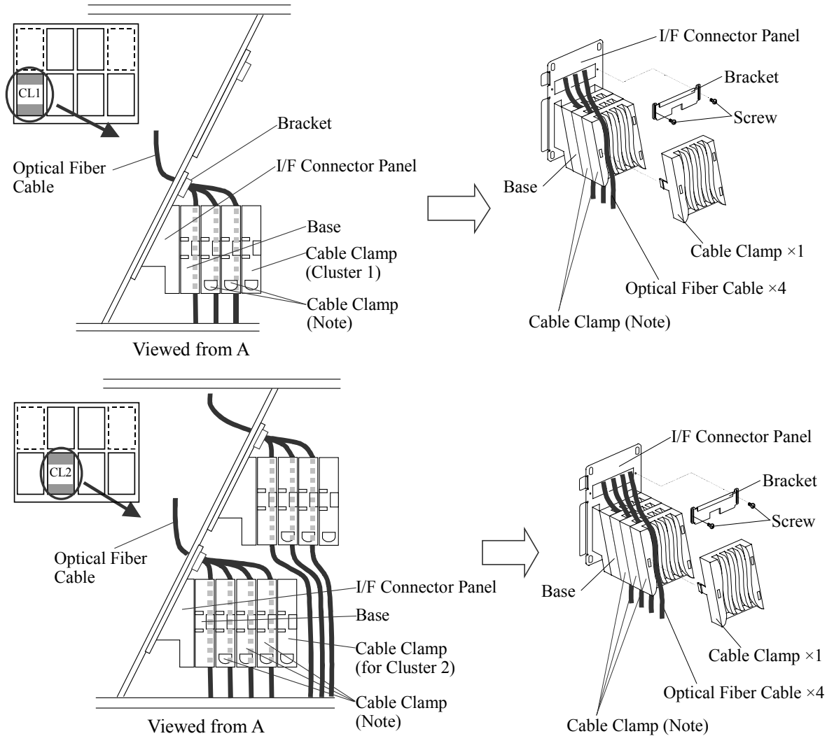
Fig. 4.2-1 The Mounting Location of Channel Options (6/7)
