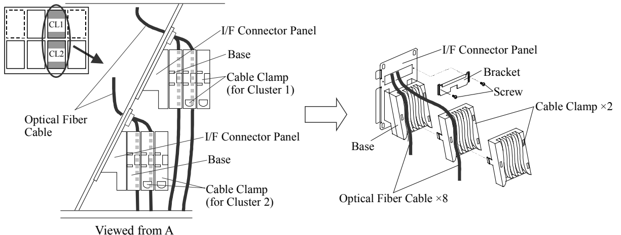
Fig. 4.2-1 The Mounting Location of Channel Options (3/7)
