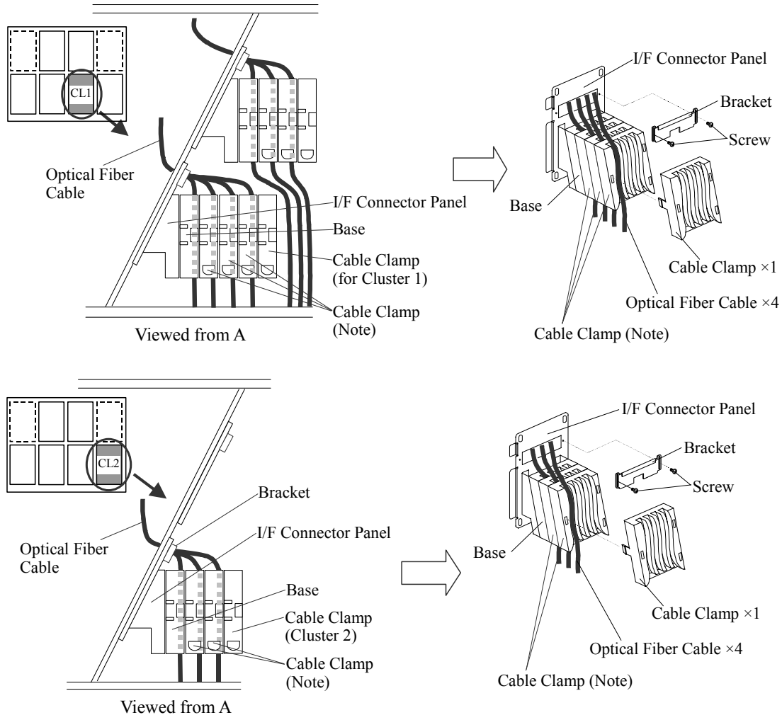
Fig. 4.2-1 The Mounting Location of Channel Options (5/7)
