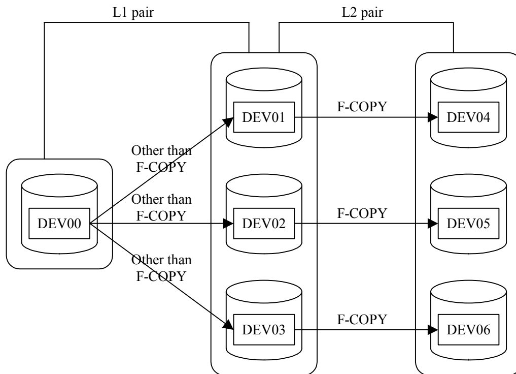
Fig. 3.14.9-1 HMRCF Extended Configuration Formed by Means of ShadowImage-FlashCopy® Option
