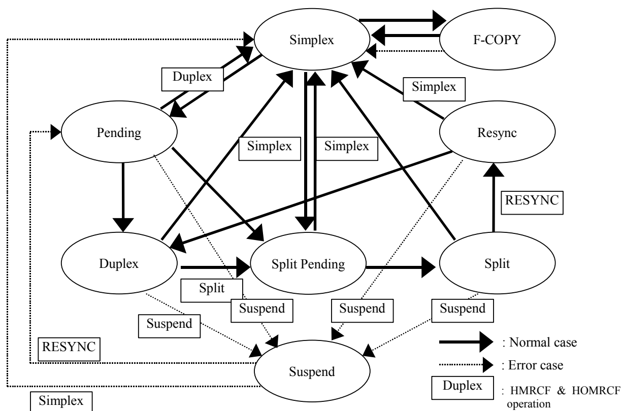
Fig. 3.14.5-1 Status transition map
