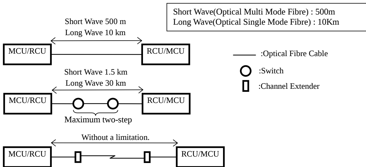
Fig. 3.13.3-2 Distance between Disk subsystems of Fibre channel interface connention
