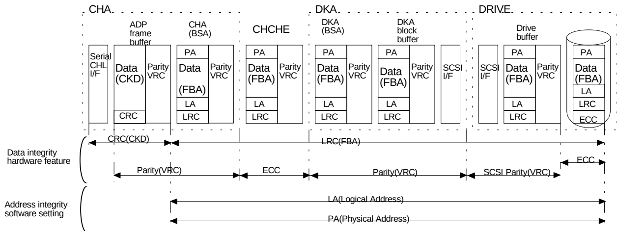
Fig. 3.3.3 Outline of Data Integrity
