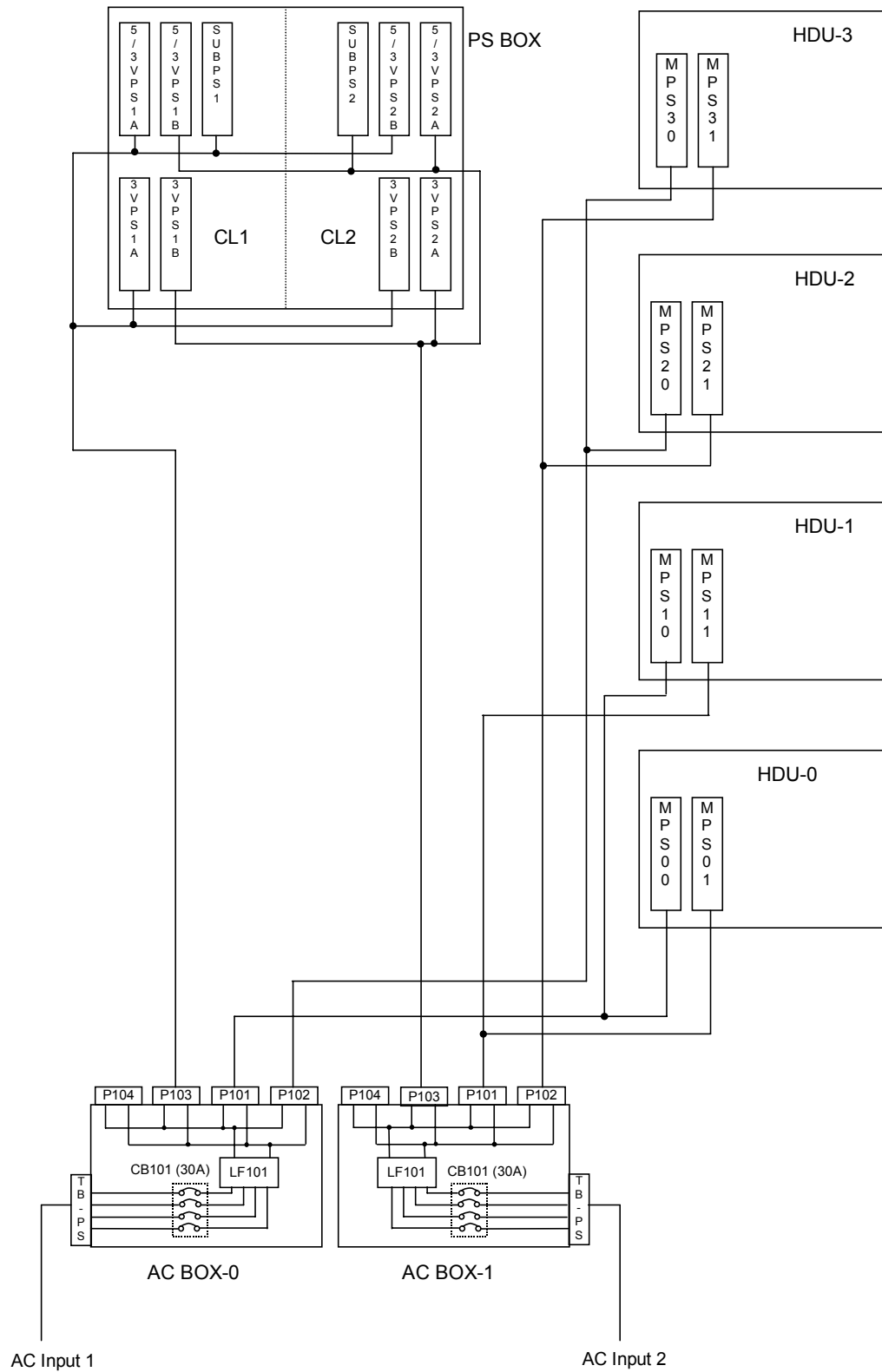
Fig. 3.3.1-2 Connection of POWER SUPPLIES
