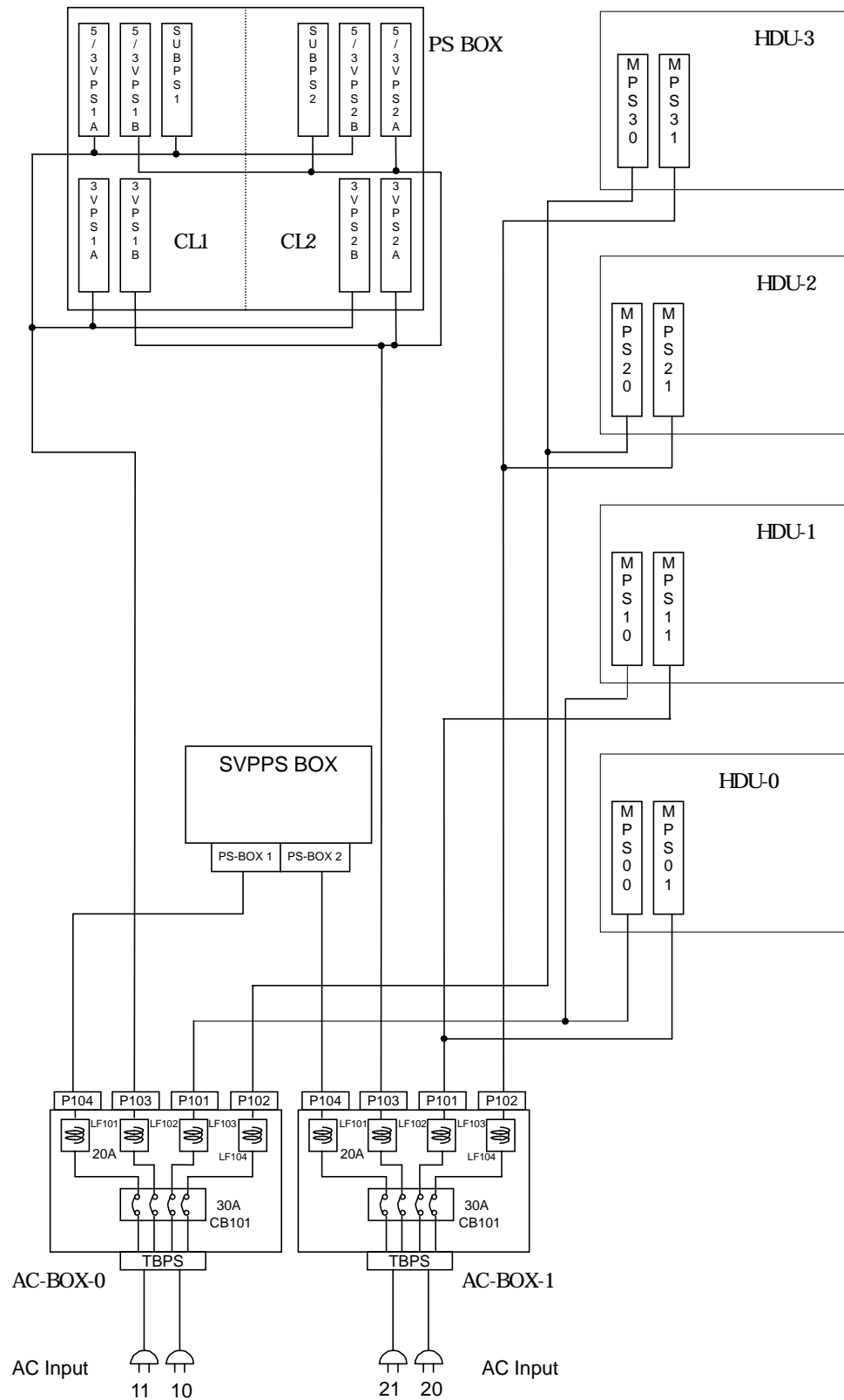
Fig. 3.3.1-2A Connection of Power Supplies for 30A
