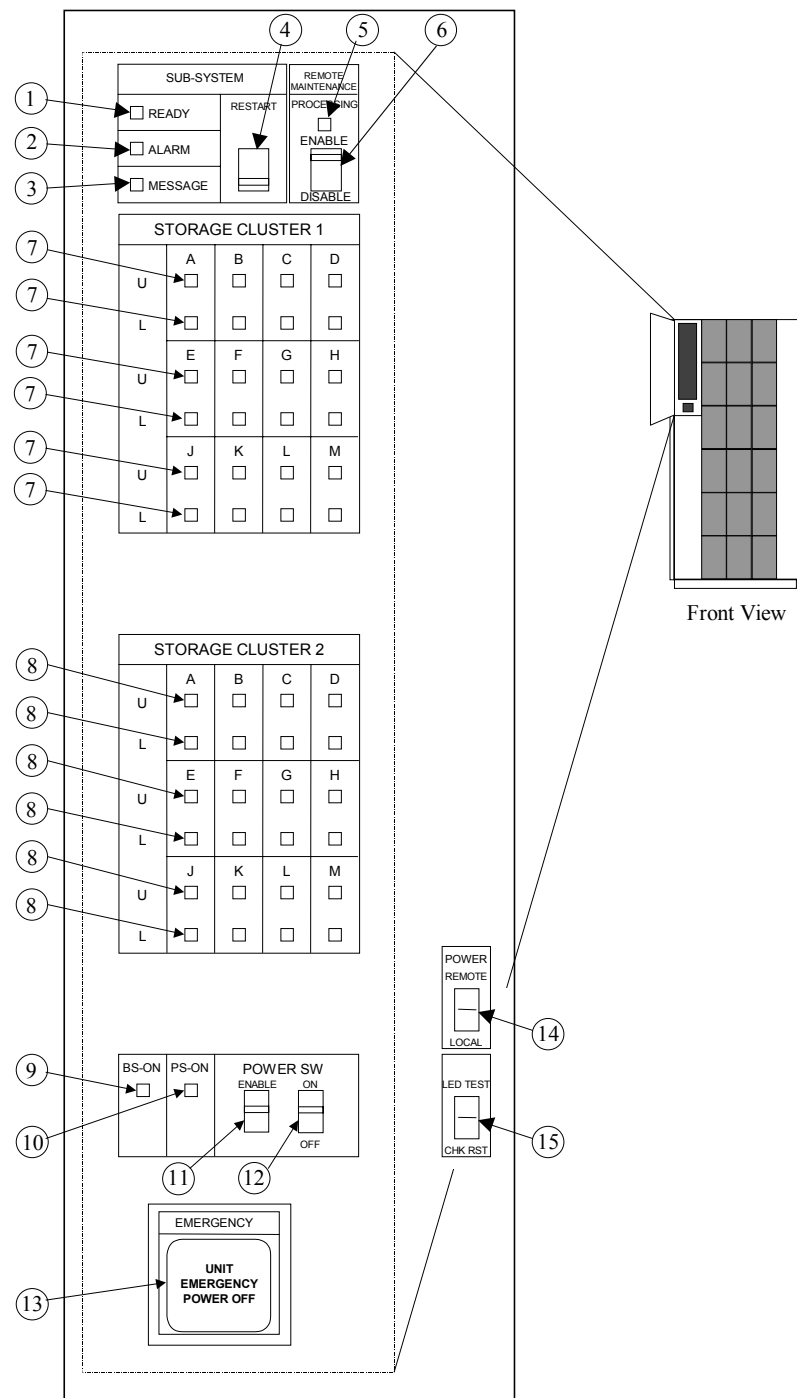
Fig. 3.1-1 Operator Panel
