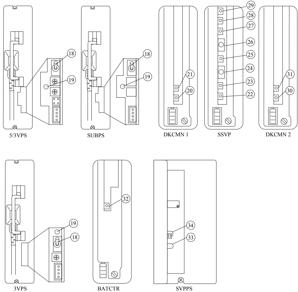
Fig 3.2-2 Other Switches and LEDs (2/3)
