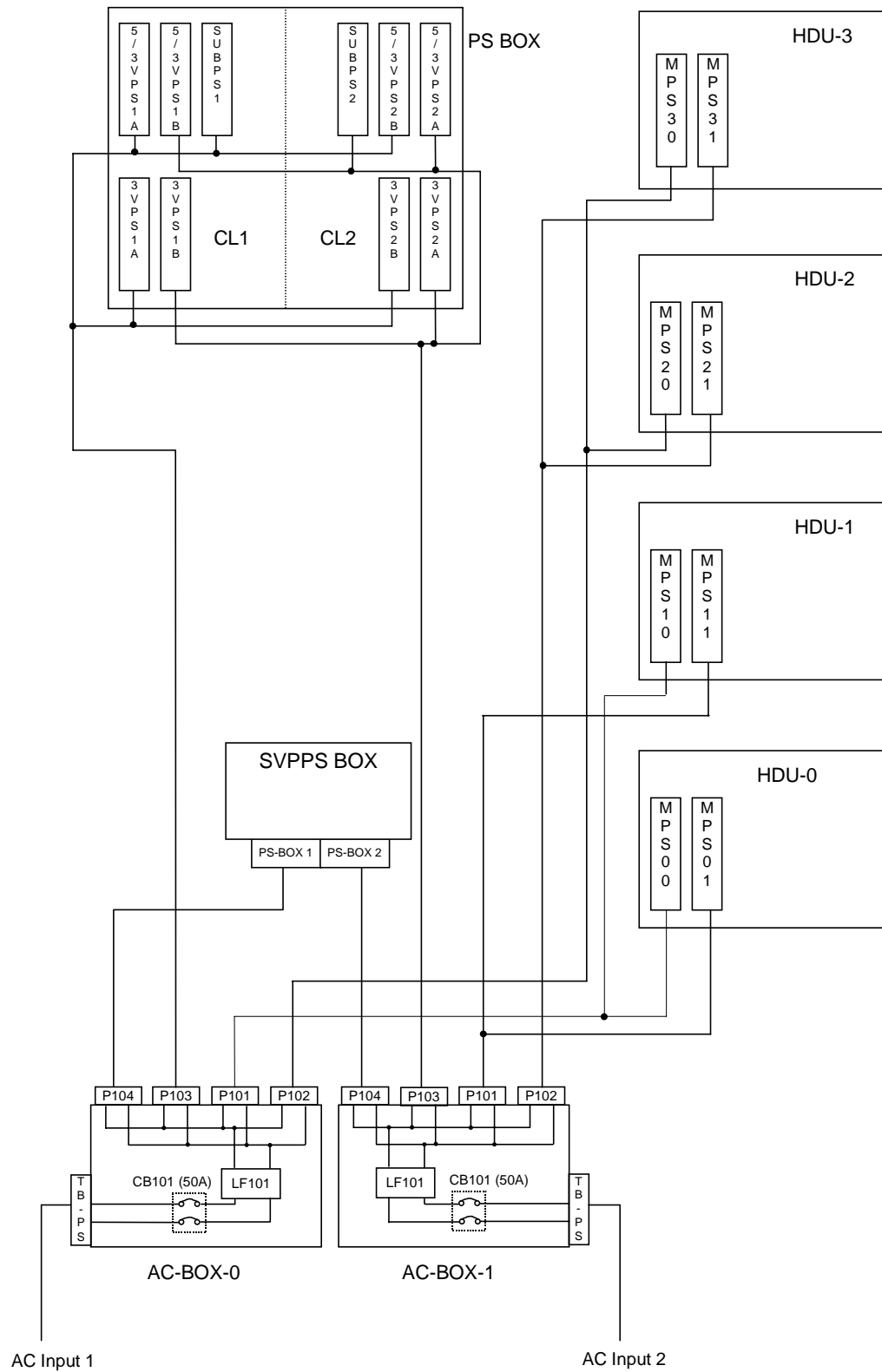
Fig. 3.3.1-2 Connection of Power Supplies for 50A
