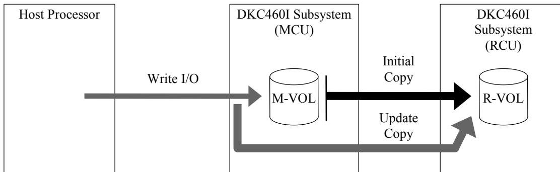
Fig. 3.11.4-1 HRC Copy Activities
