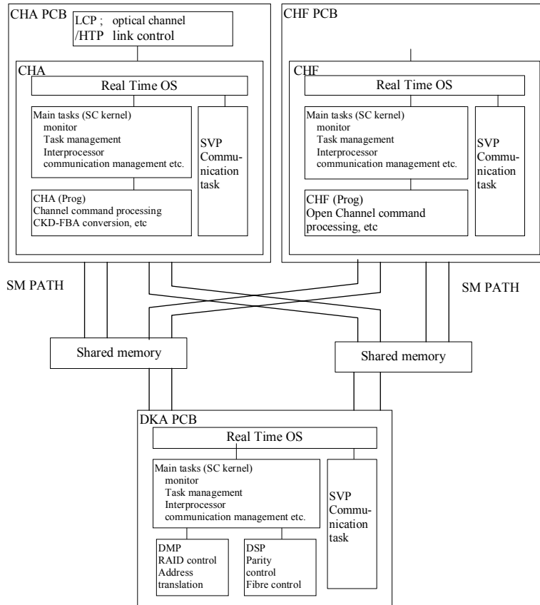
Fig. 3.2-1 Software Organization
