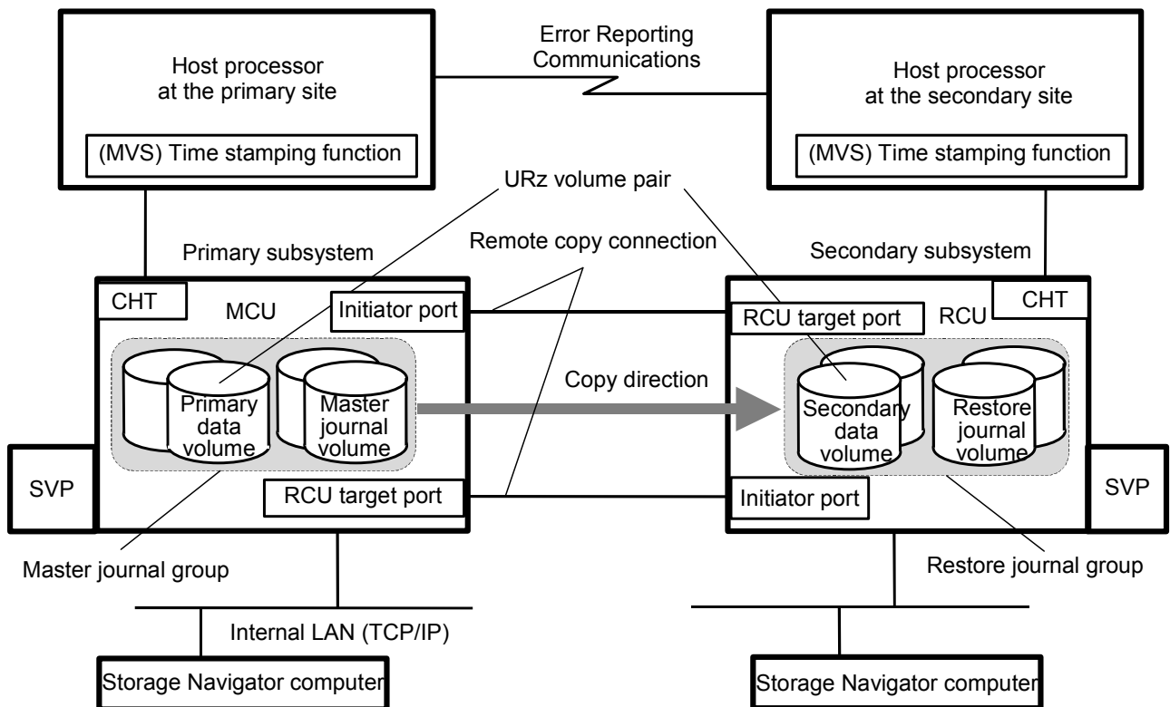
Figure 3.22-1 URz components
