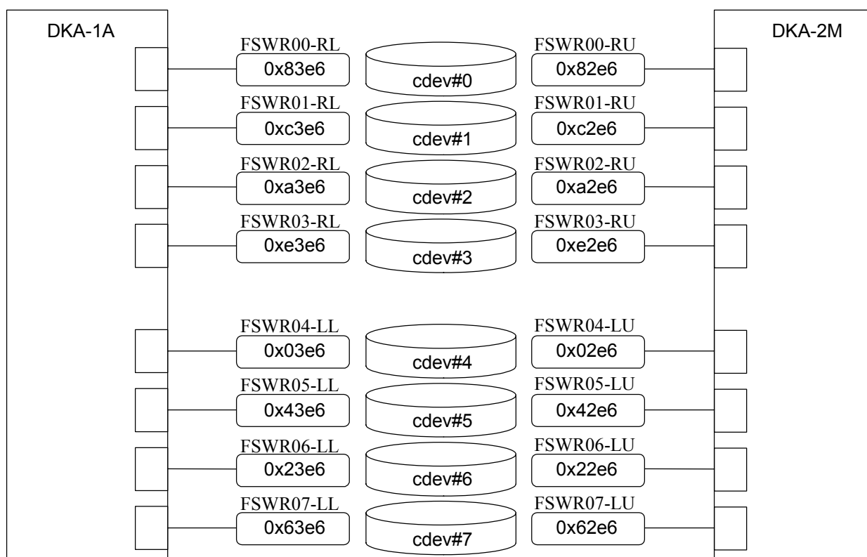
Fig. 6.2-1 DKA Path Address mapping (R0 Unit)
