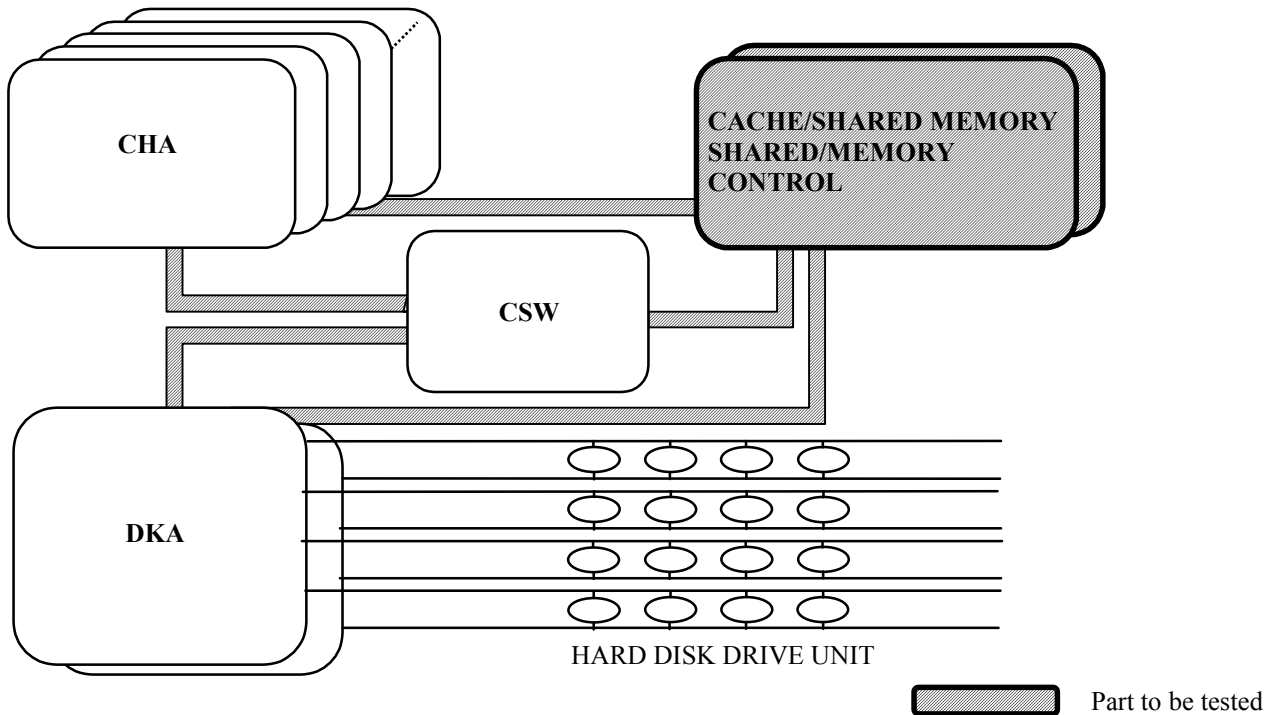
Fig. 3-2 Parts Subject to INLINE CUDG Tests
