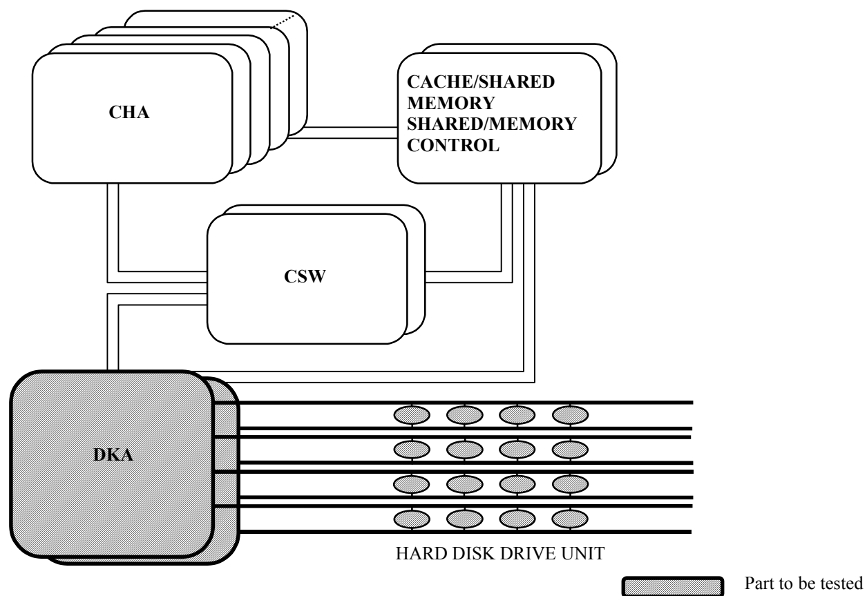
Fig. 3-3 Parts Subject to DKU INLINE Tests
