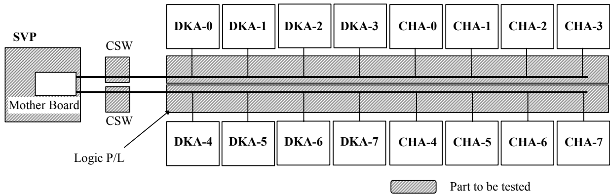
Fig. 3-5 Parts Subjects to LAN check
