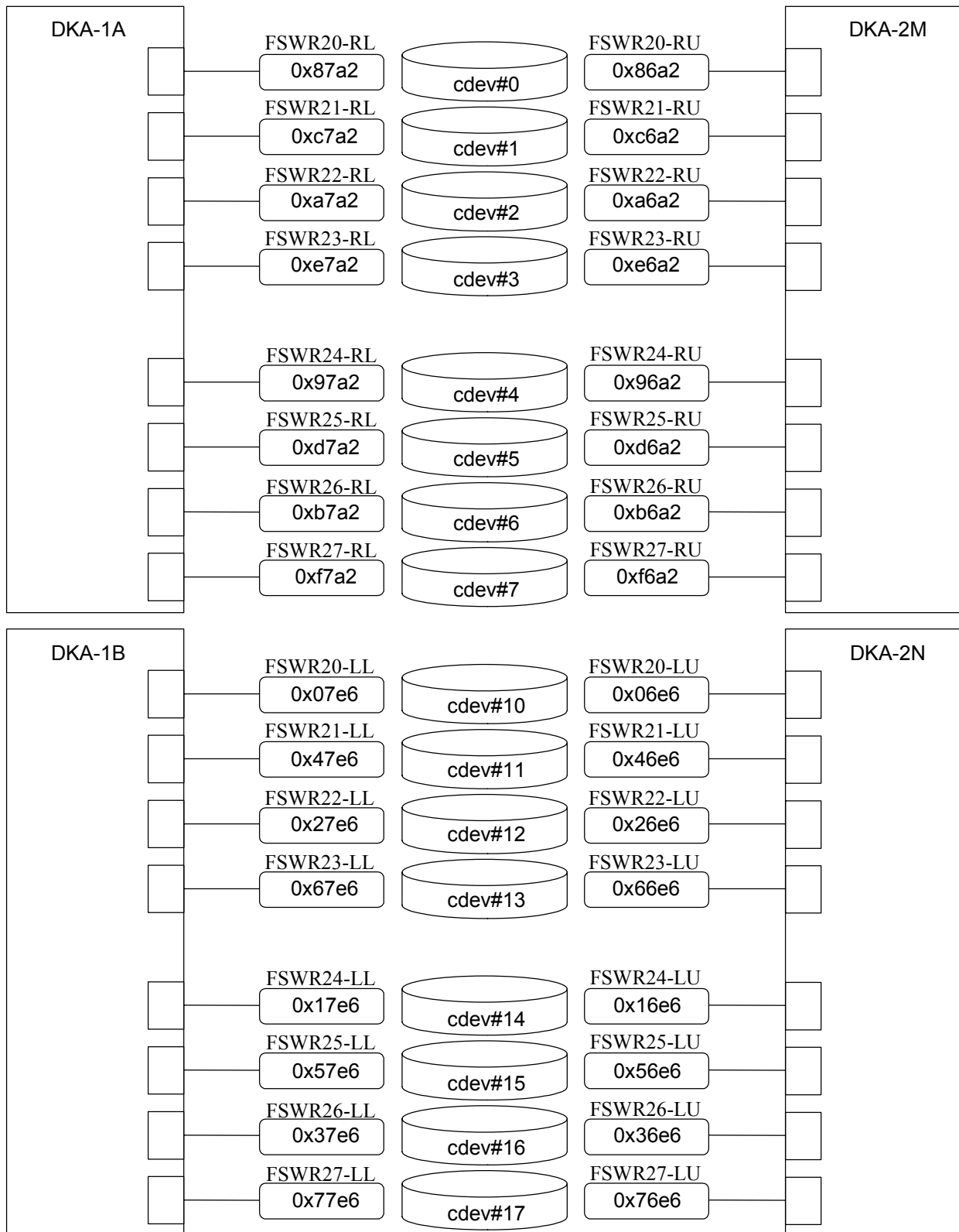
Fig. 6.2-3 DKA Path Address mapping (Hi-Performance Model : R2 Unit)
