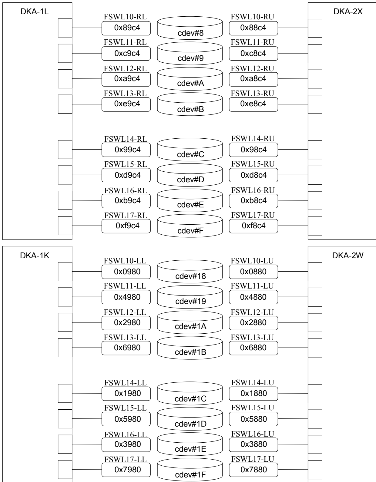
Fig. 6.2-4 DKA Path Address mapping (Hi-Performance Model : L1 Unit)
