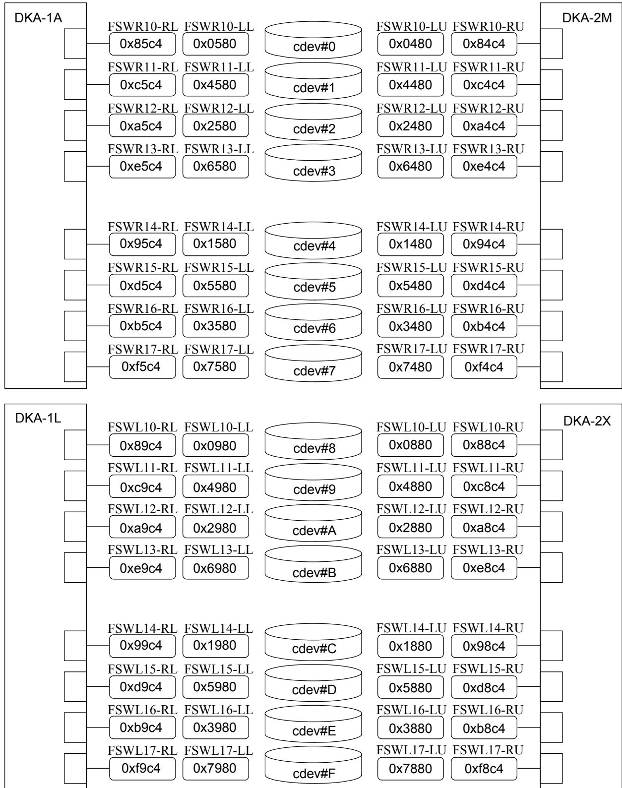
Fig. 6.2-6 DKA Path Address mapping (Standard Model : R1,L1 Unit)
