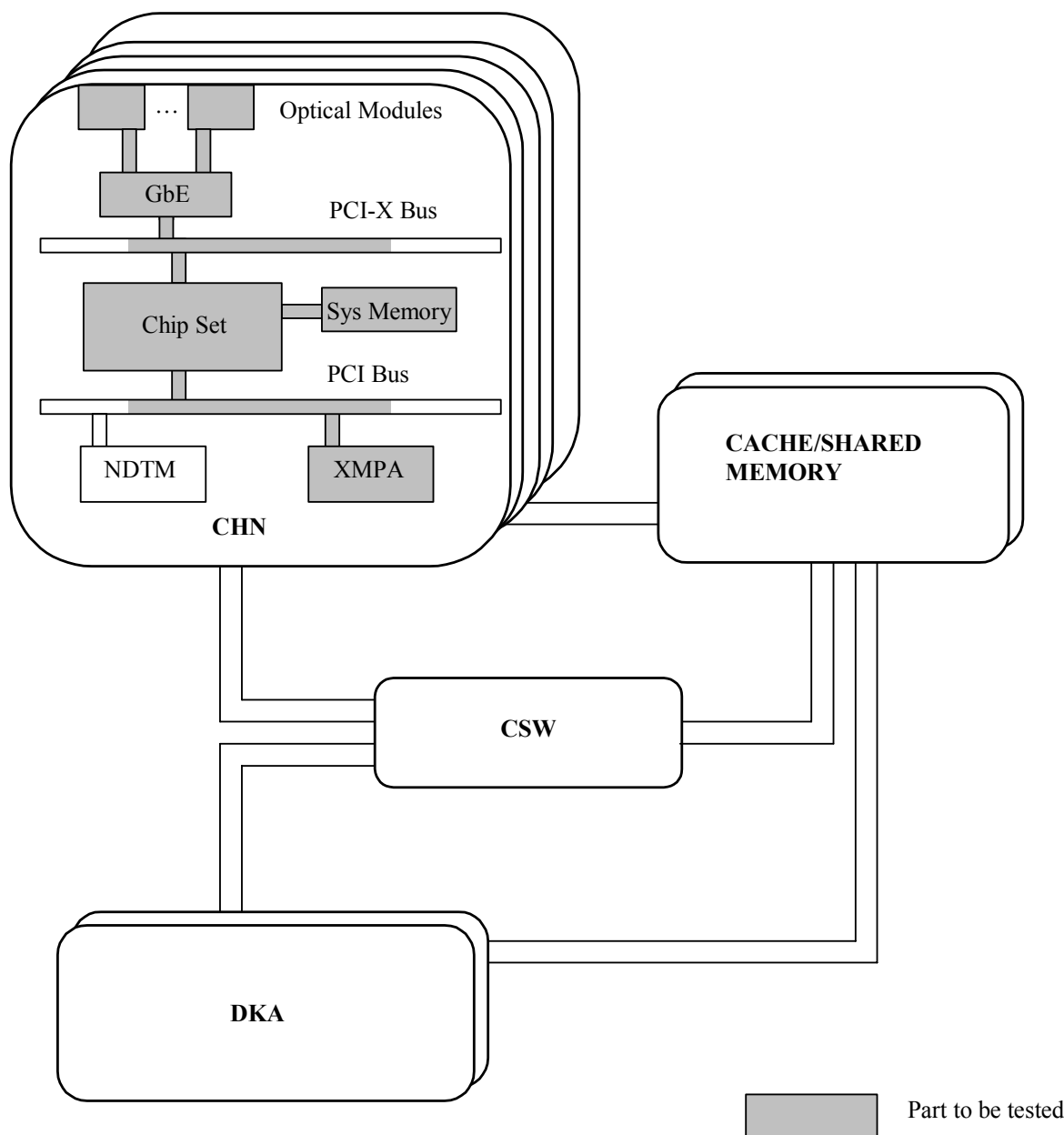
Fig. 3-8 Parts Subject to PCDG4 Tests
