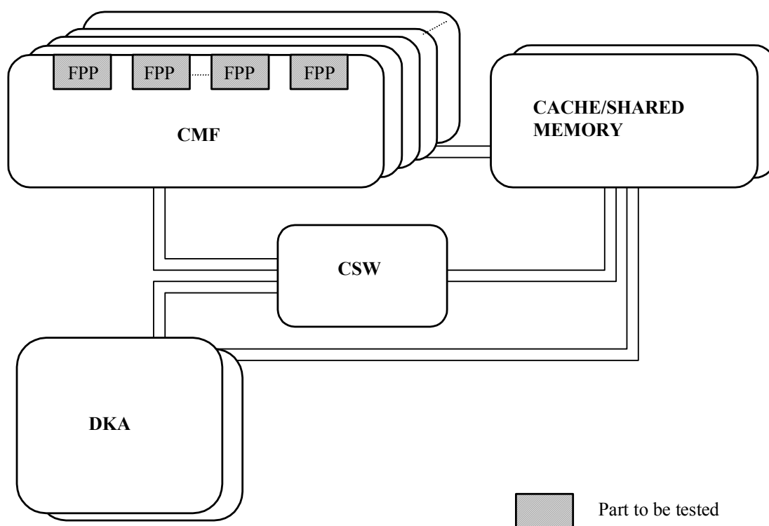
Fig. 3-7 Parts Subject to FCDG4 Tests
