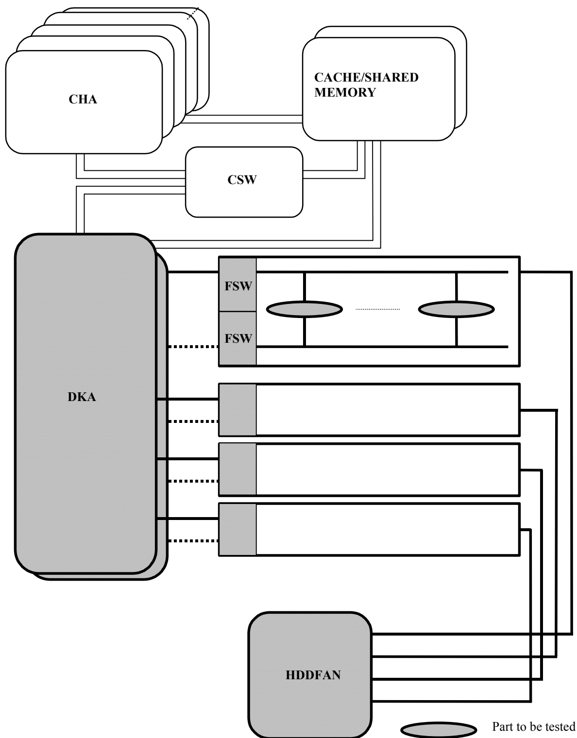
Fig. 3-4 Parts Subject to DKU PATH INLINE Tests
