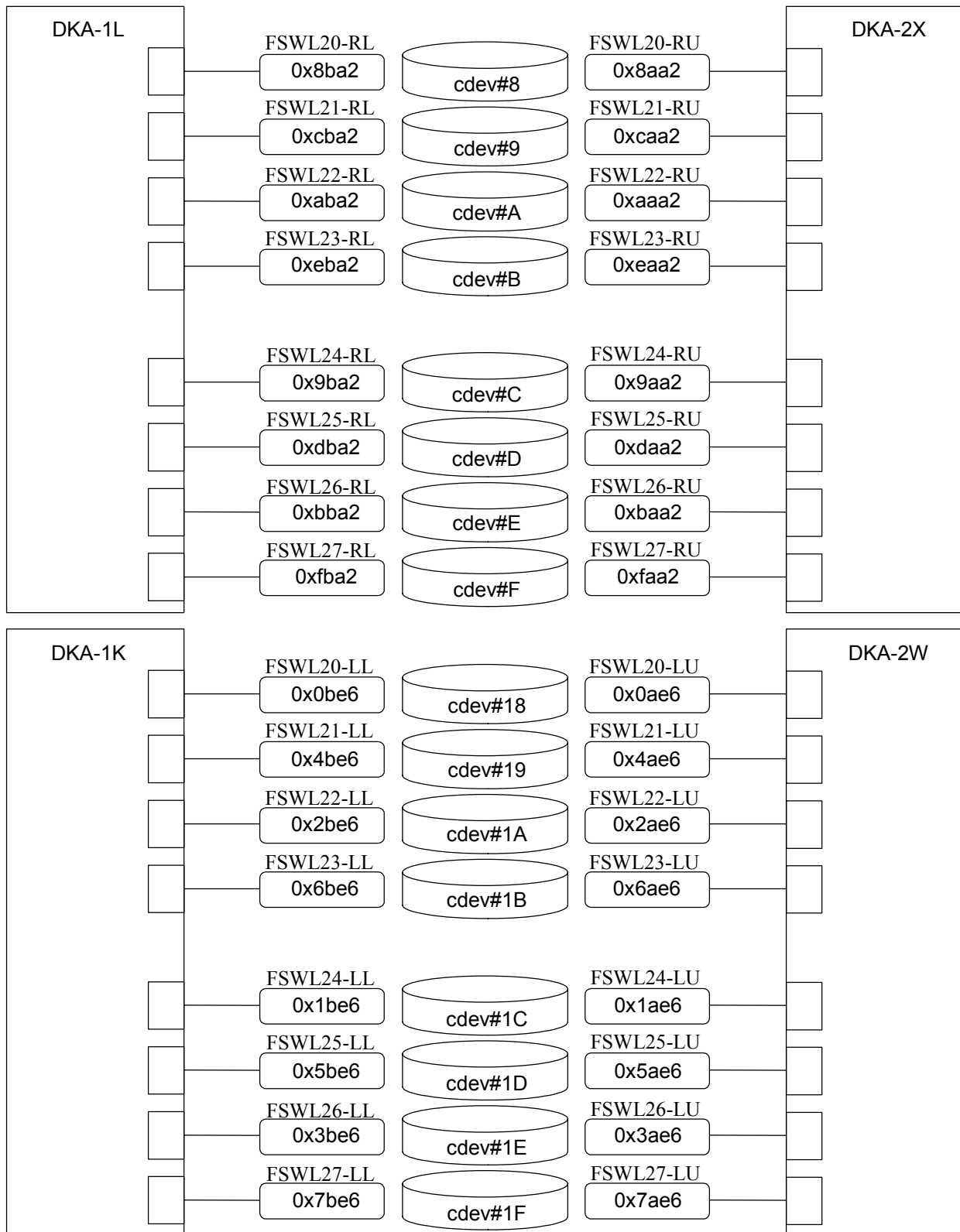
Fig. 6.2-5 DKA Path Address mapping (Hi-Performance Model : L2 Unit)
