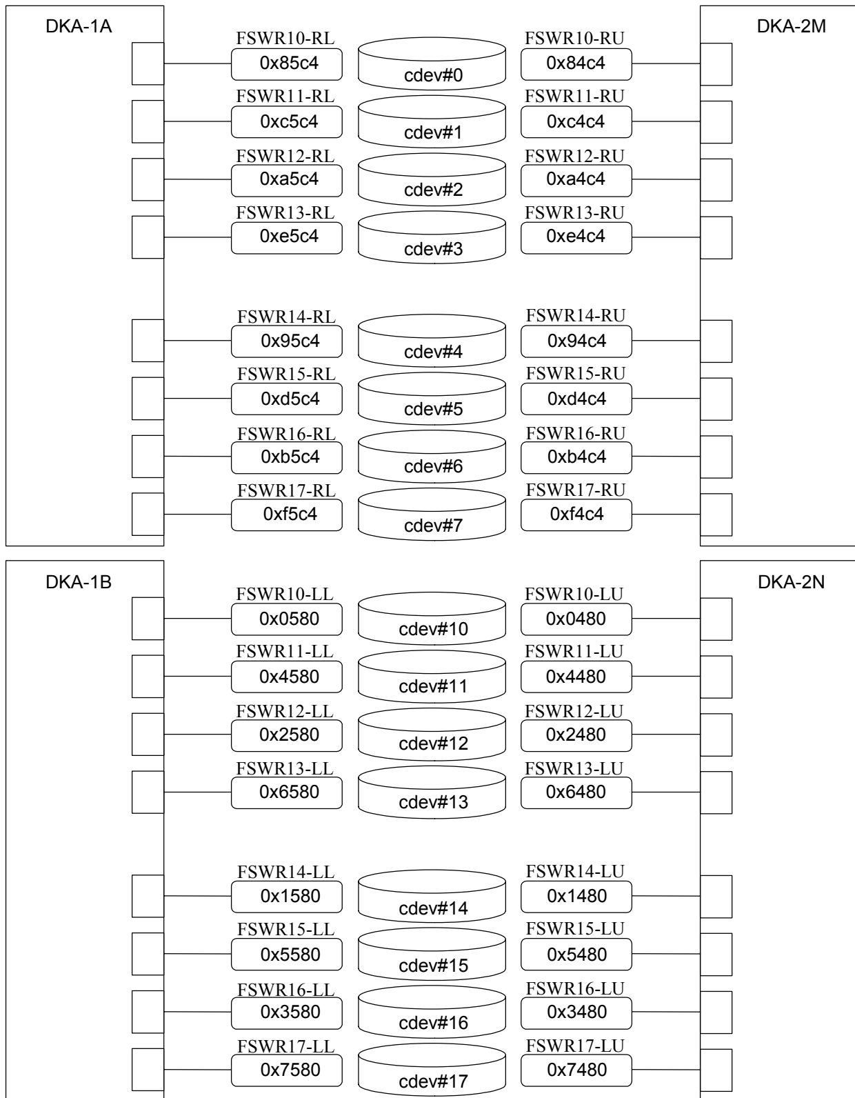
Fig. 6.2-2 DKA Path Address mapping (Hi-Performance Model : R1 Unit)
