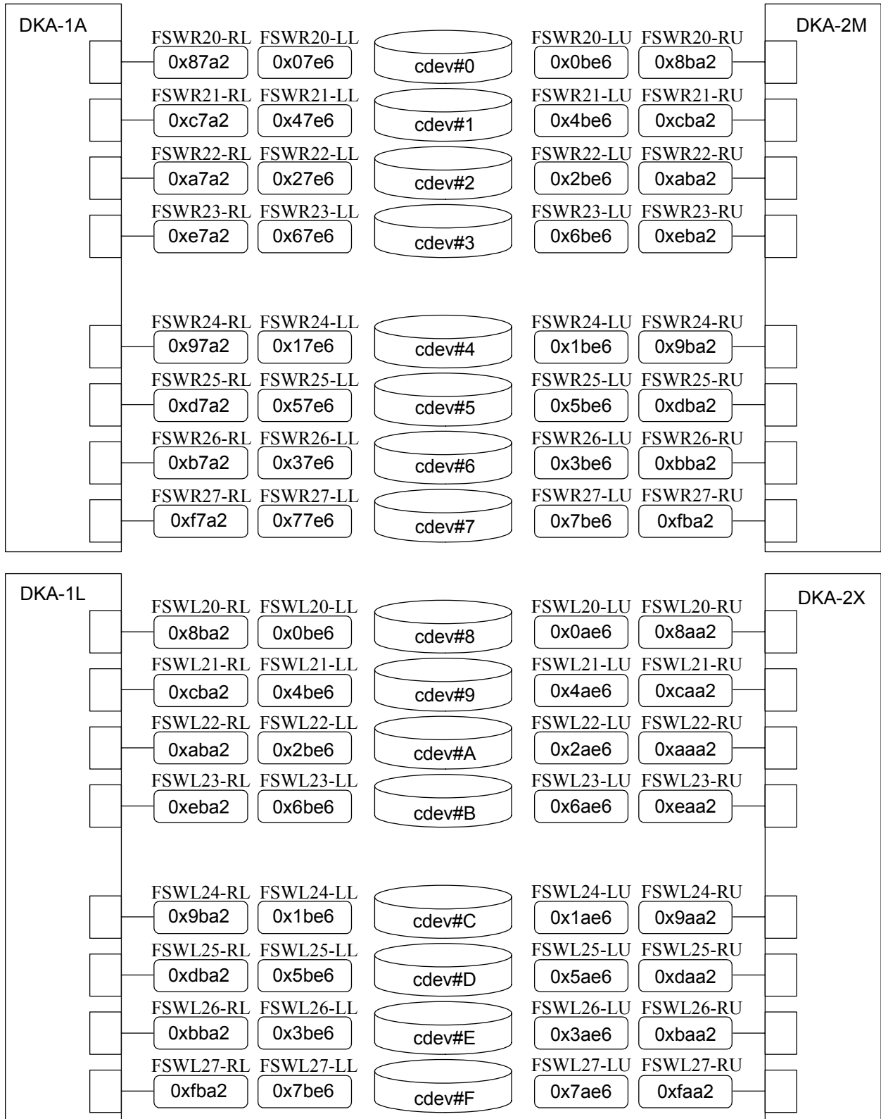
Fig. 6.2-7 DKA Path Address mapping (Standard Model : R2,L2 Unit)
