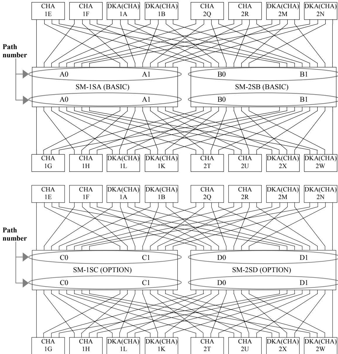
SHSN Logical path layout
