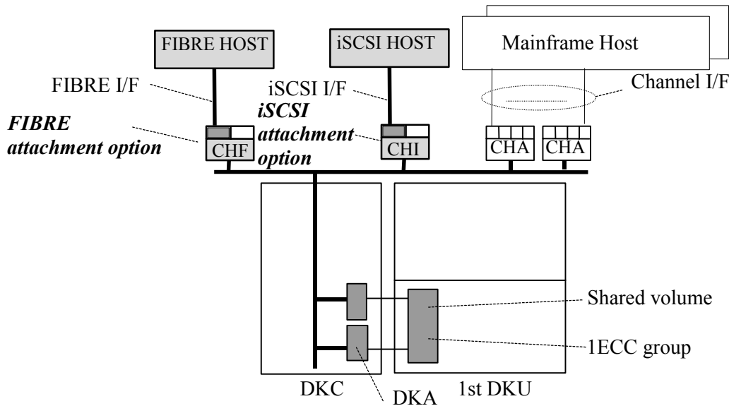
Fig. 3.1.1-1 multiplatform configuration example
