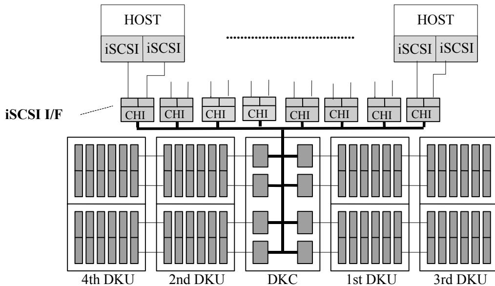
Fig. 3.1.3-2 Maximum system configuration example for All iSCSI
