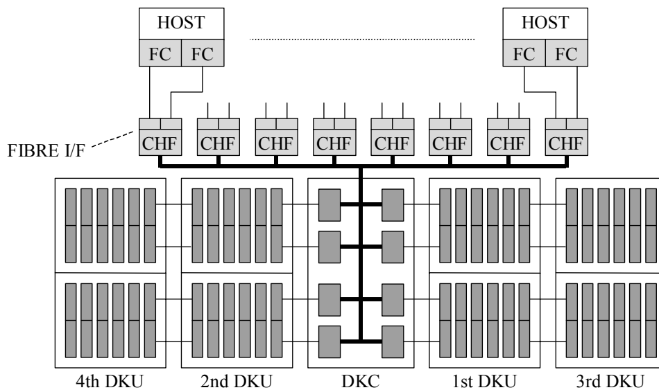
Fig. 3.1.2-2 Maximum system configuration example for All FIBRE
