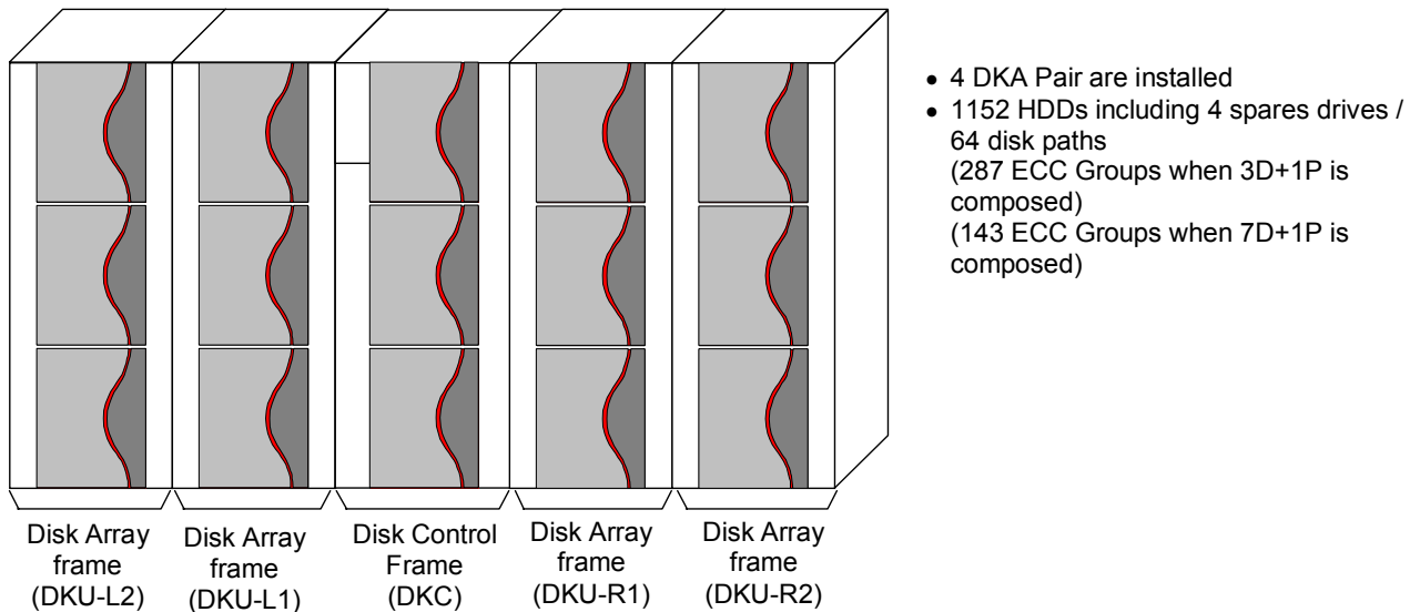
Fig. 3.6.1-2 Maximum volume configuration
