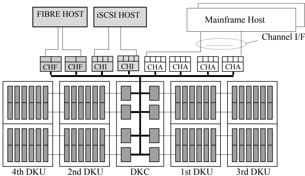
Fig. 3.1.1-2 multiplatform configuration example
