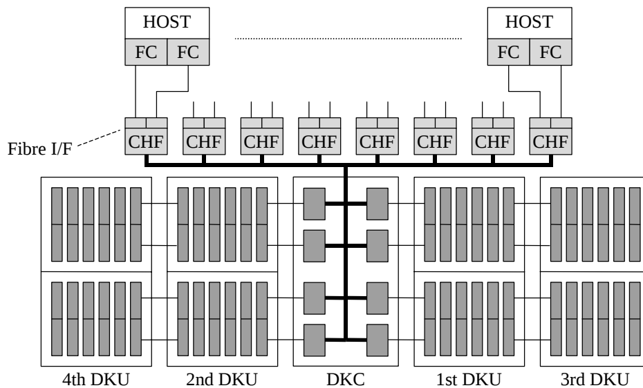
Fig. 3.1.2-2 Maximum system configuration example for All Fibre
