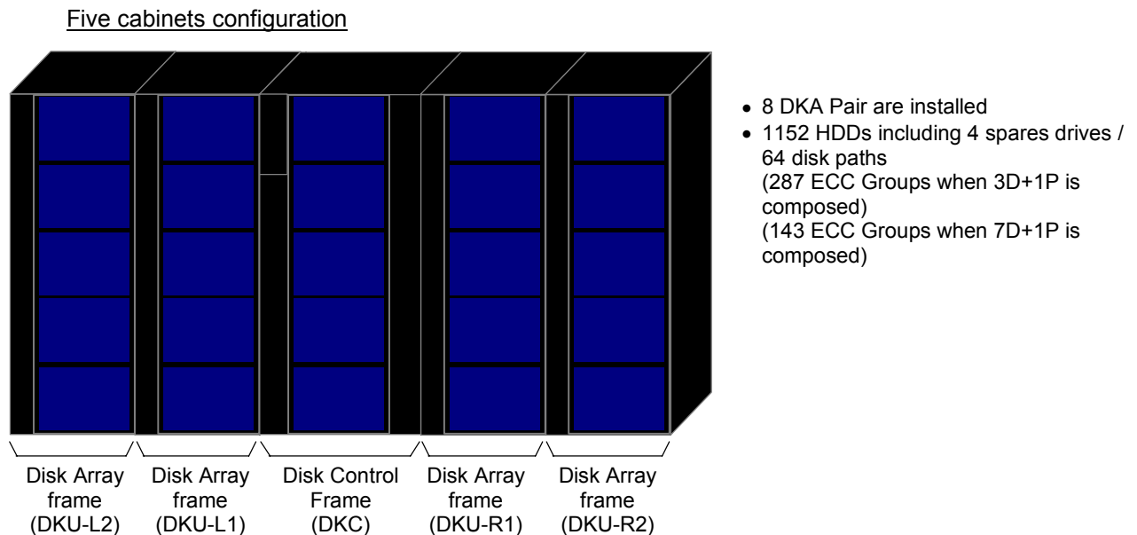
Fig. 3.6.1-2 Maximum volume configuration
