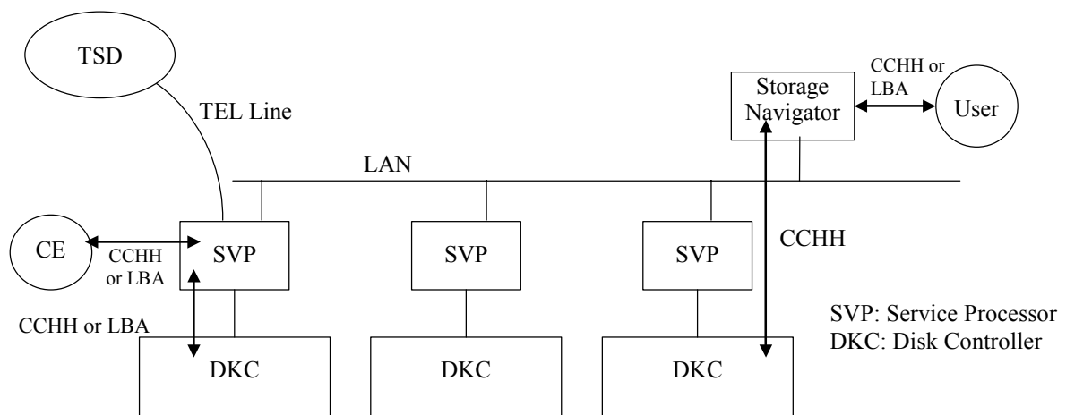
Fig. 2.4-1 Maintenance Execution Route when DCR Is Used
