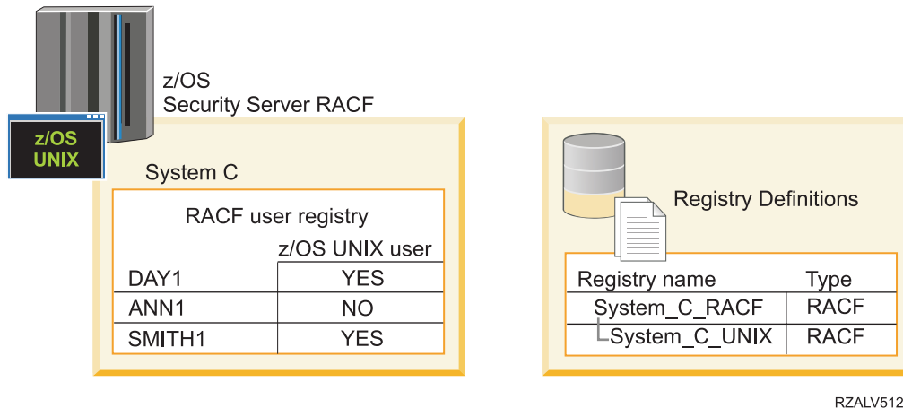
Figure 7: EIM registry definitions for the RACF user registry and for users of z/OS UNIX
