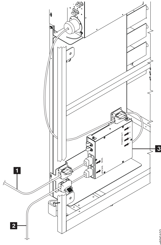
Figure 83. Dual AC power. The view is from the side and rear of a frame. The side panel has been removed to show the placement of the power switch and the two independent AC power cords.
