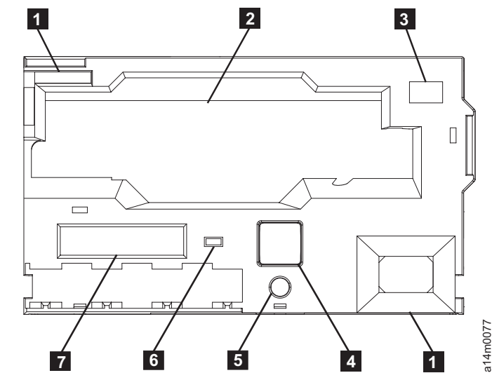
Figure 69. Front view of the 3592 J1A
