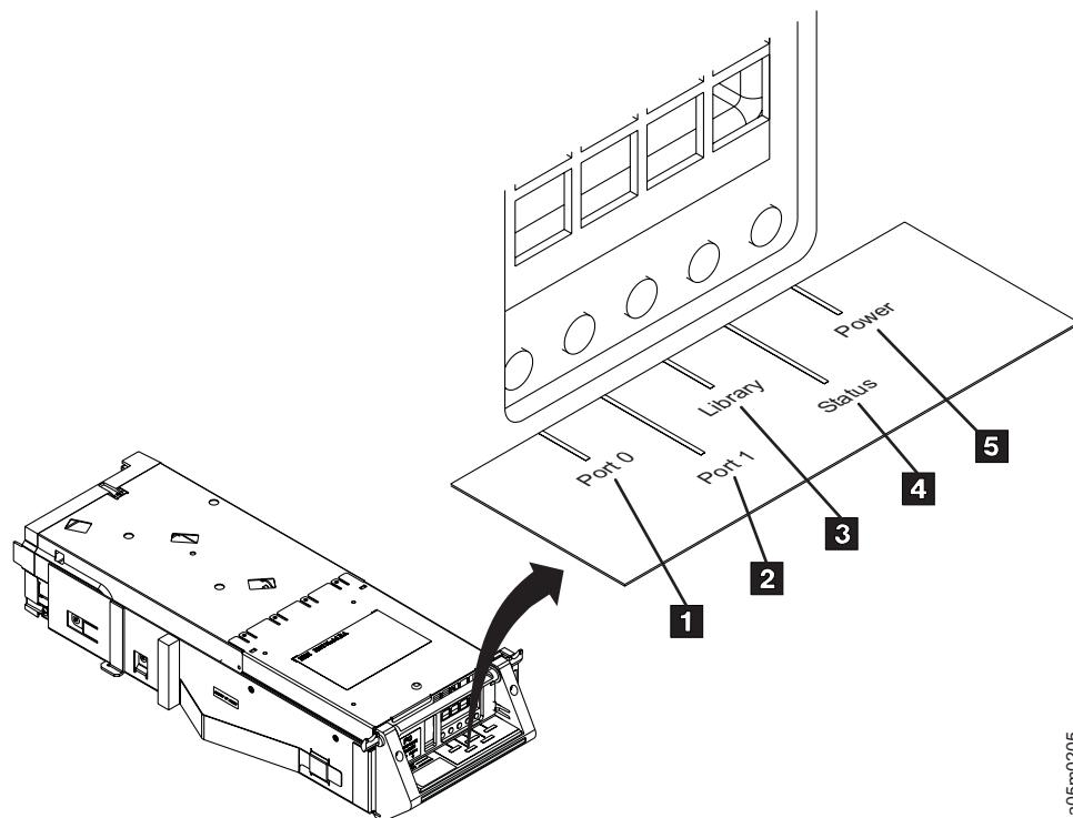
Figure 70. Rear view of the 3592 J1A
