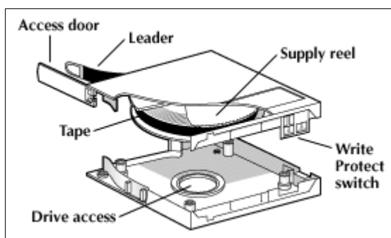
Figure 1-9 DLT cartridge
