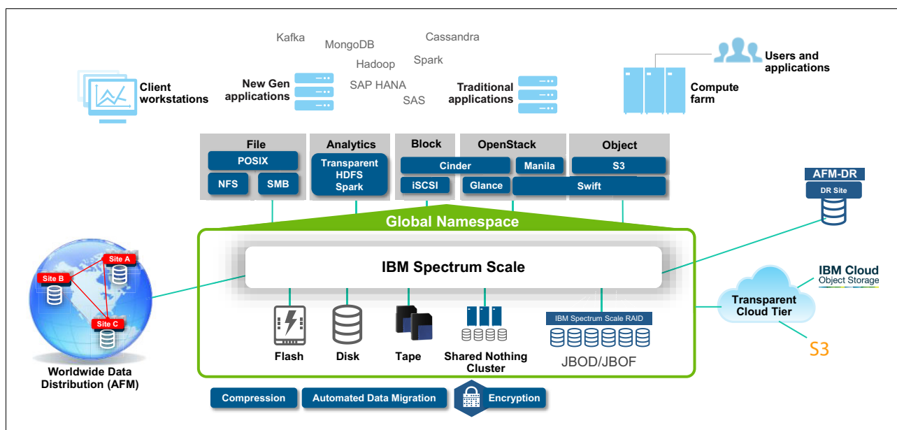
Figure 1-20 IBM Spectrum Scale Architecture
