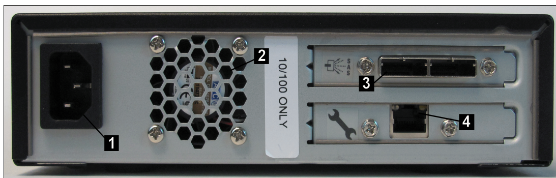
Figure 6-4 Rear view of the TS2270 tape drive
