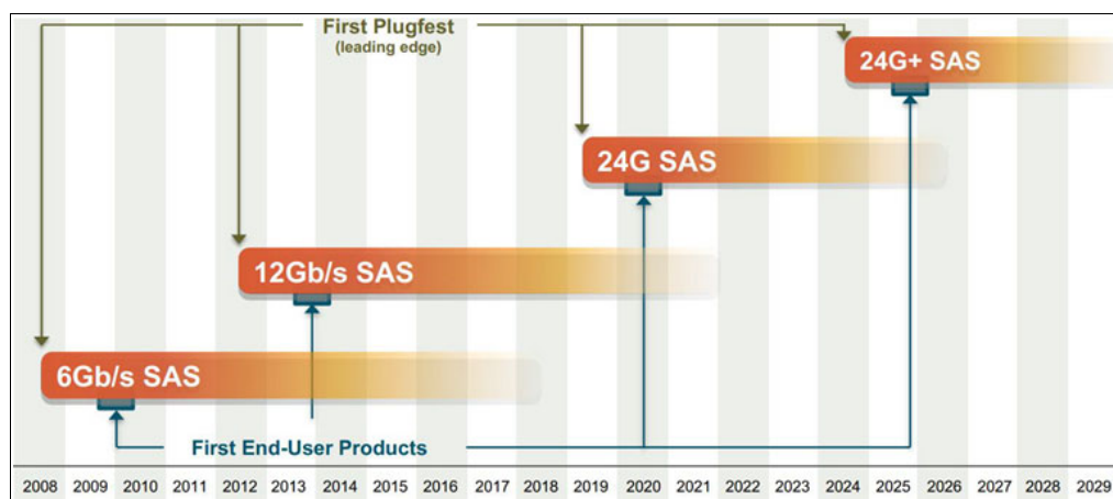
Figure 2-13 SAS roadmap 2
