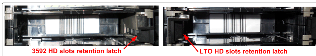
Figure 11-11 HD slot
