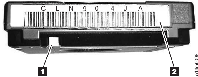
Figure 55. Characteristics that identify the 3592 cleaning cartridge
