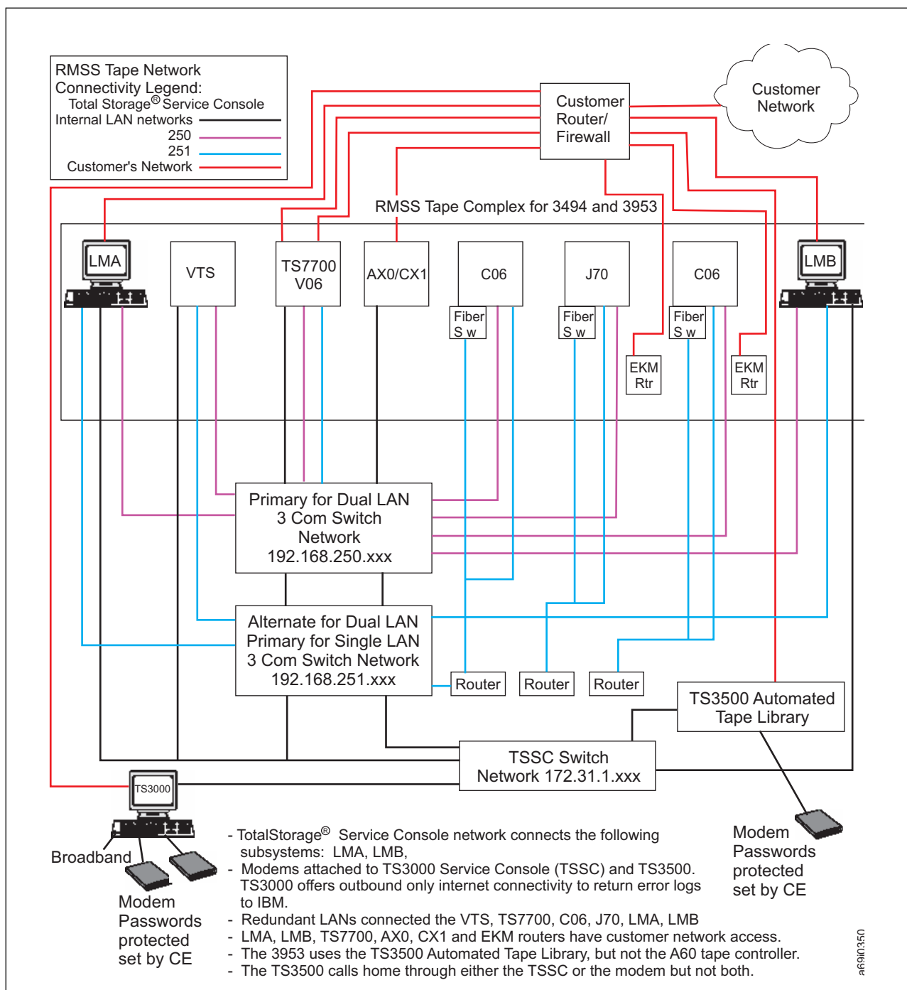
Figure 14. Attachment of the system console to the TS3500 tape library and the 3953 tape system for remote support
