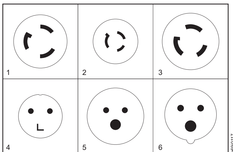
Figure 32. Types of receptacles for power cords used by models L32 and D32 of the TS3500 tape library
