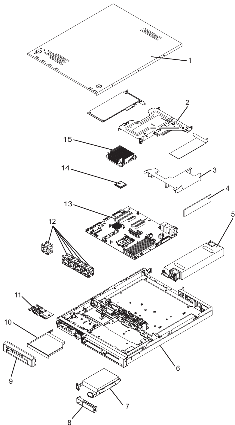
Figure 4. x3250 M3, 4252 Model PCJ FRU List
