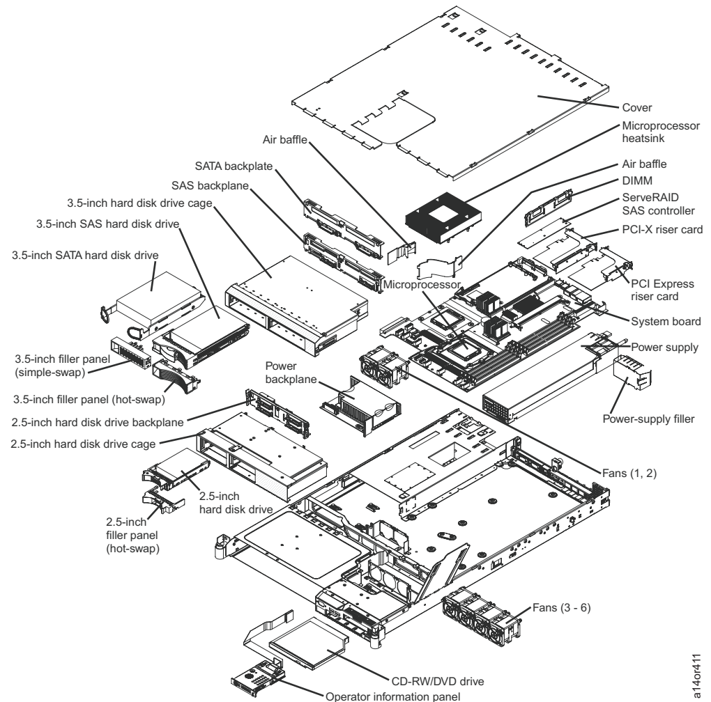
Figure 2. Model x3550 (type 7978) FRU List
