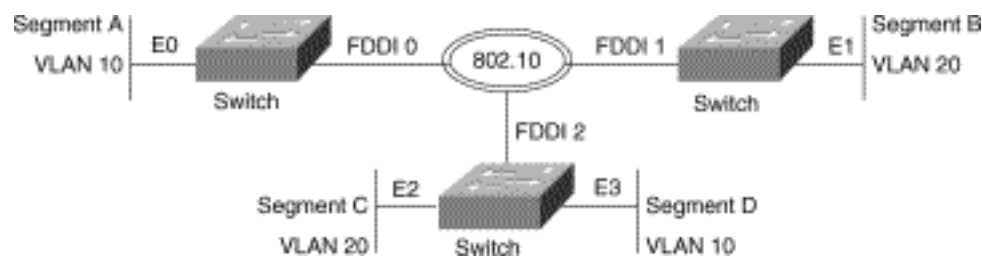
Figure 12-7: IEEE 802.10 switched backbone implementation.
