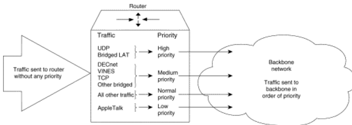
Figure 2-4: Priority queuing.
