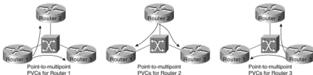
Figure 8-27: Switch-based broadcasting.
