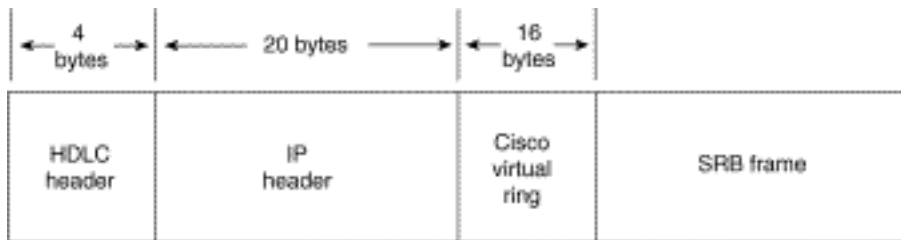
Figure 4-19: SRB frame encapsulated in FST with HDLC header.
