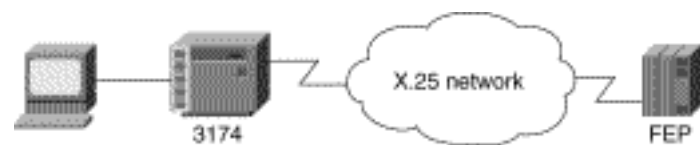
Figure 5-17: Typical QLLC topology.
