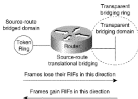
Figure 2-15: Source-route translational bridging topology.
