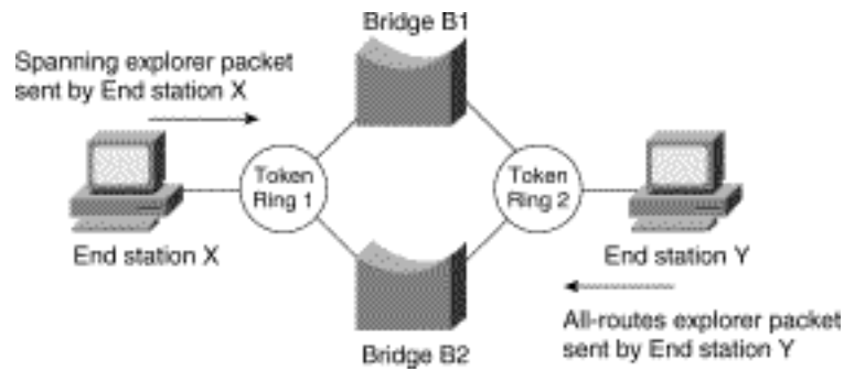
Figure 4-6: Explorer packet processing (spanning explorer broadcast).
