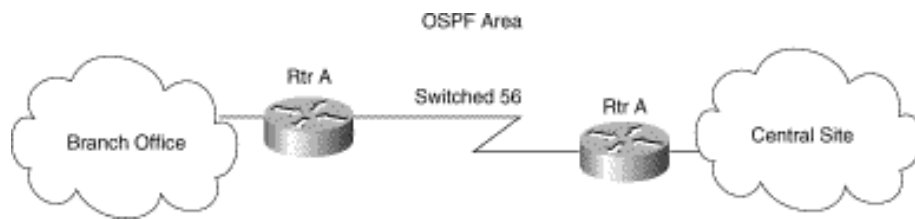
Figure 3-16: OSPF area.
