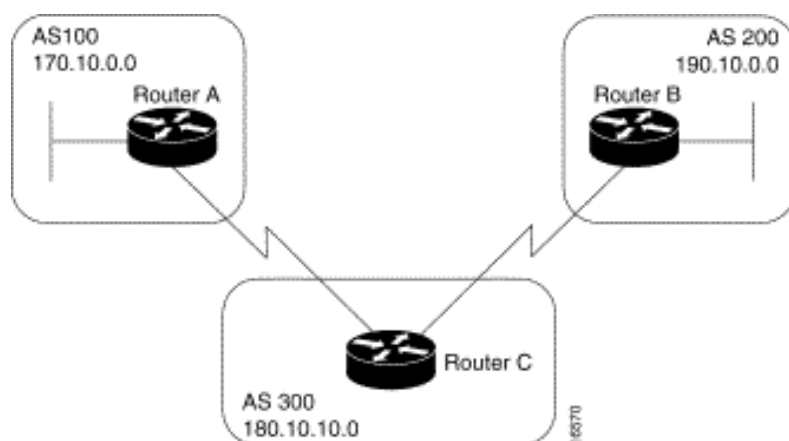
Figure 3-24: AS_path attribute.
