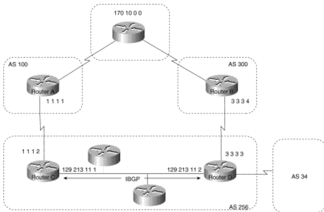
Figure 3-30: Local preference.
