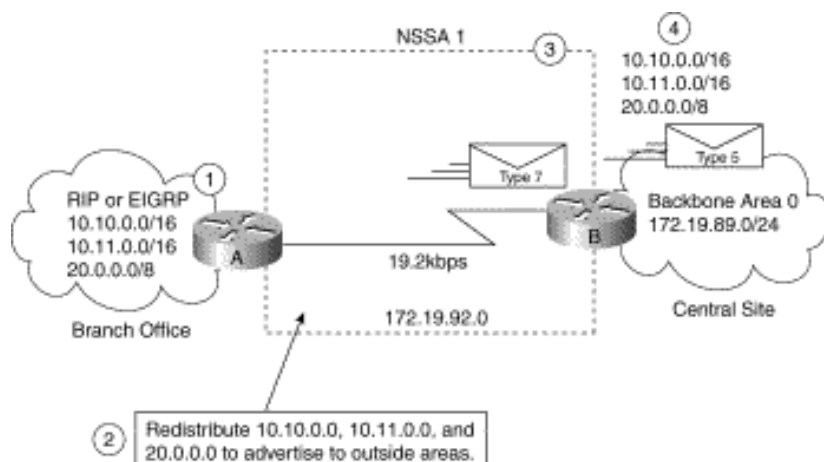
Figure 3-14: OSPF NSSA operation.
