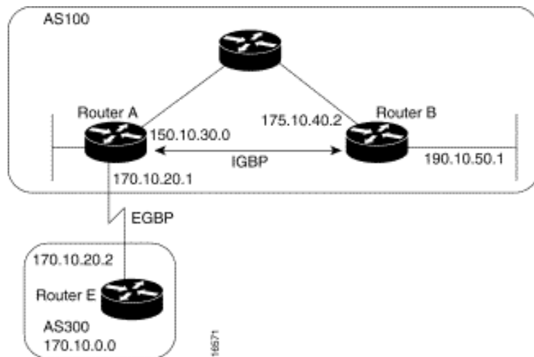
Figure 3-25: Origin attribute.
