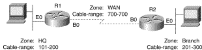
Figure 10-6: AppleTalk snapshot routing.
