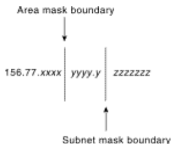
Figure 3-12: Areas and subnet masking.
