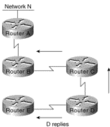
Figure 3-9: DUAL example (part 3): switching to a feasible successor.
