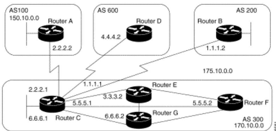
Figure 3-36: BGP peer groups.
