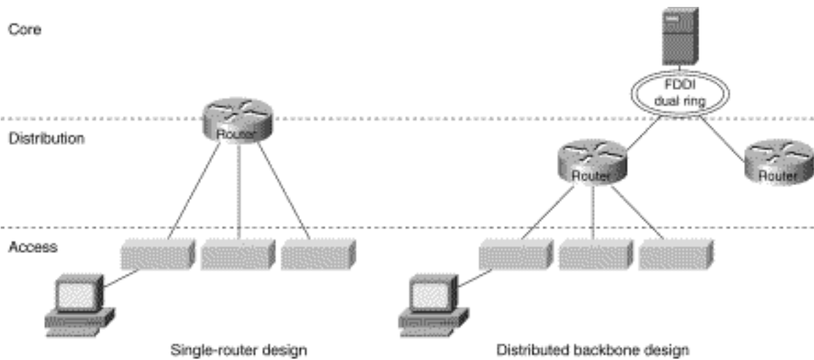
Single-router design
