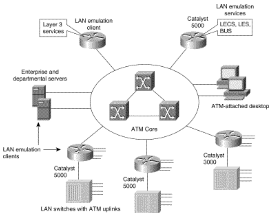
Figure 8-13: Components of an ATM LANE network.
