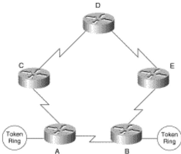
Figure 4-28: Convergence topology.
