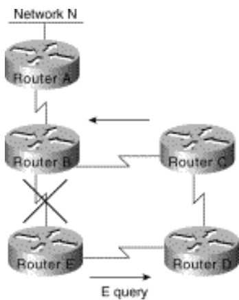
Figure 3-8: DUAL example (part 2): sending queries.
