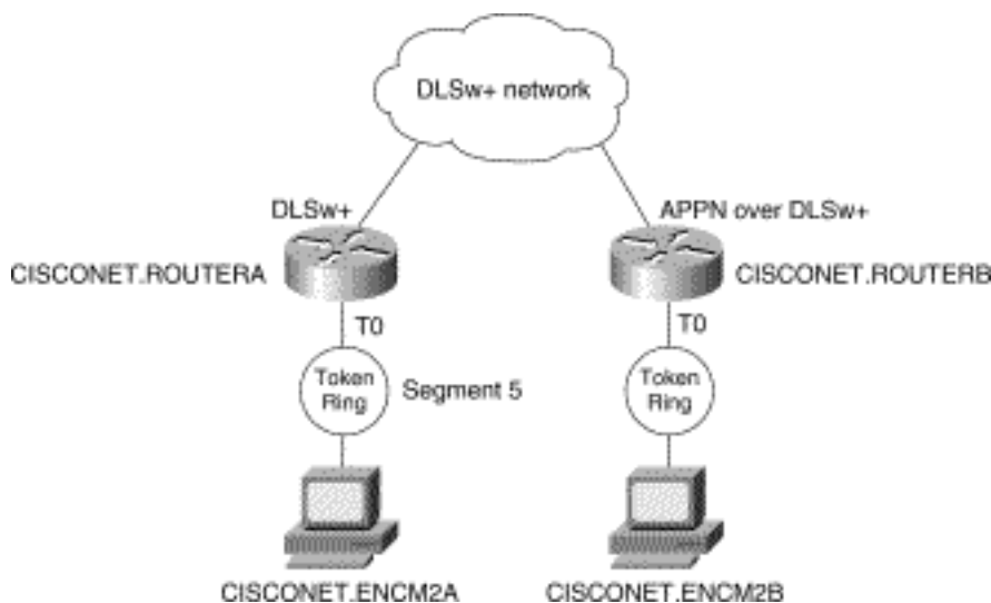
Figure 6-21: Example of APPN with DLSw+.
