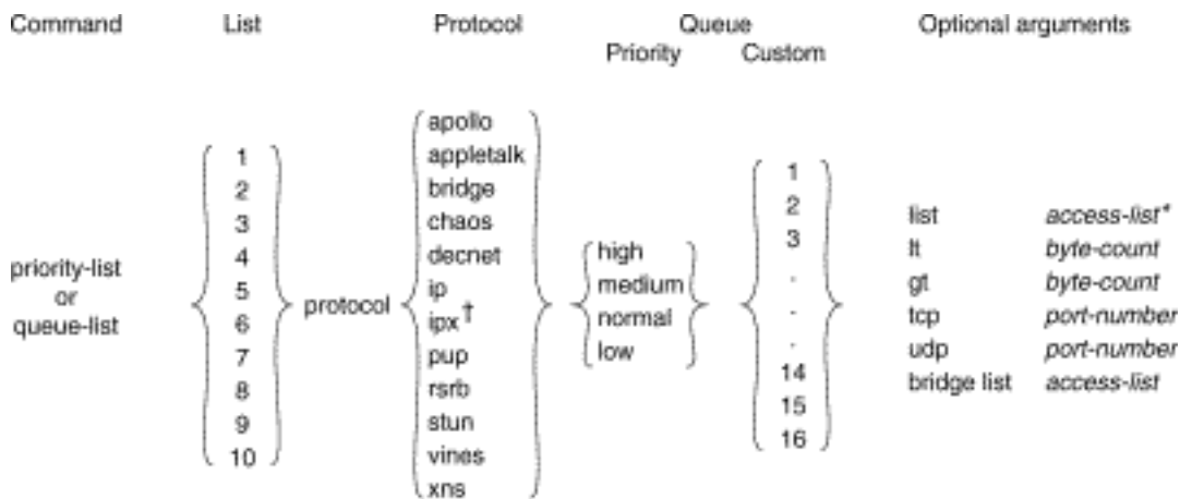
Figure 4-36: Priority and custom queuing command syntax.
