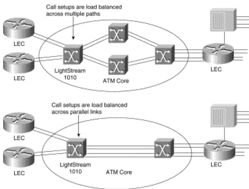
Figure 8-17: Load balancing calls across multiple paths and multiple links.
