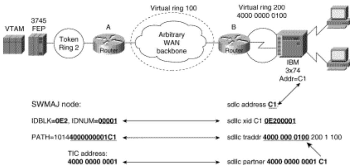
Figure 5-12: Required end-to-end SDLLC information.
