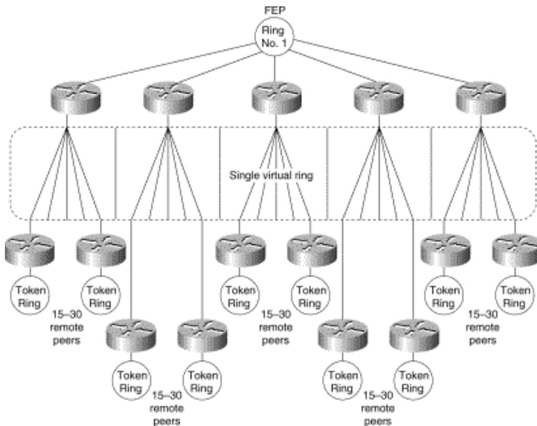
Figure 4-34: Virtual ring environment interconnecting multiple remote peers.
