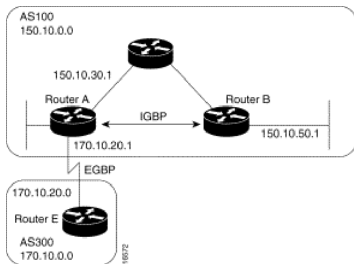
Figure 3-26: Next hop attribute.
