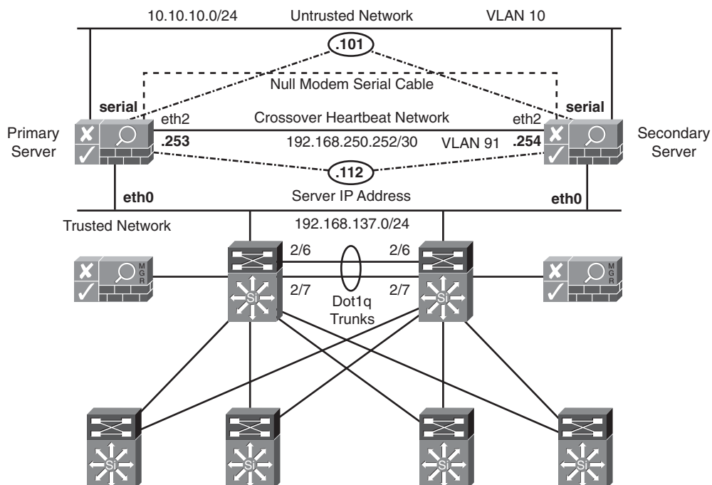
Figure 12-7 Sample NAC Appliance Server HA Network Topology
