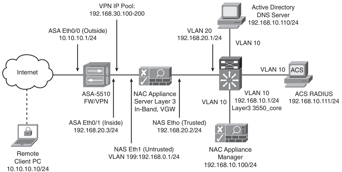
Figure 11-34 Deploying NAC over VPN
