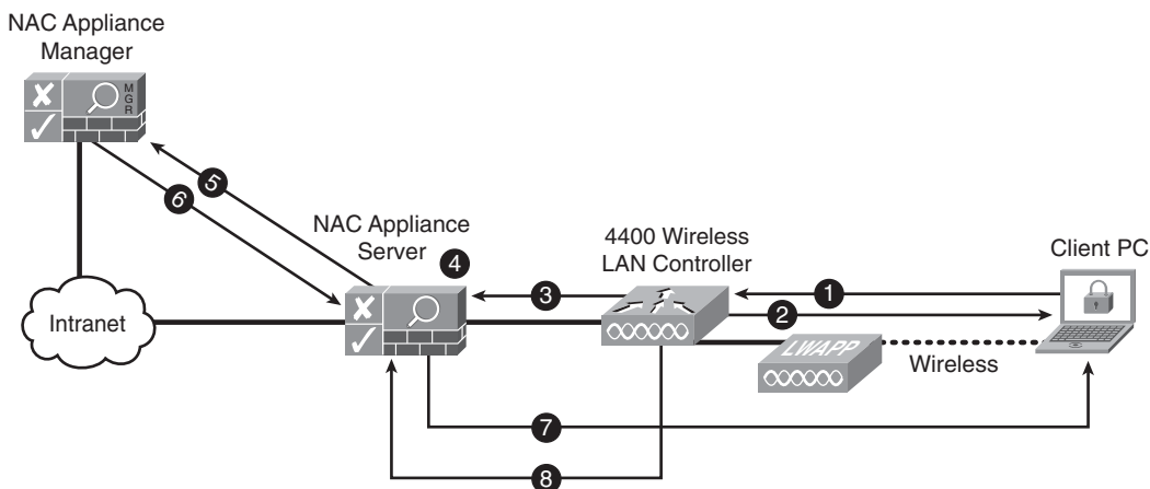
Figure 5-11 Wireless SSO Process
