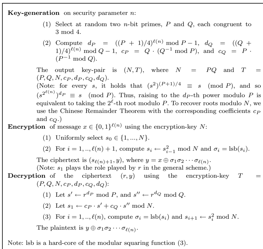
Fig. 5.3 The Blum–Goldwasser Public-Key Encryption Scheme (30). For simplicity we assume that \ell , which is polynomially bounded (e.g., \ell(n) = n ), is known at key-generation time.
