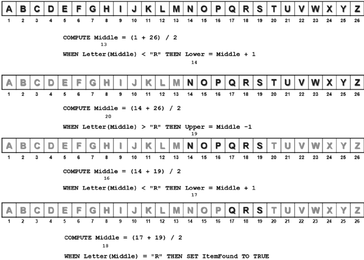
Figure 13-8. Finding the letter R using a binary search
