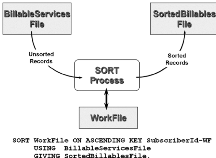
Figure 14-2. Diagram showing how the simple SORT works
