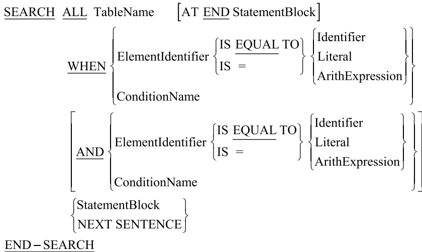
Figure 13-9. Metalanguage for SEARCH ALL
