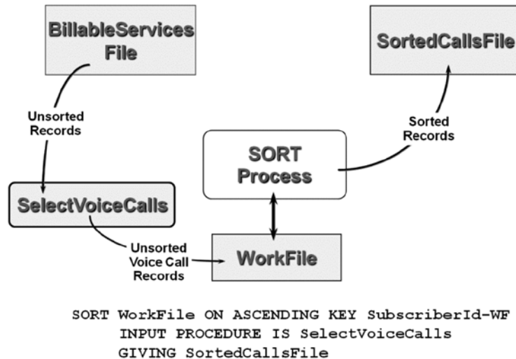
Figure 14-5. INPUT PROCEDURE used to select the voice call records
