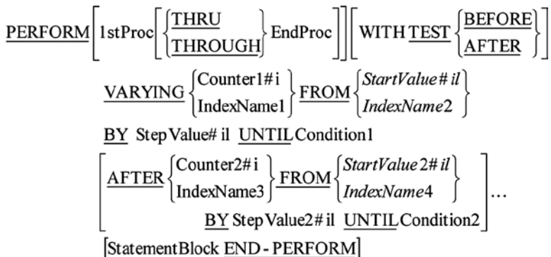
Figure 2-3. PERFORM. .VARYING metalanguage
