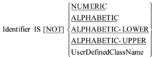
Figure 5-3. Metalanguage for class conditions
