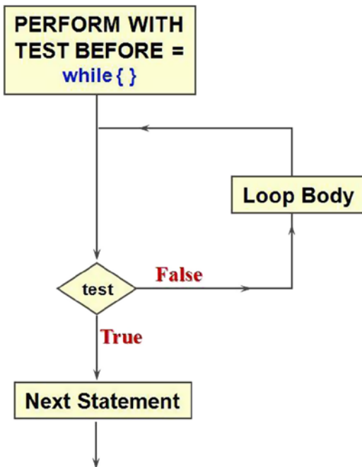
Figure 6-4. Pre-test loop
