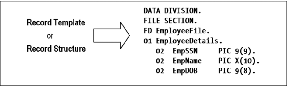
Figure 7-1. Record template/structure
