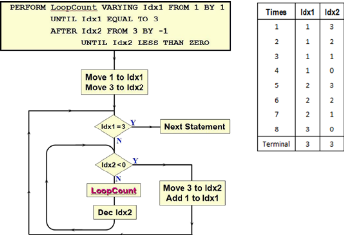
Figure 6-7. PERFORM..VARYING..AFTER
