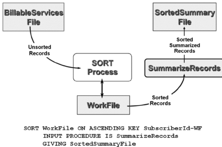
Figure 14-8. Using an OUTPUT PROCEDURE TO summarize records
