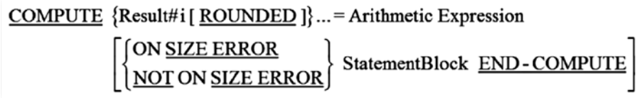
Figure 2-4. COMPUTE metalanguage syntax diagram
