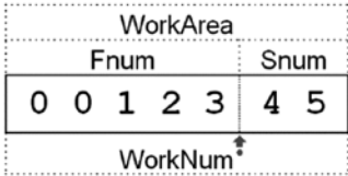
Figure 12-6. Model showing WorkArea, Fnum, and Snum redefined as WorkNum
