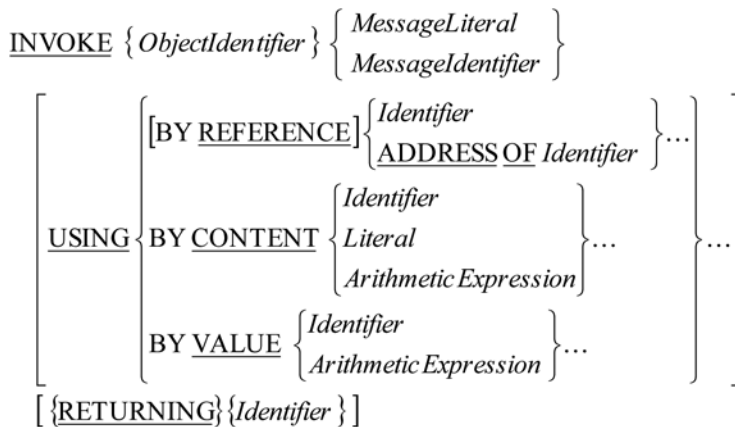
Figure 19-4. Metalanguage for the INVOKE verb
