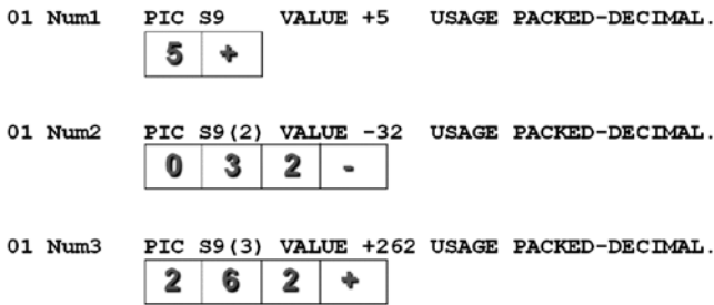
Figure 12-12. Memory representation of BCD numbers
