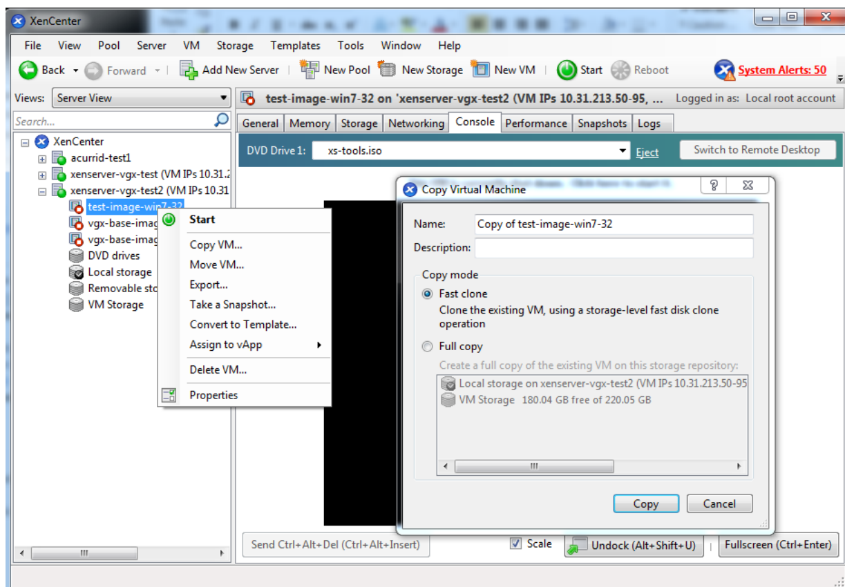
Figure 36. Cloning a VM using XenCenter
