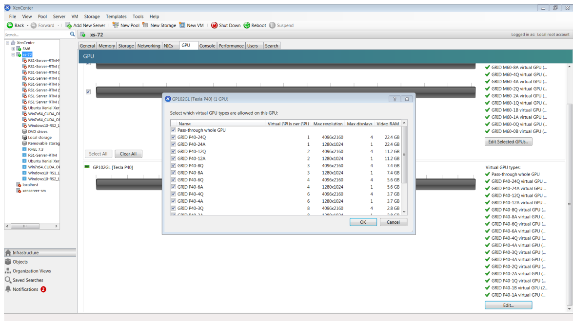
Figure 34. Editing a GPU's enabled vGPU types using XenCenter
