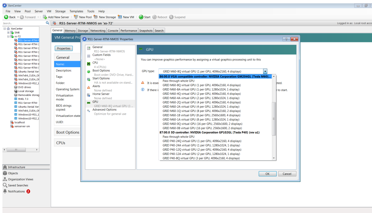
Figure 35. Using a custom GPU group within XenCenter
