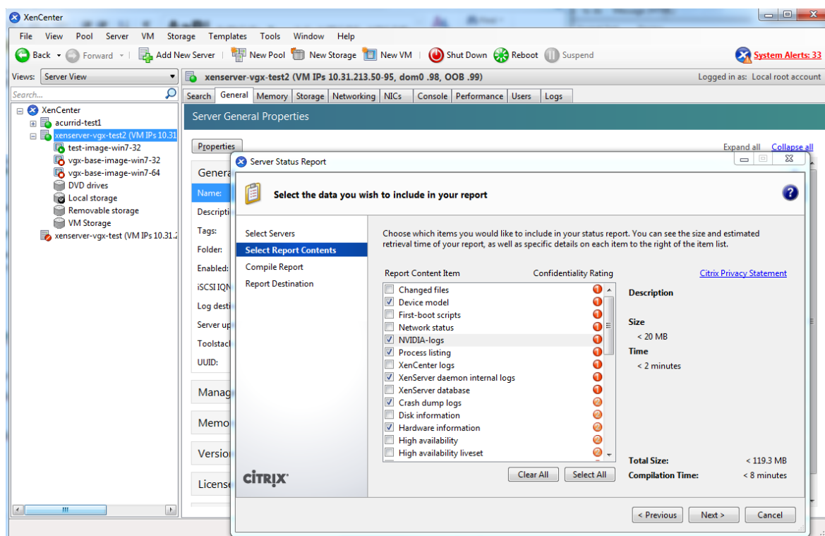
Figure 29. Including NVIDIA logs in a Citrix Hypervisor status report
