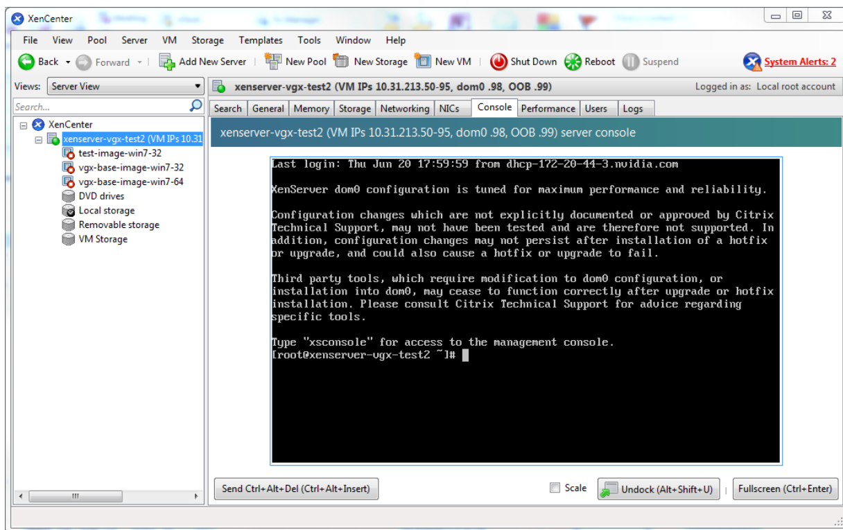
Figure 31. Connecting to the dom0 shell by using XenCenter
