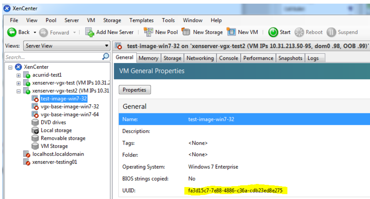
Figure 32. Using XenCenter to determine a VM's UUID
