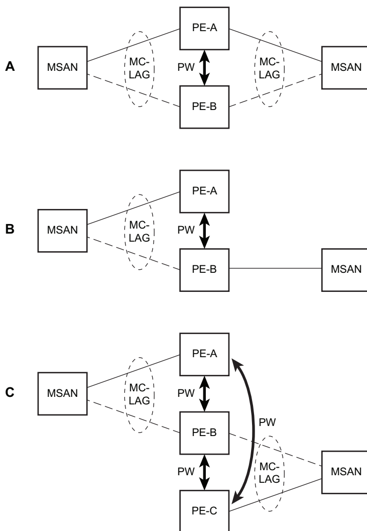
Figure 42 MC-LAG Layer 2 Dual Homing to Local PE-Pairs
