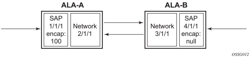
Figure 47 MTU Configuration Example
