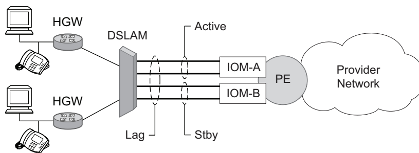
Figure 38 LAG on Access Interconnection
