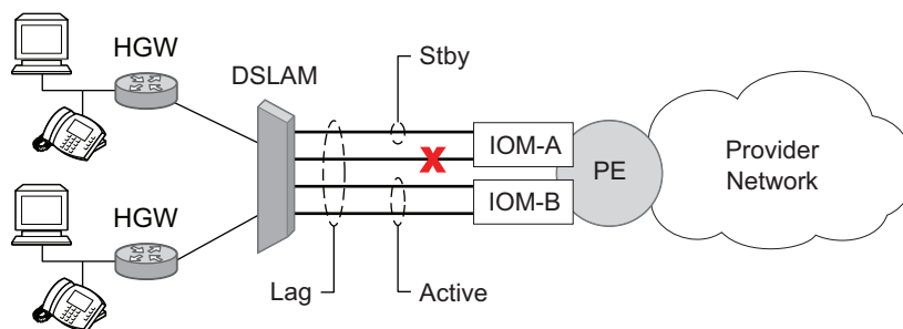
Figure 39 LAG on Access Failure Switchover
