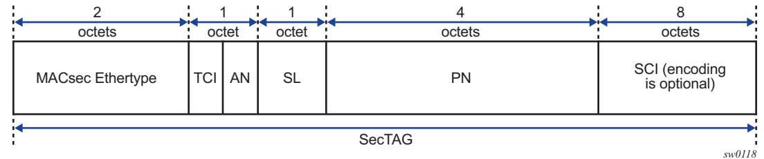
Figure 5 SecTAG Format
