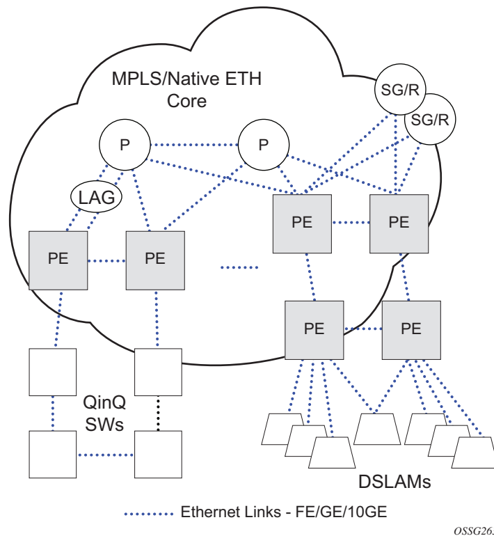
Figure 29 Generic Customer Use Case For LLDP
