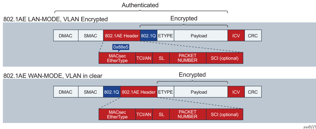
Figure 6 802.1 AE LAN/WAN Modes and VLAN Encrypted/Clear
