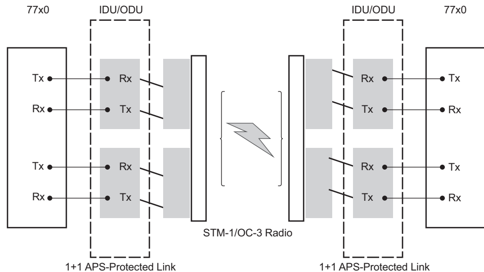
Figure 27 1+1 APS Protected Microwave SDH Transport
