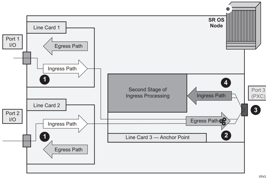
Figure 31 Traffic Pre-Processing Utilizing Cross-Connected Port (PXC)
