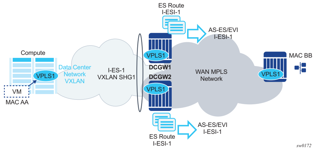
Figure 195 The Interconnect ES Concept
