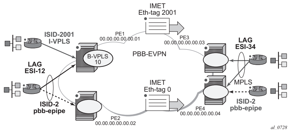
Figure 174 PBB-EVPN and I-VPLS Flooding Containment
