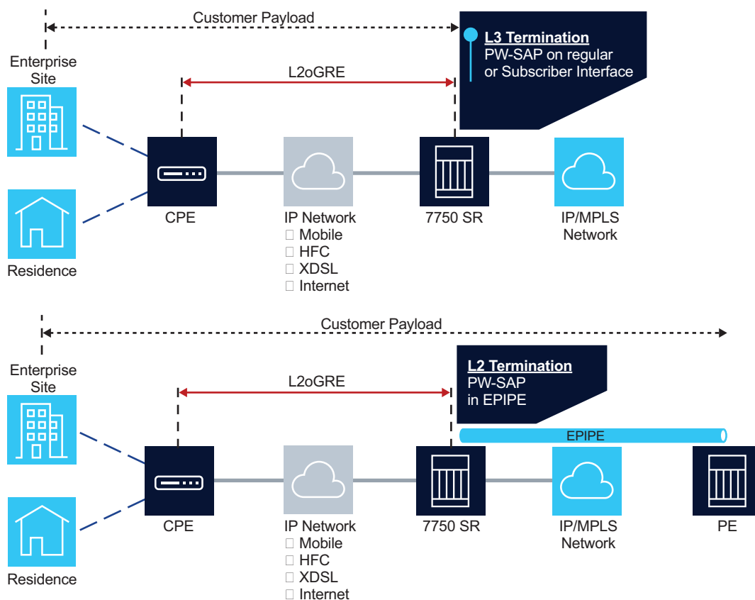
Figure 213 L2oGRE Network Examples
