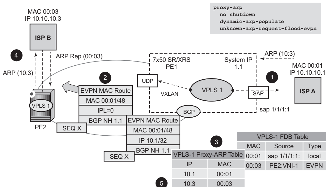
Figure 192 Proxy-ARP Example Usage in an EVPN Network
