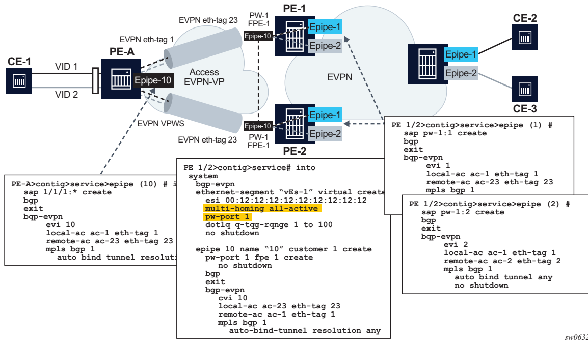
Figure 171 ES FPE-based pw-port - access EVPN-VPWS
