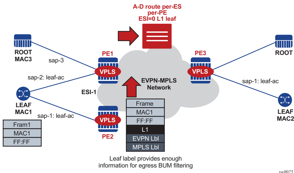
Figure 188 EVPN E-Tree BUM Egress Filtering and Multi-homing
