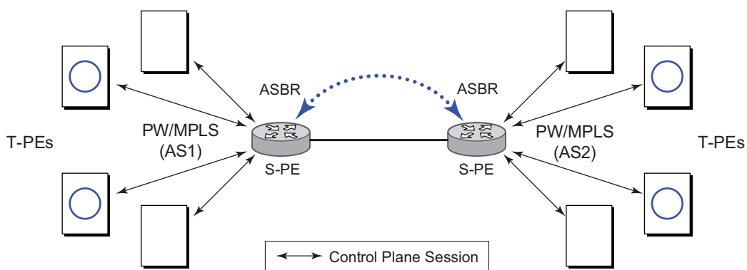
Figure 22 VLL Using Dynamic MS-PWs, Inter-AS Scenario
