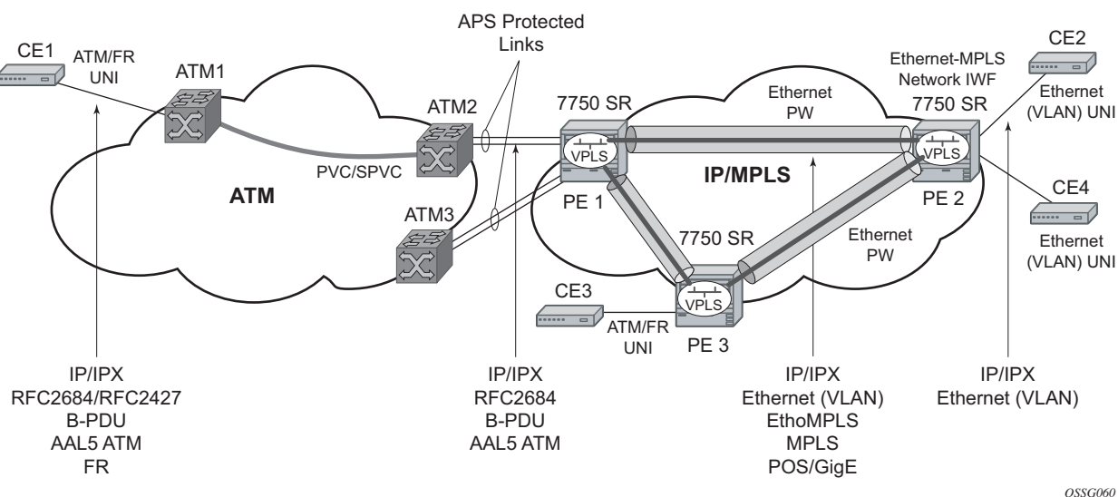
Figure 98 ATM/Frame Relay PVC Access and Termination on a VPLS Example
