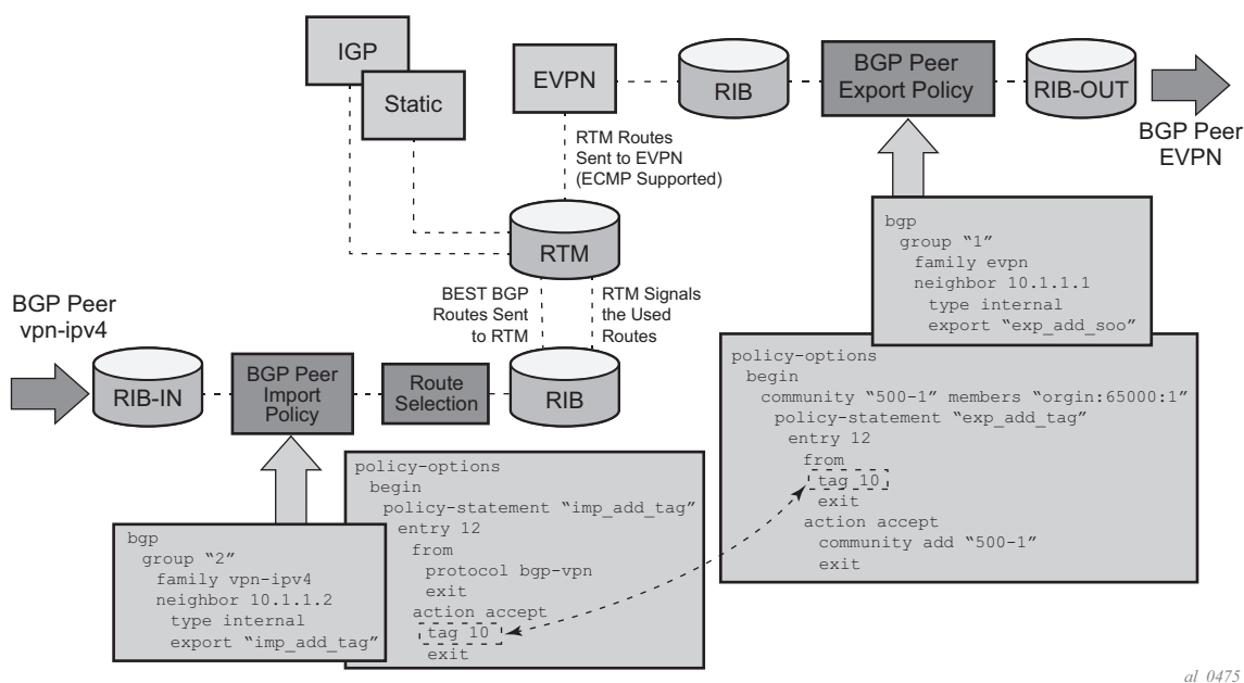
Figure 204 IP-VPN Import and EVPN Export BGP Workflow
