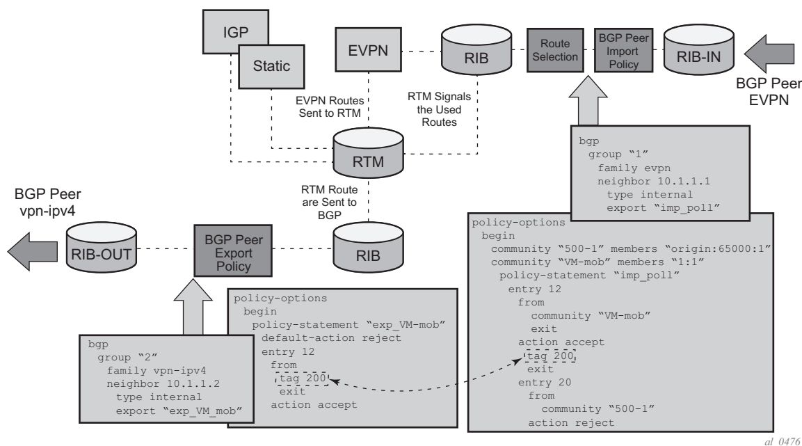
Figure 205 EVPN Import and I-VPN Export BGP Workflow
