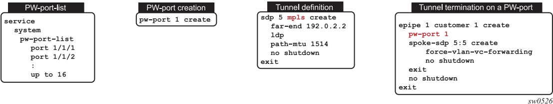
Figure 219 Provisioning MPLS-Based Spoke SDP Termination on a Flex PW Port
