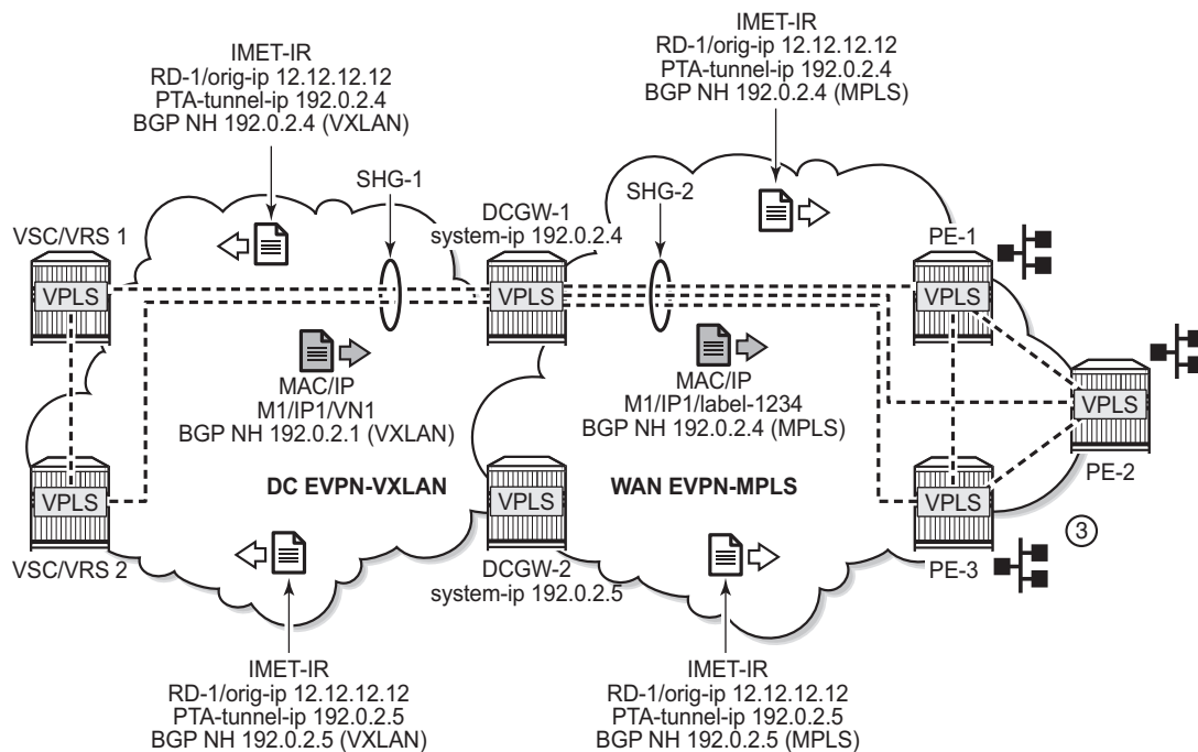
Figure 193 Multi-homed Anycast Solution
