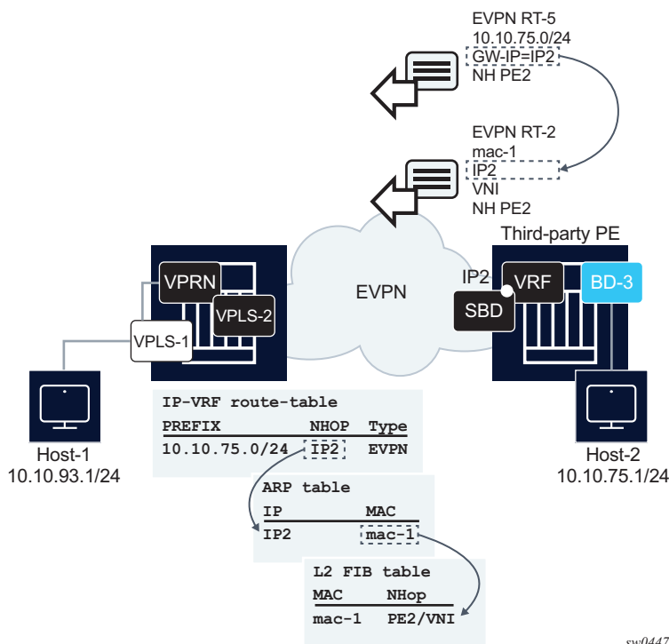
Figure 200 Interface-ful IP-VRF-to-IP-VRF with SBD IRB Model
