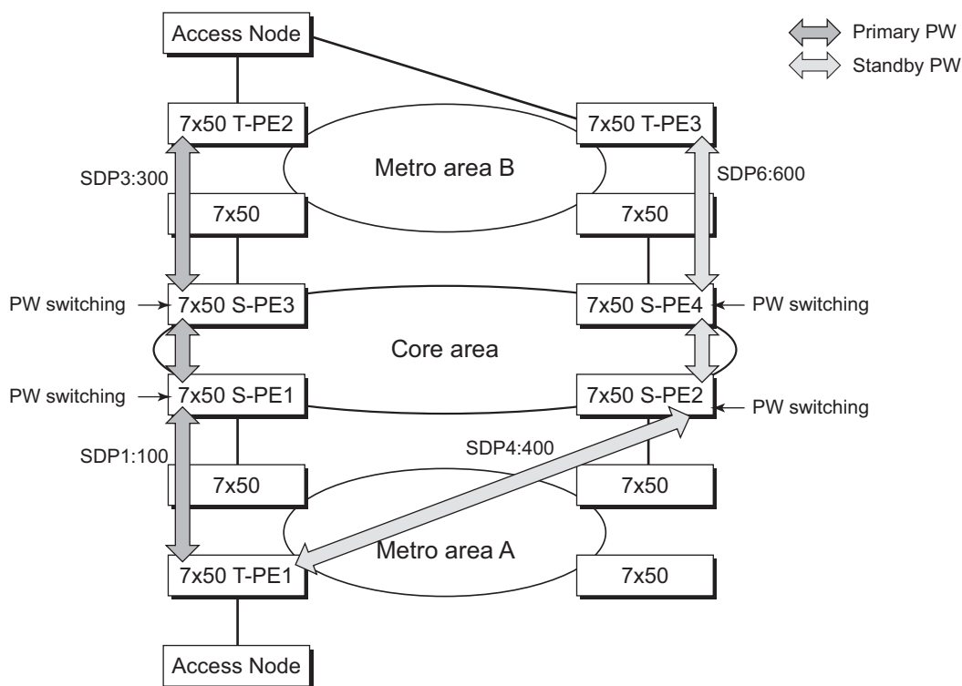
Figure 35 VLL Resilience with Pseudowire Redundancy and Switching
