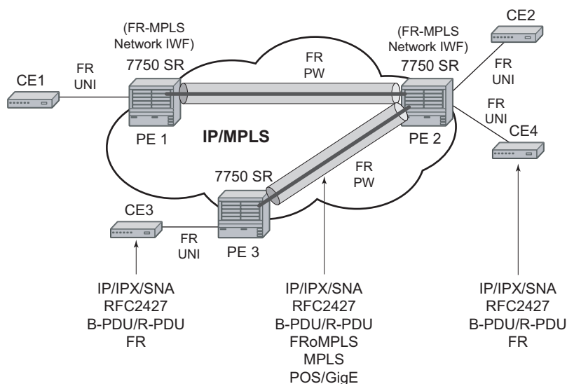
Figure 9 Application of a Fpipe
