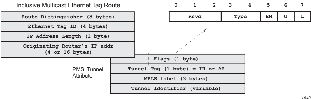
Figure 146 PMSI Attribute Flags Field for AR
