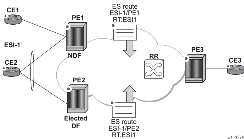
Figure 164 ES Discovery and DF Election
