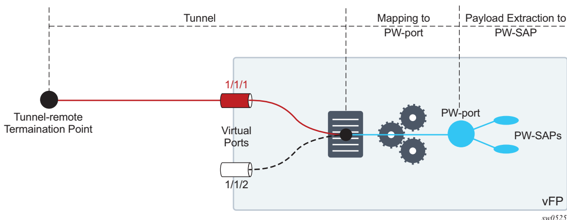
Figure 218 Flex PW Port
