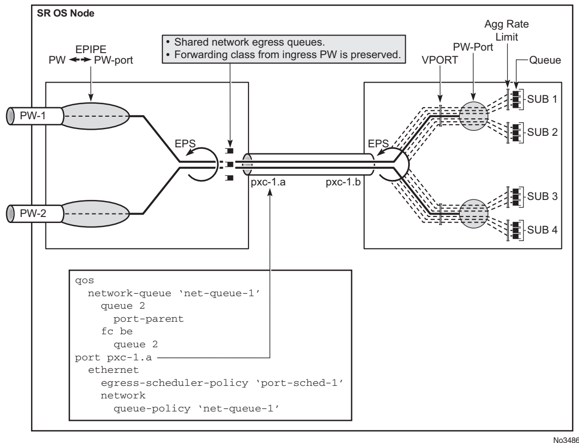
Figure 212 QoS on FPE-Based PW-Port
