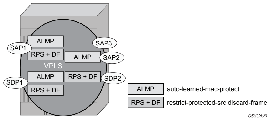
Figure 63 Auto-Learn-Mac-Protect Operation
