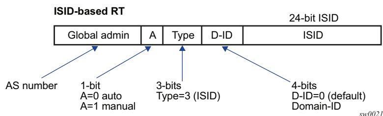
Figure 180 PBB-EVPN auto-rt ISID-based Route Target Format
