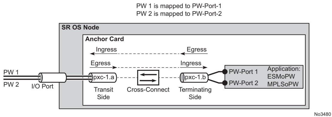
Figure 206 Multiplexing PWs over PXC-Based Internal Cross-Connect
