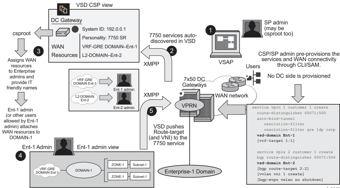
Figure 153 WAN Services Attachment Workflow
