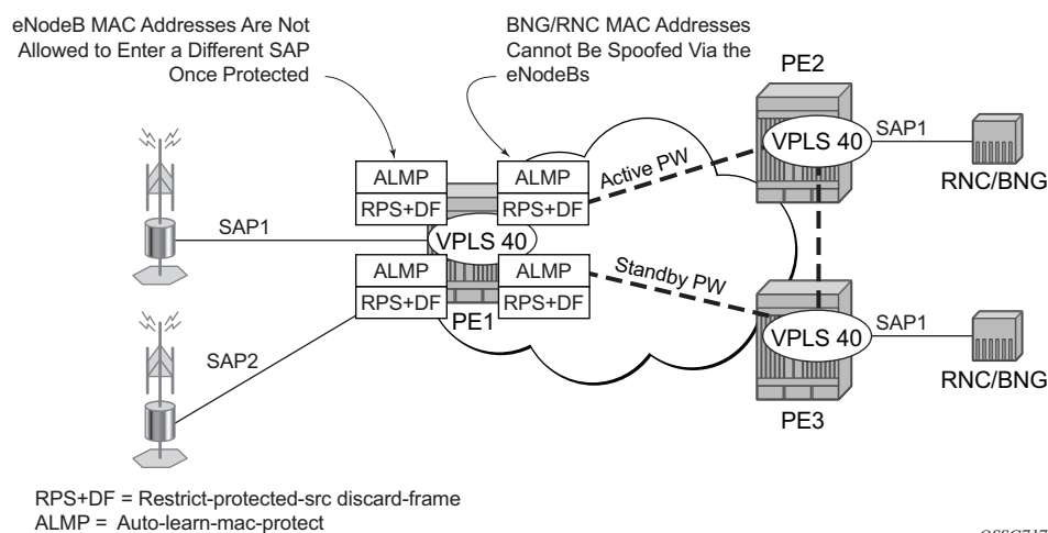
Figure 64 Auto-Learn-Mac-Protect Example
