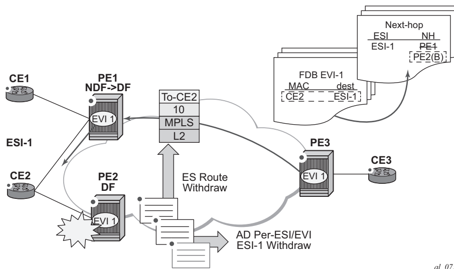
Figure 169 Single-Active Multi-Homing ES Failure
