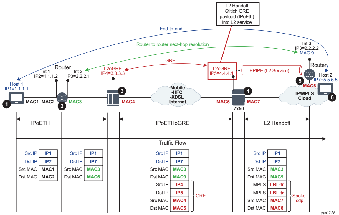
Figure 215 Layer 2 Termination and Hand-off
