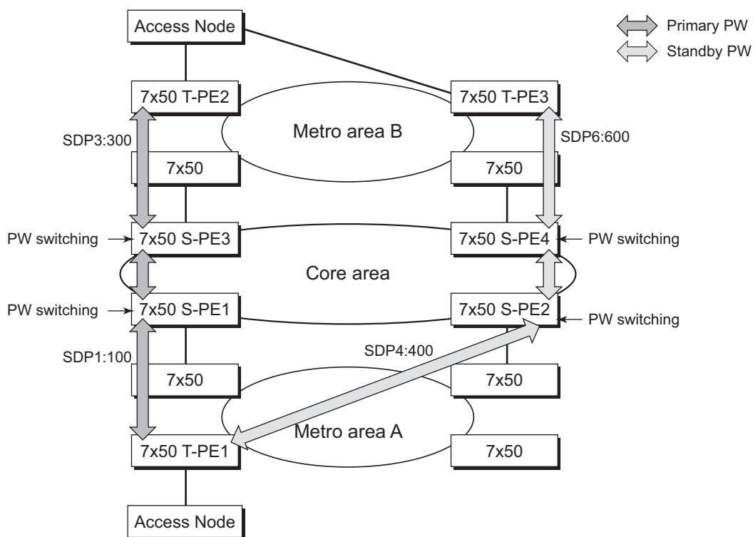
Figure 50 VLL Resilience with Pseudowire Redundancy and Switching
