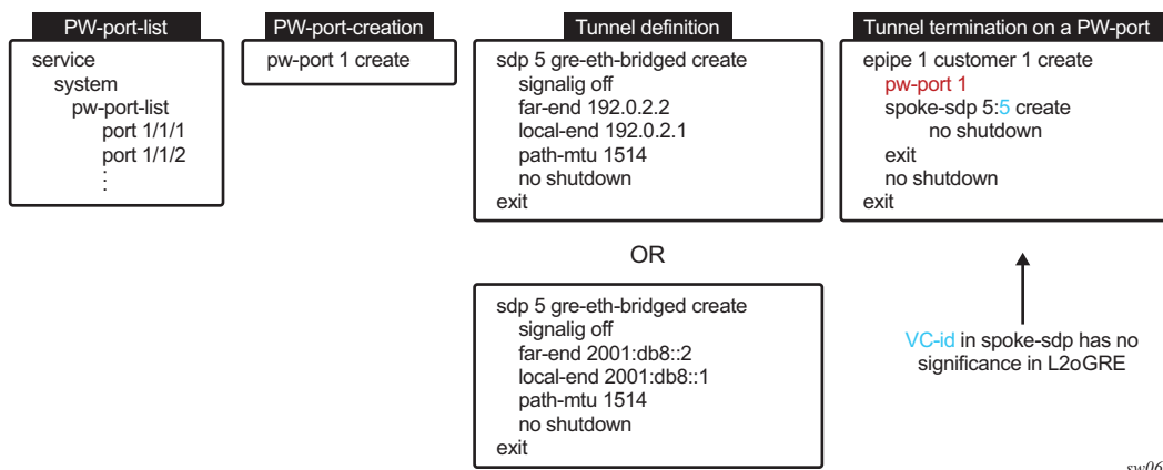
Figure 221 Provisioning L2oGRE Spoke-SDP termination on a Flew PW Port
