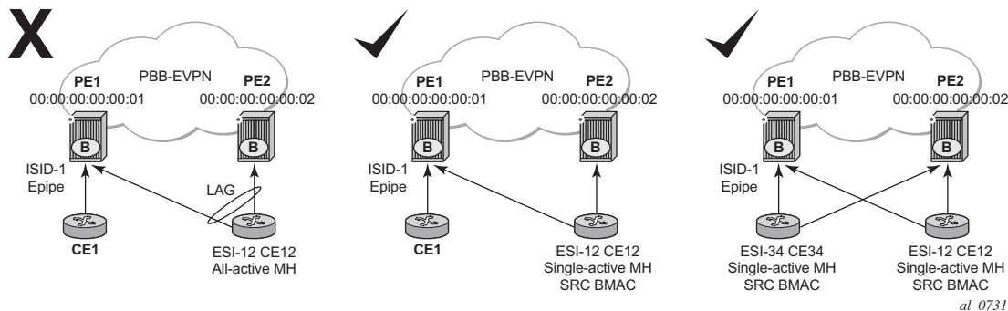
Figure 178 PBB-EVPN MH in a Two-Node Scenario
