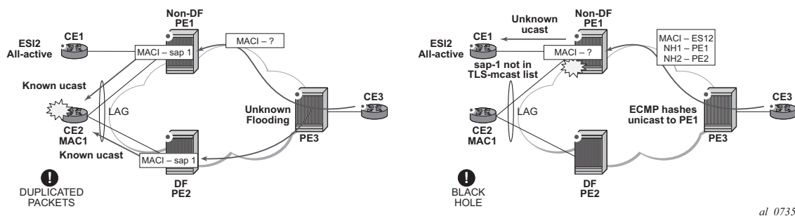
Figure 167 Transient Issues Caused by “slow” MAC Learning
