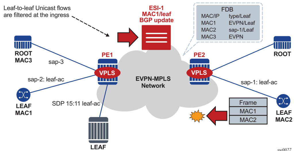
Figure 186 EVPN E-Tree Known Unicast Ingress Filtering
