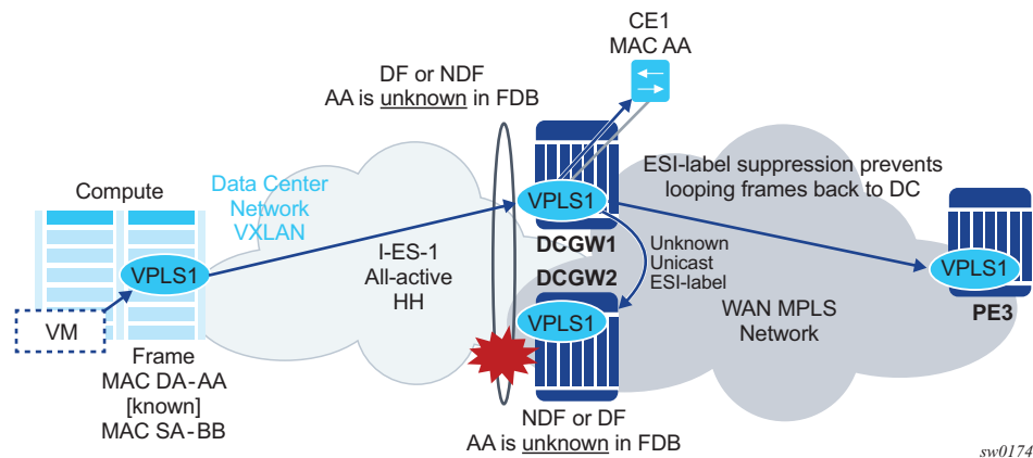
Figure 197 All-active Multi-Homing and Unknown Unicast on the NDF
