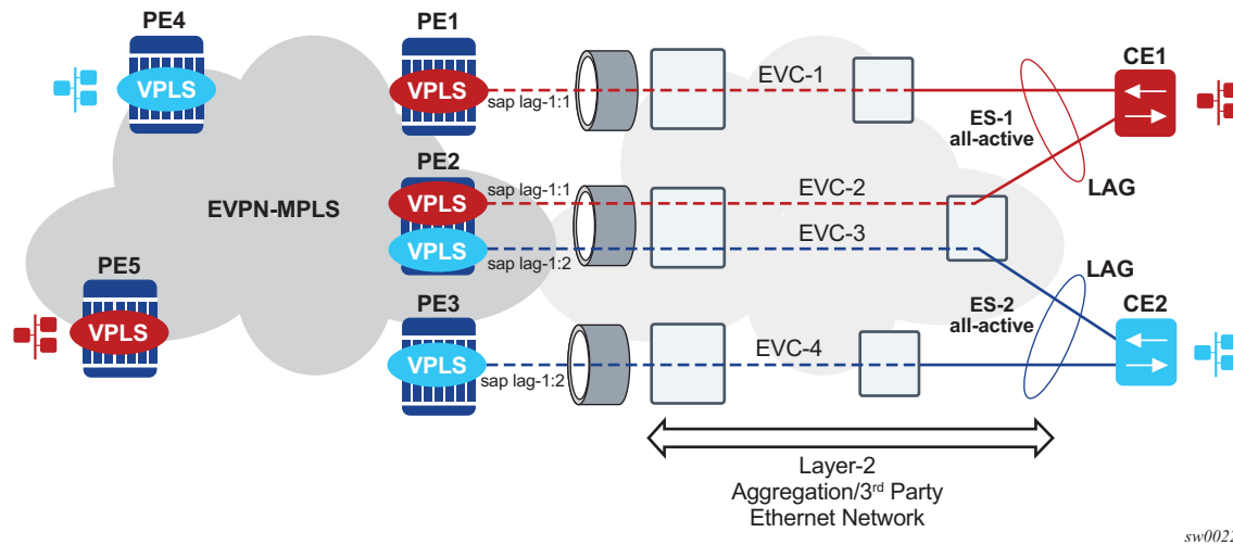
Figure 181 All-Active Multi-Homing on vES
