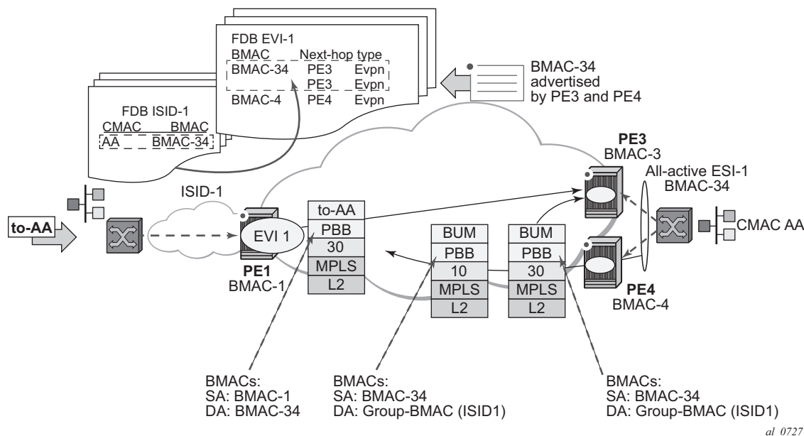
Figure 175 PBB-EVPN All-Active Multi-Homing
