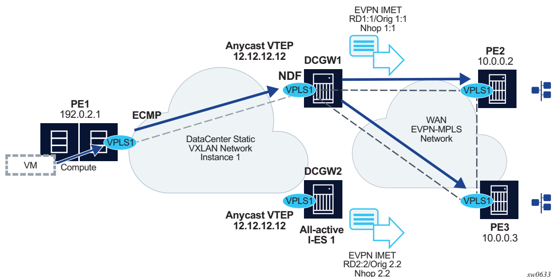
Figure 198 I-ES Multi-homing - static VXLAN with anycast VTEPs
