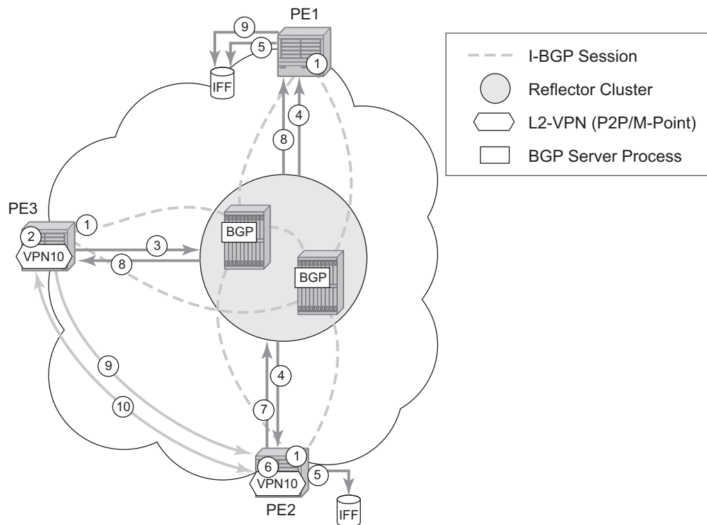
Figure 80 BGP-AD and T-LDP Interaction
