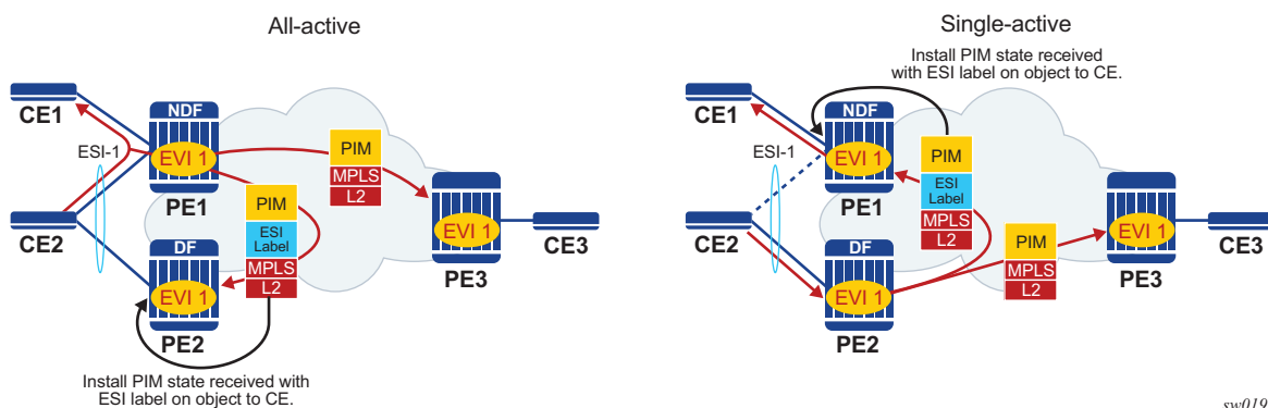
Figure 184 Data-driven PIM Snooping for IPv4 Synchronization with EVPN Multihoming
