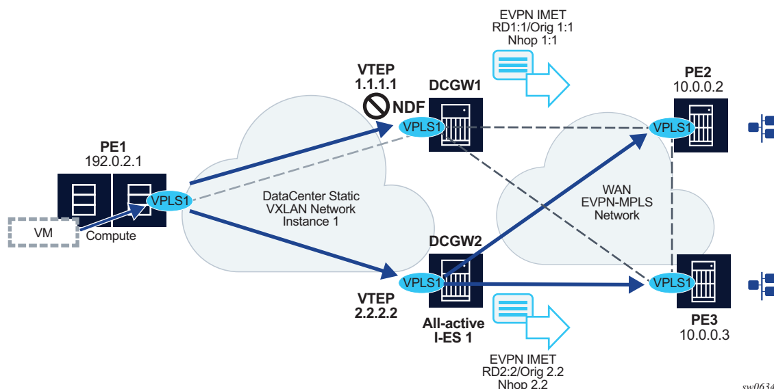
Figure 199 I-ES Multi-homing - static VXLAN with non-anycast VTEPs
