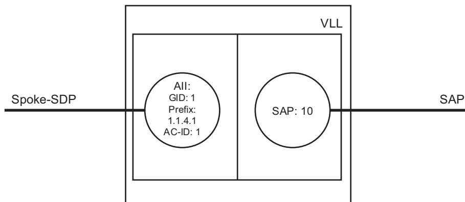
Figure 21 Mapping of AII to SAP
