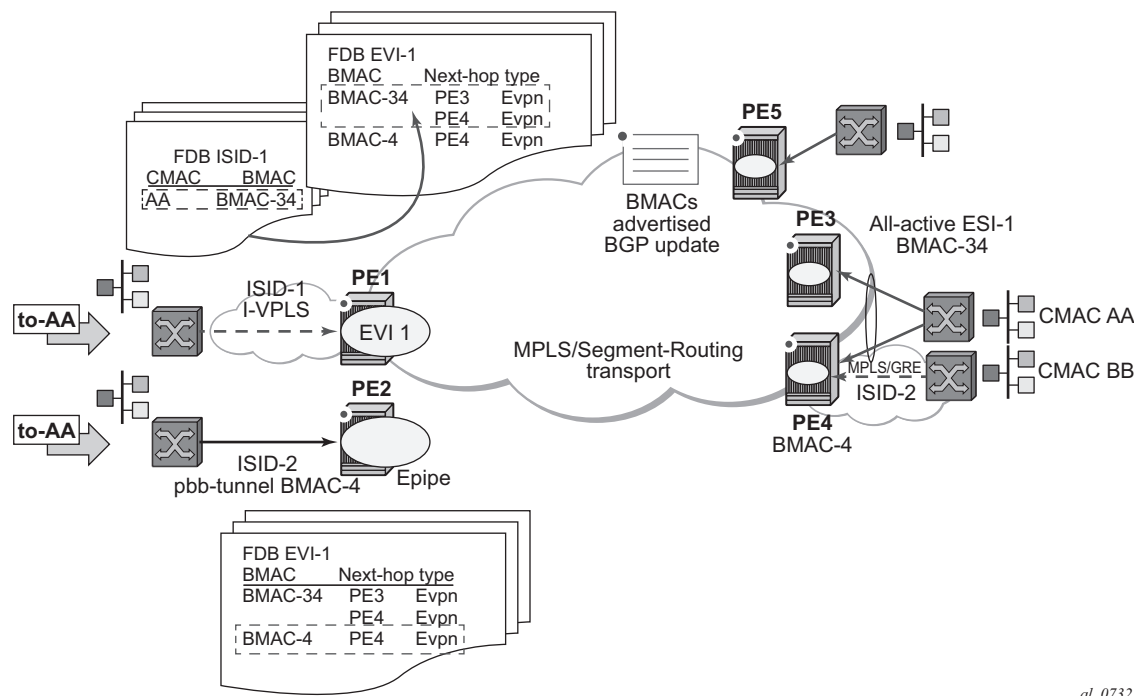
Figure 173 PBB-EVPN for I-VPLS and PFF Epipe Services
