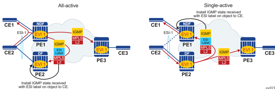
Figure 183 Data-driven IGMP Snooping Synchronization with EVPN Multihoming
