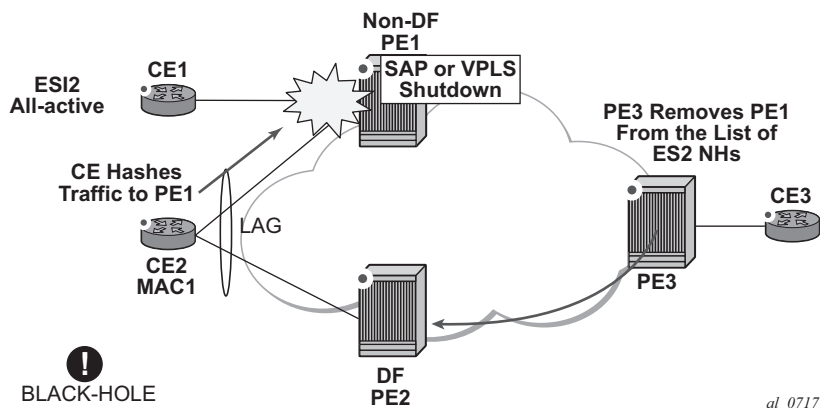
Figure 166 Blackhole Caused by SAP/SVC Shutdown
