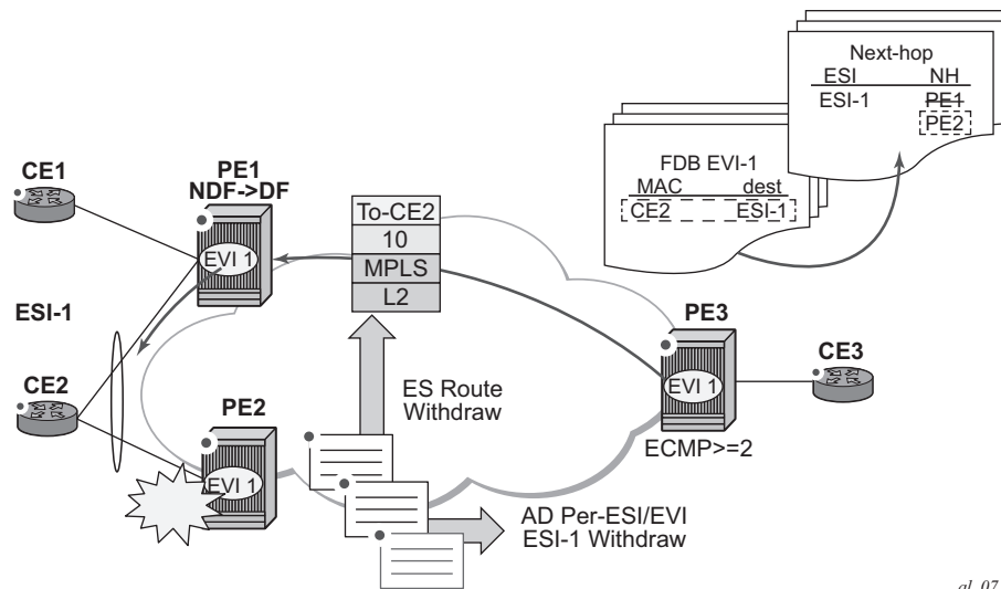
Figure 165 All-Active Multi-Homing ES Failure
