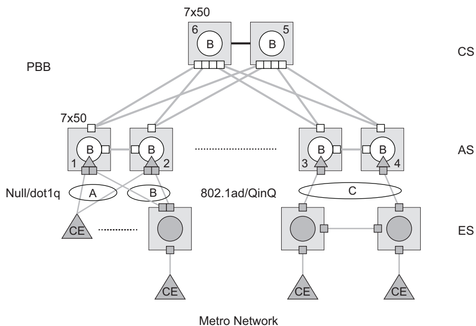
Figure 65 Access Resiliency
