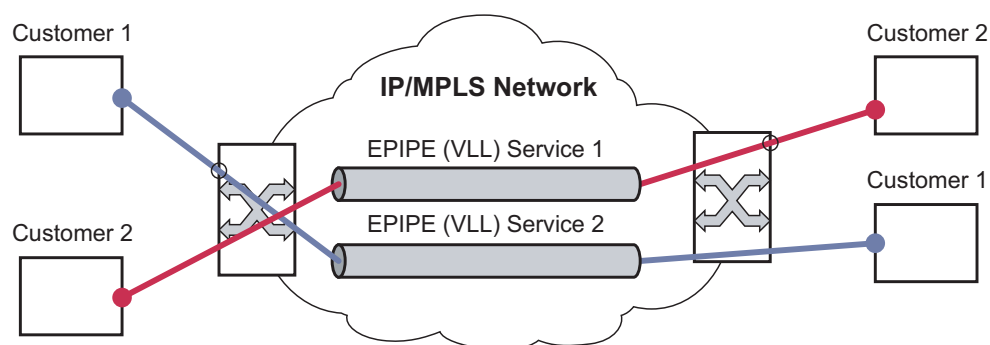
Figure 5 Epipe/VLL Service
