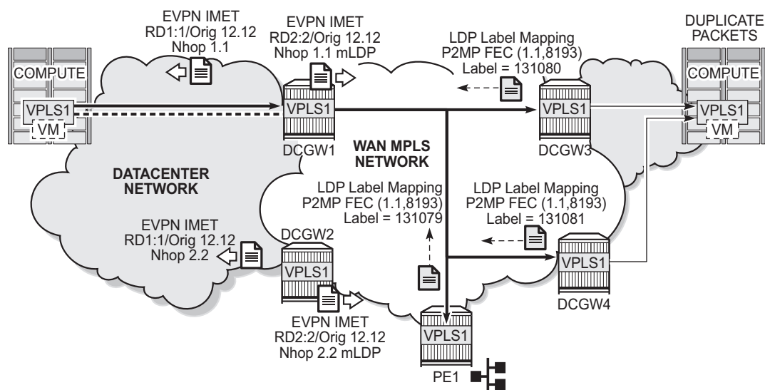
Figure 194 Anycast Multi-homing and mLDP
