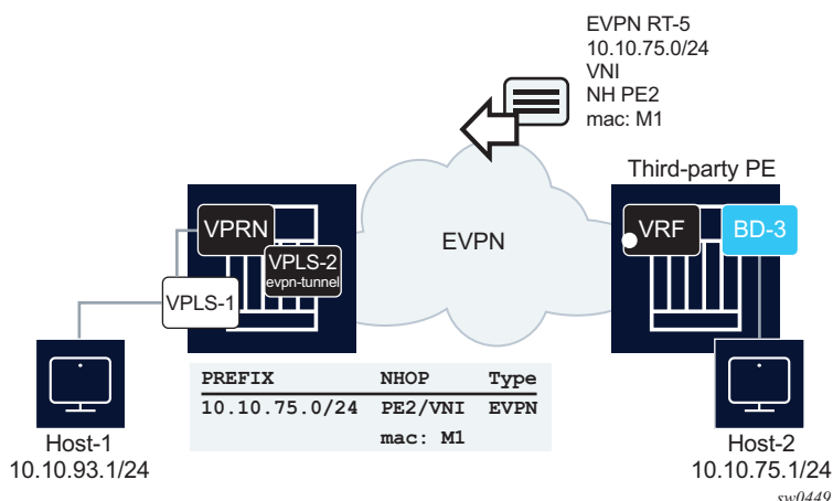
Figure 202 Interface-less IP-VRF-to-IP-VRF Model
