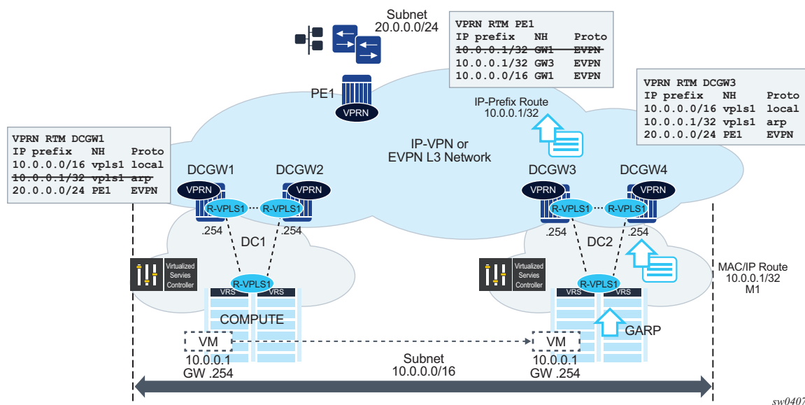
Figure 203 Extended Layer-2 Data Centers
