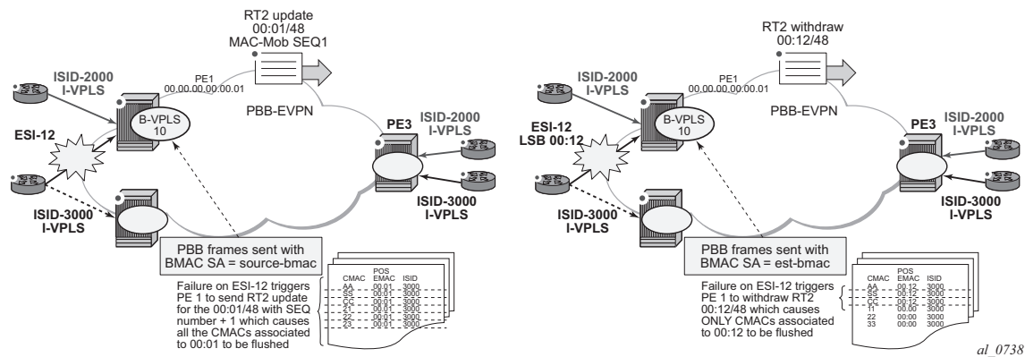
Figure 176 Source-Bmac Versus Es-Bmac CMAC Flushing
