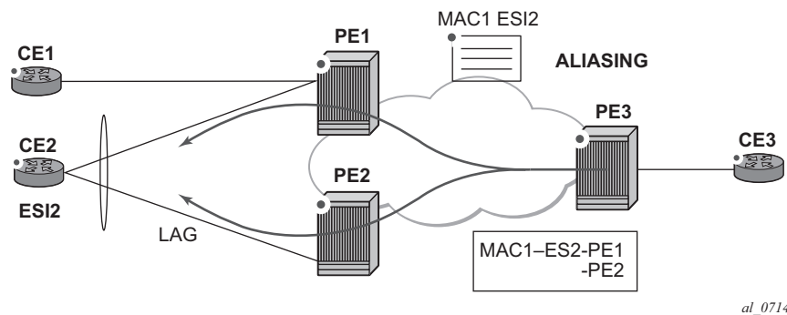
Figure 163 Aliasing
