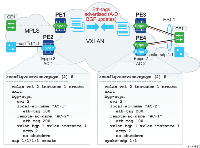
Figure 149 EVPN-MPLS VPWS
