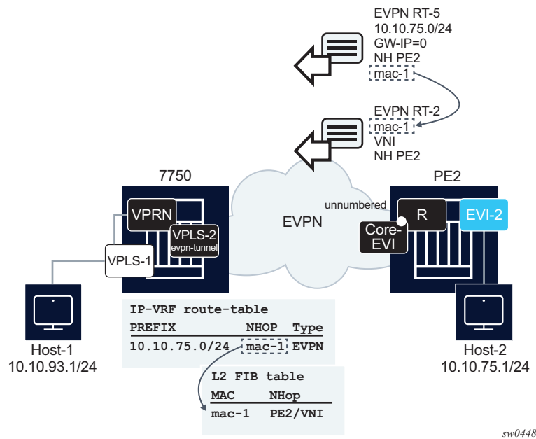
Figure 201 Interface-ful IP-VRF-to-IP-VRF with Unnumbered SBD IRB Model
