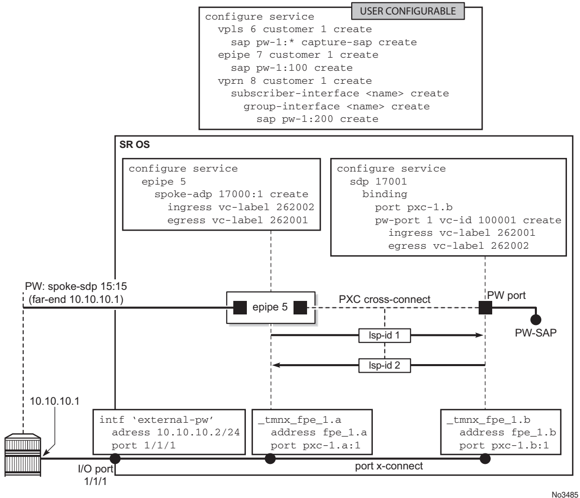
Figure 211 Service Termination on PW-SAP
