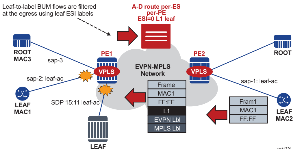
Figure 187 EVPN E-Tree BUM Egress Filtering
