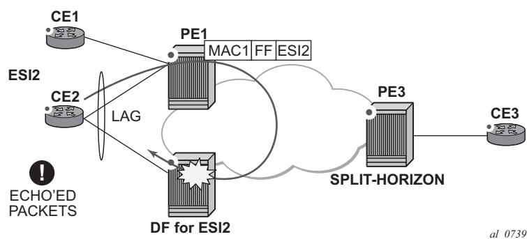
Figure 162 Split-Horizon
