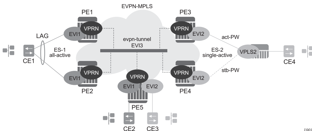
Figure 172 EVPN-MPLS Multi-Homing in R-VPLS Services
