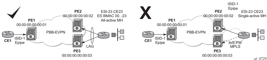
Figure 177 PBB-EVPN MH in a Three-Node Scenario
