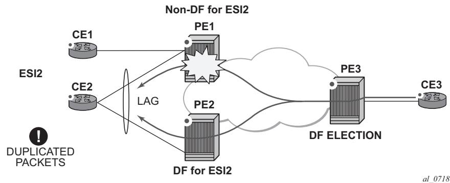
Figure 161 DF Election
