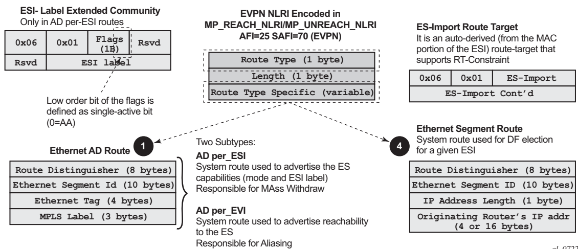
Figure 159 EVPN Routes Type 1 and 4
