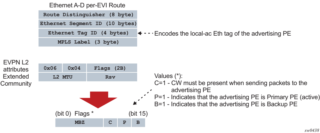
Figure 148 EVPN VPWS BGP Extensions
