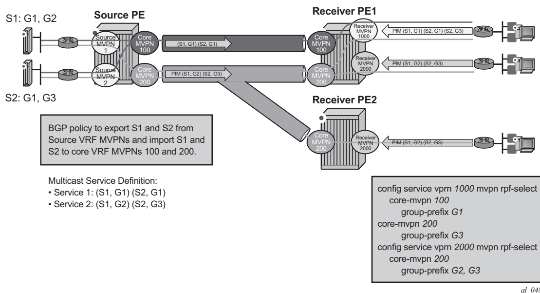
Figure 31 Source PE Transit Replication and Receiver PE Per-group SSM Extranet Mapping
