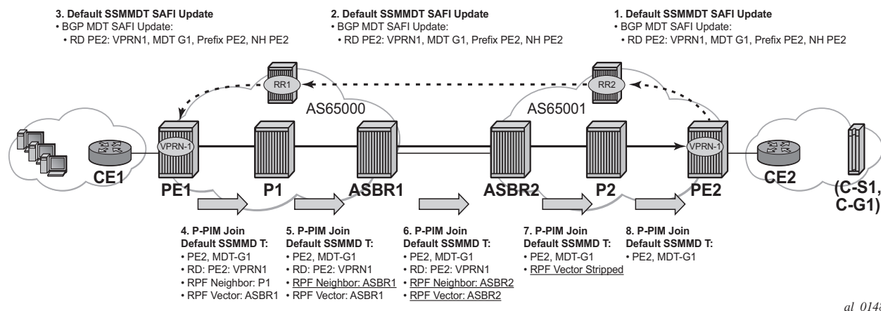
Figure 45 Inter-AS Option C Default MDT Setup
