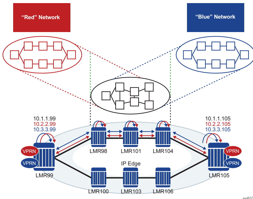
Figure 37 Logical Networks Using Multi-Instance IGP
