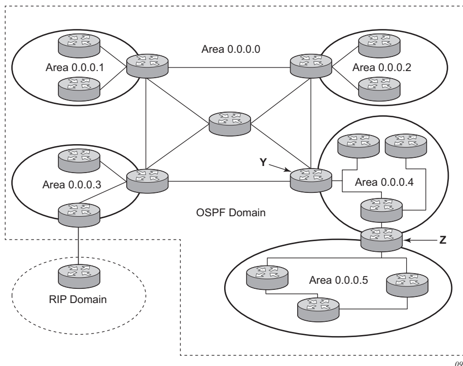
Figure 53 OSPF Areas
