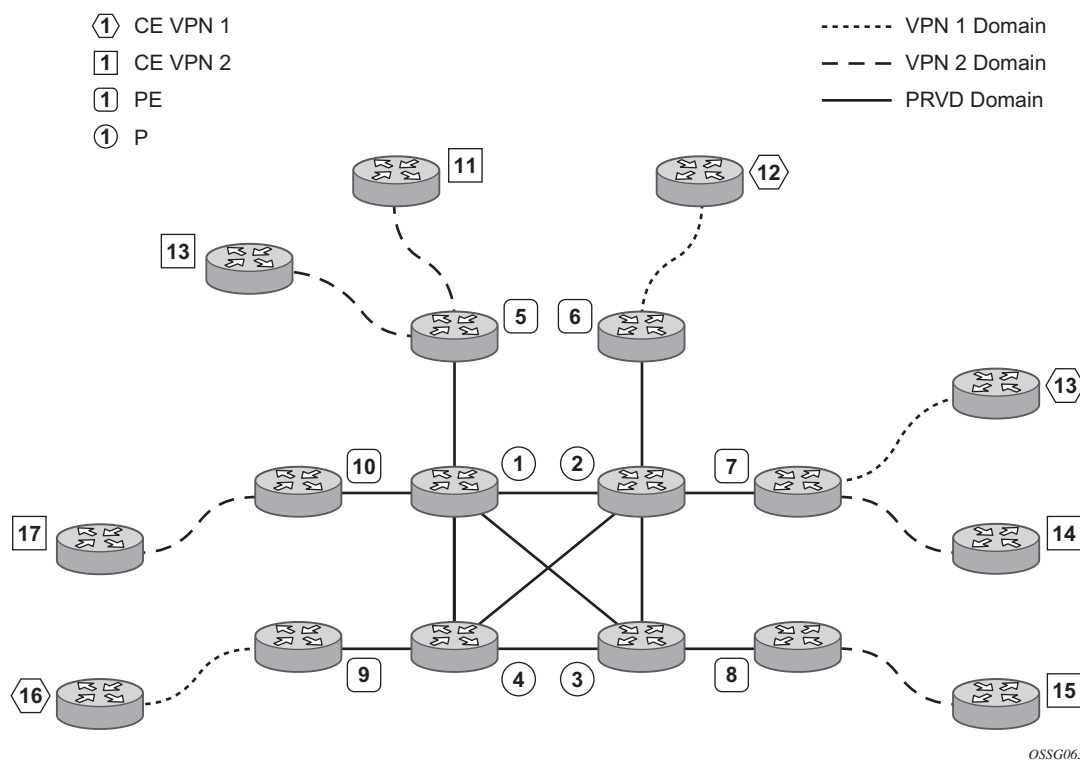
Figure 27 Multicast in IP-VPN Applications
