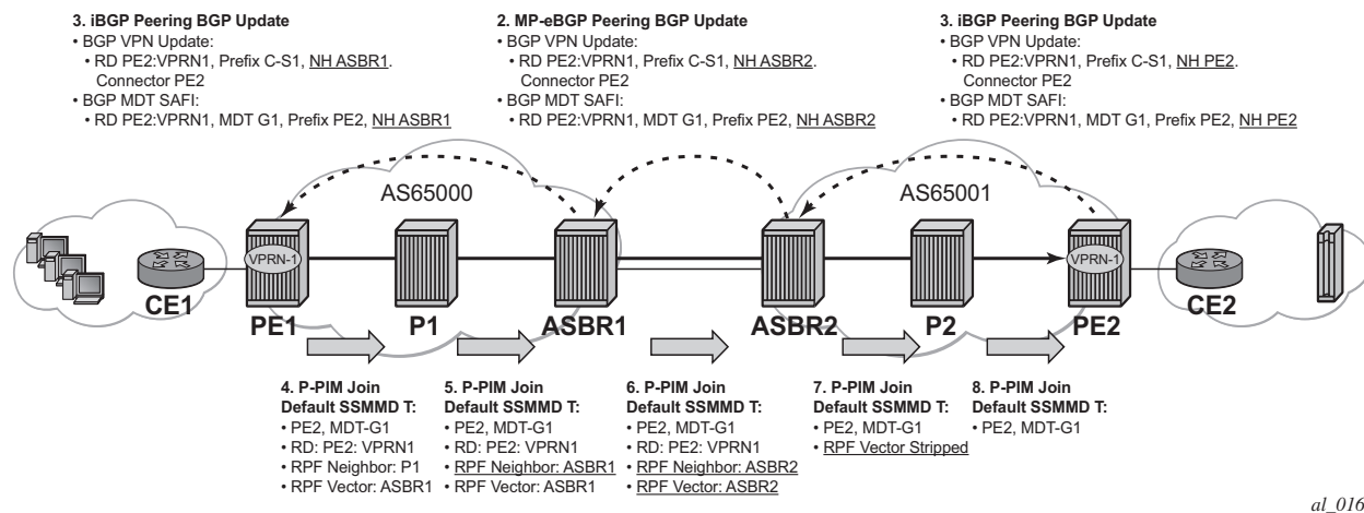
Figure 44 Inter-AS Option B Default MDT Setup
