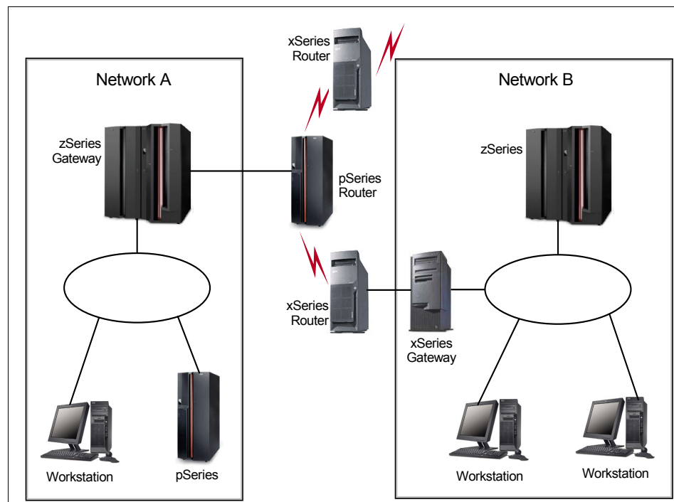
Figure 17-2 TCP/IP introduction
