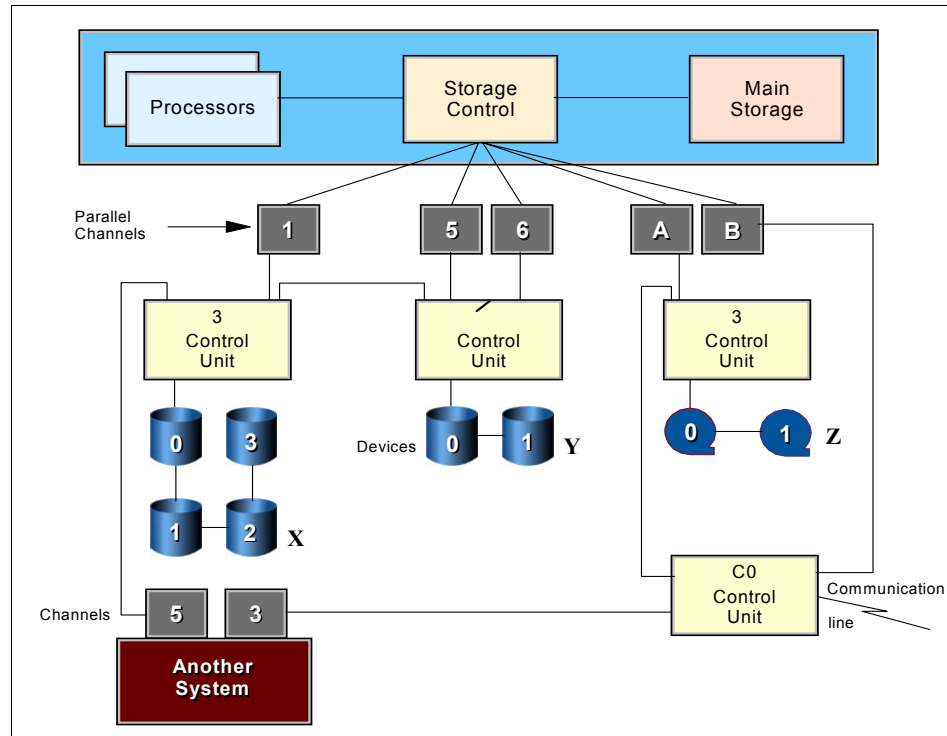
Figure 2-2 Conceptual S/360
