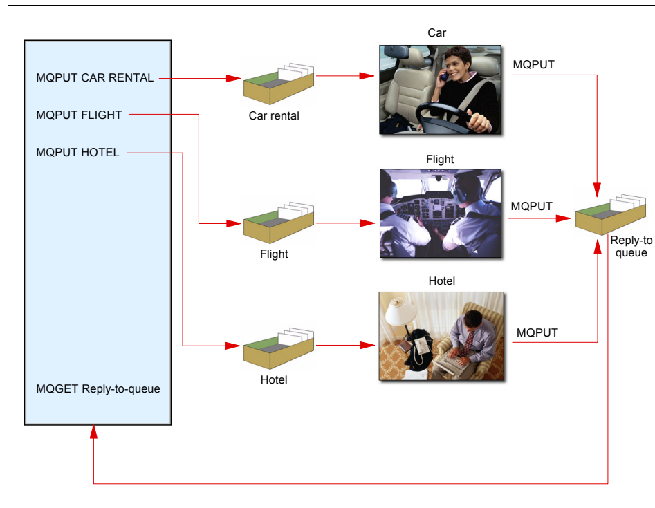
Figure 14-4 Parallel processing
