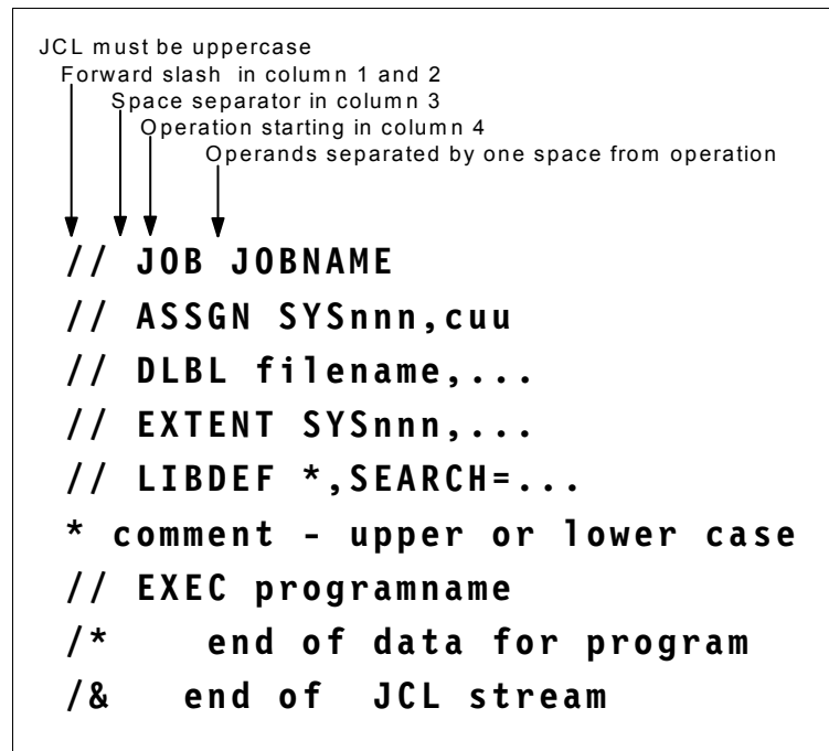
Figure 6-1 Basic JCL coding syntax
