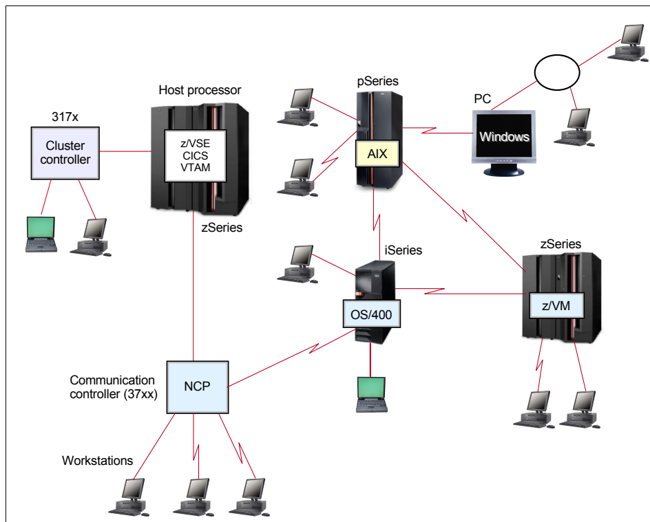
Figure 17-3 VTAM overview - the SNA environment
