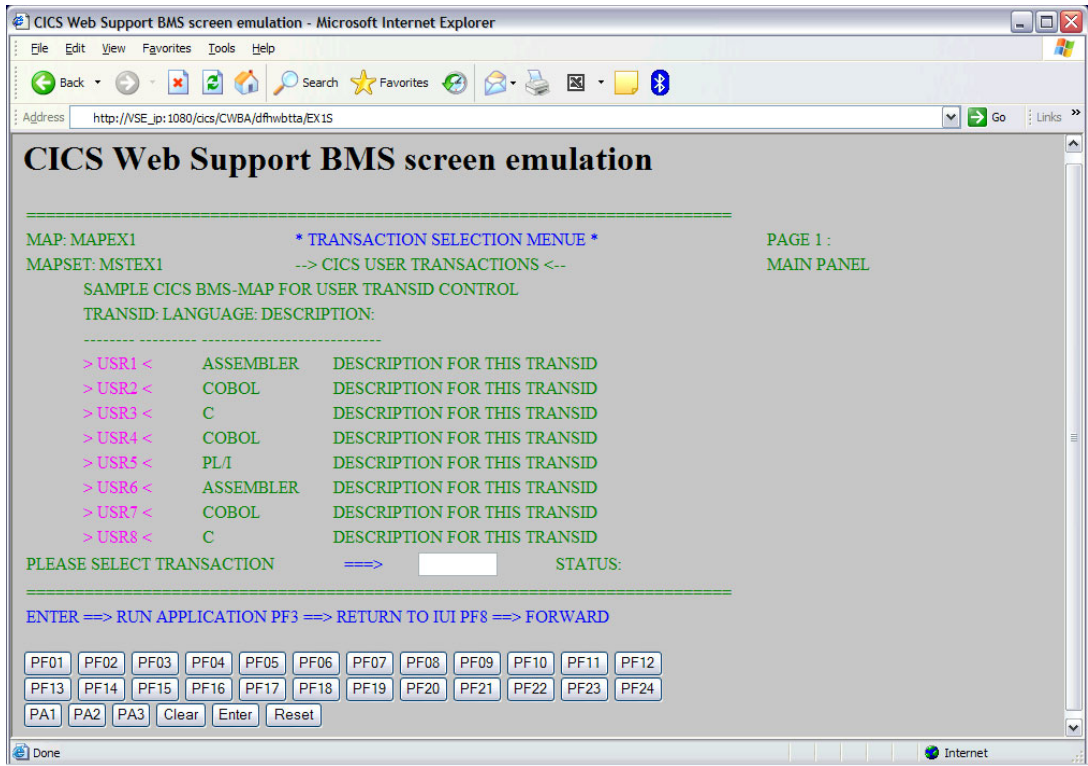
Figure D-3 HTML correspondent of BMS map MAPEX1
