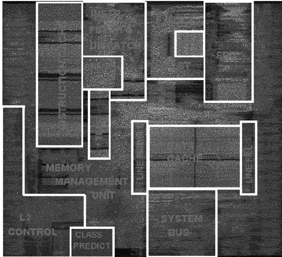
Figure 3. NorthStar Chip
