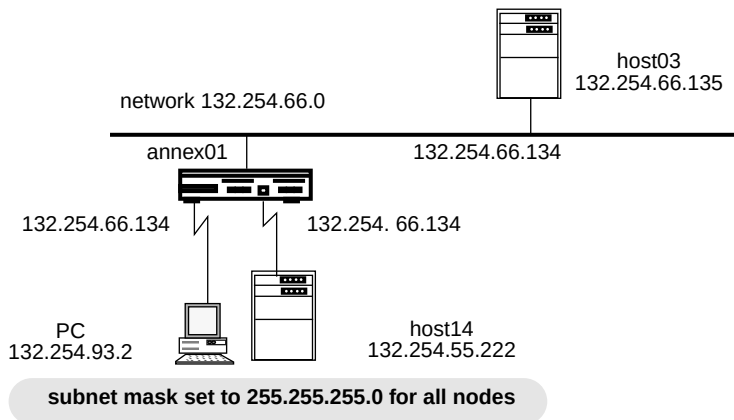
Figure A-19. Advertising Subnet Routes
