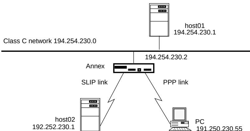
Figure A-14. Configuration Using Four Class C Node Addresses
