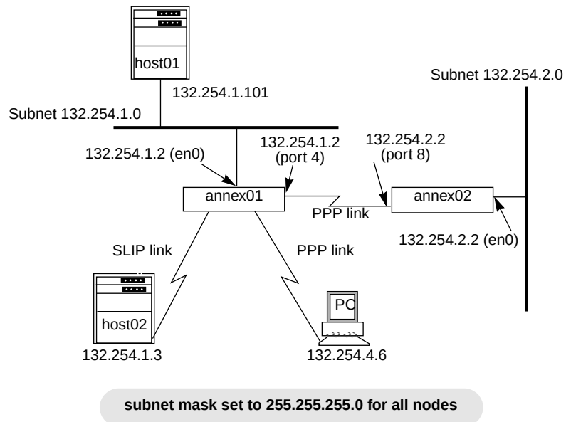
Figure A-17. Sample Network for Defining Default Routes with Passive RIP
