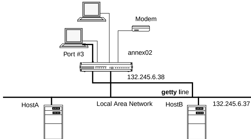
Figure A-2. Host Applications Accessing a Terminal
