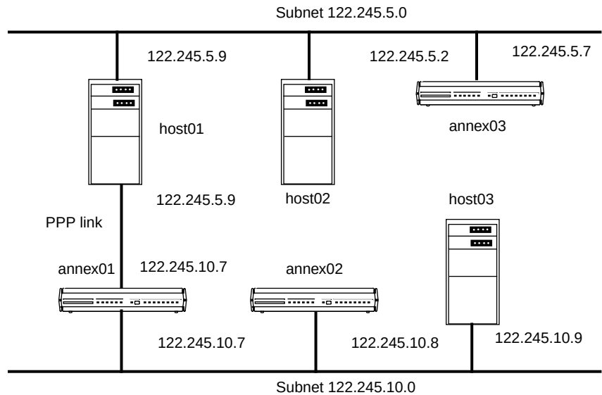
Figure A-7. PPP Link Connecting Two Subnets
