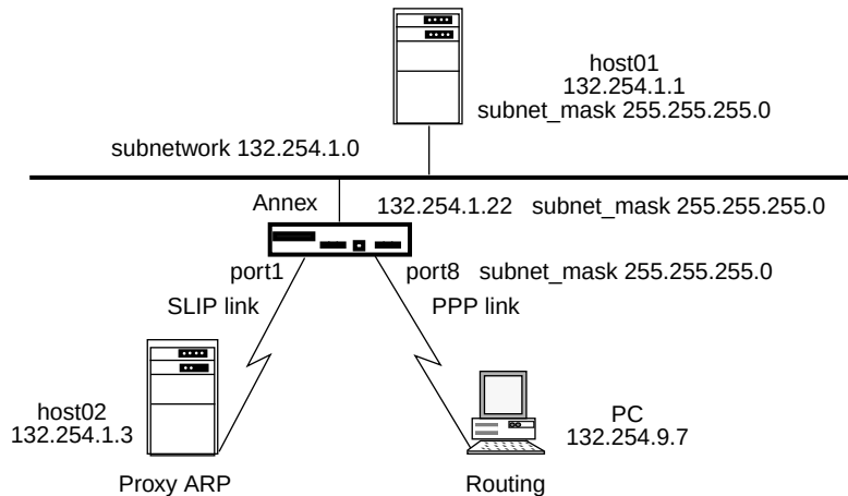
Figure A-16. Proxy ARP versus Routing
