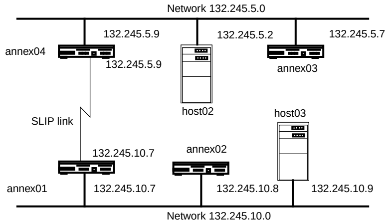
Figure A-11. SLIP Link with Two IP Addresses
