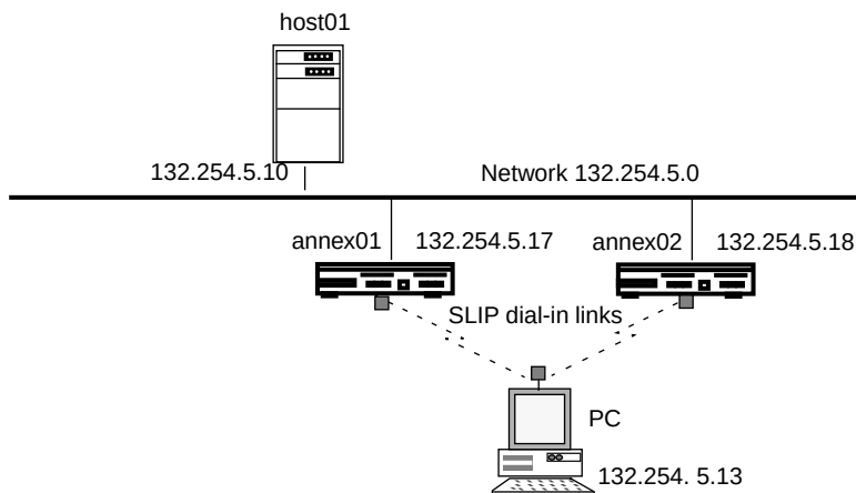
Figure A-22. Configuration in Which Proxy ARP Can Fail
