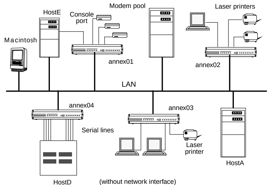
Figure A-3. Connecting Devices to a Remote Annex
