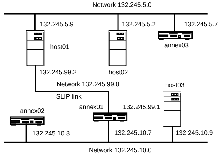
Figure A-10. SLIP Link with Separate Network Address
