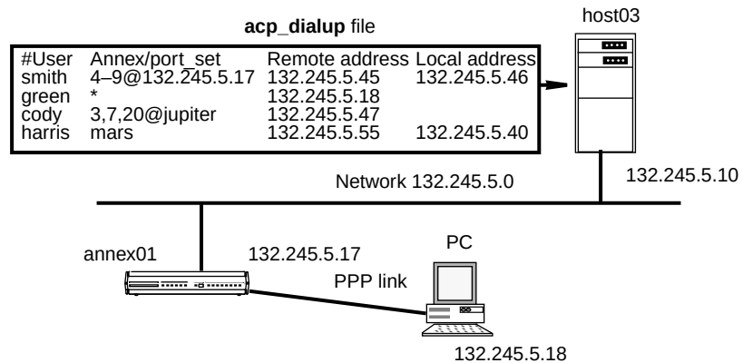
Figure A-8. Connecting a Single Host Using PPP
