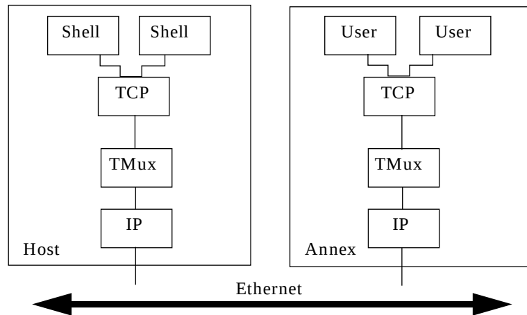
Figure A-6. TMux Block Diagram
