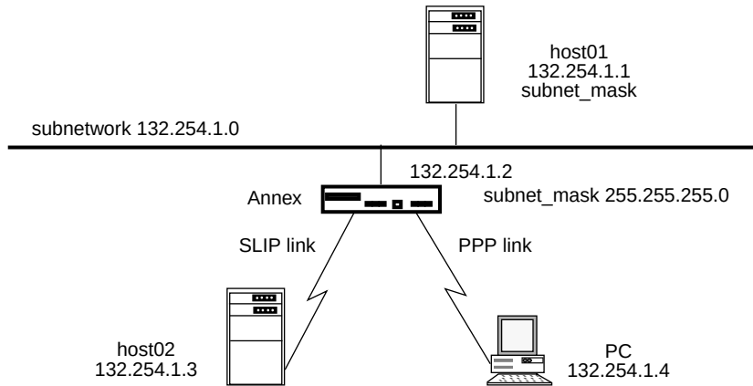
Figure A-15. Subnetting with Passive RIP
