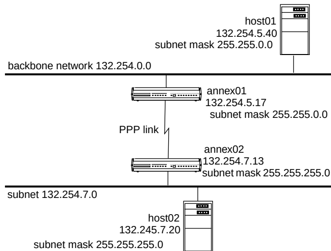
Figure A-23. Overlapping Addresses
