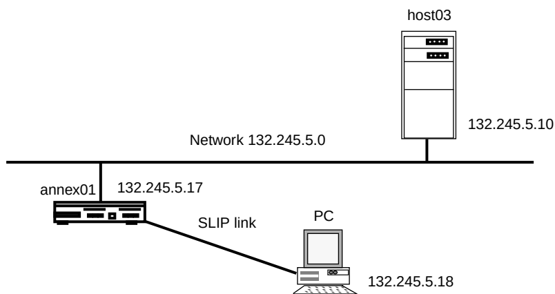
Figure A-12. Connecting a Single Host Using SLIP
