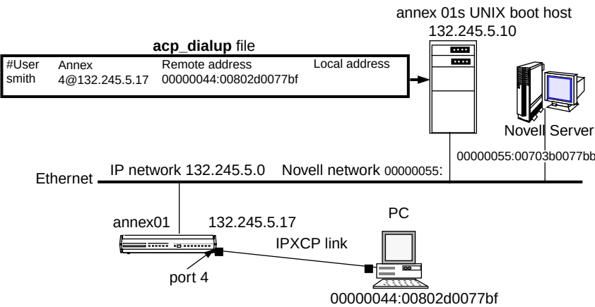
Figure A-27. Connecting a Single Host Using IPXCP
