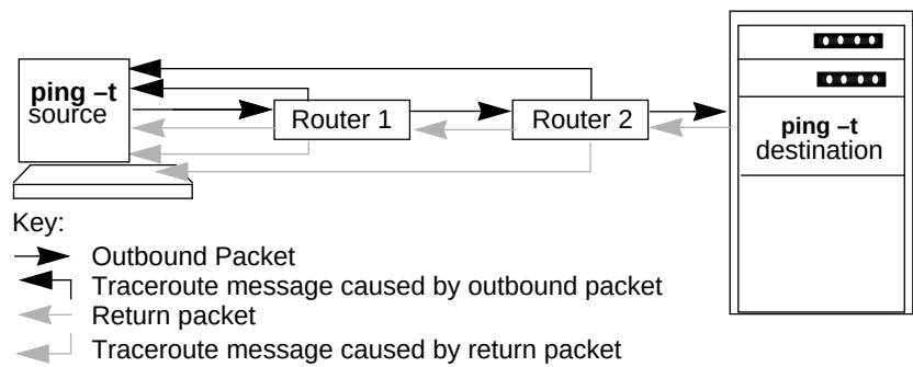
Figure A-20. Overview of ping -t Actions
