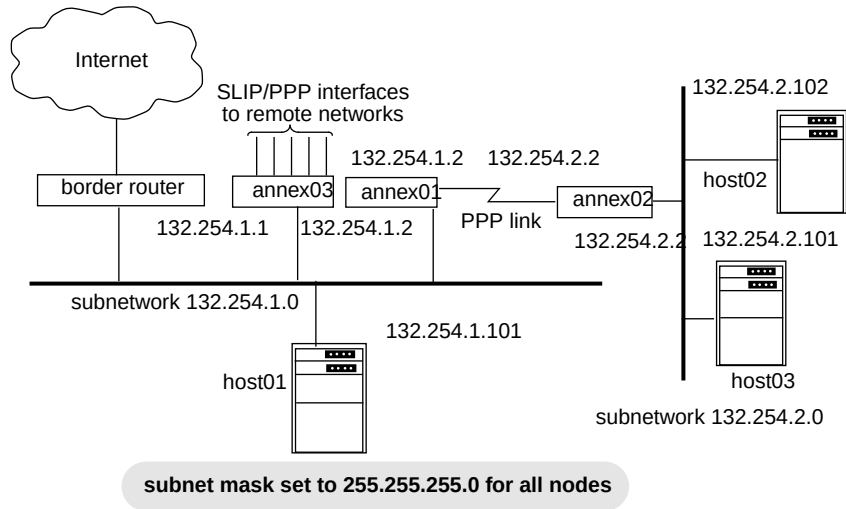
Figure A-18. Sample Network for Static and Default Routes (Passive RIP)
