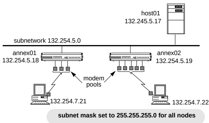
Figure A-24. Non-contiguous Subnets
