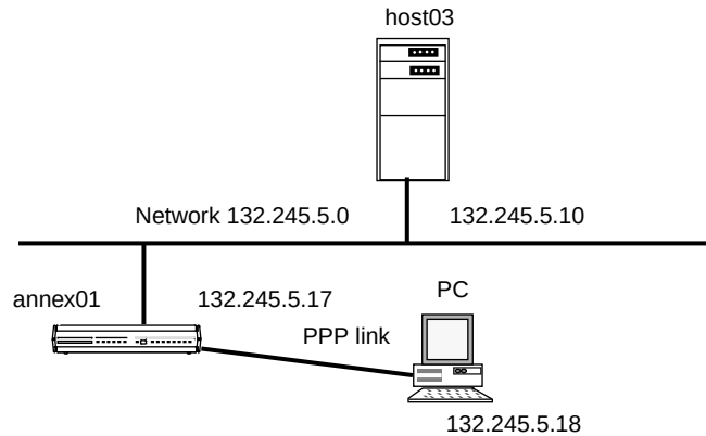
Figure A-9. Connecting a Single Host Using PPP with Fixed Addresses
