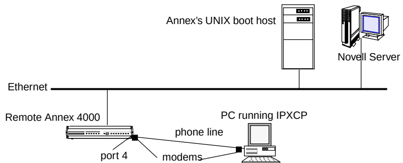
Figure A-26. Sample Hardware for Minimum IPXCP Configuration
