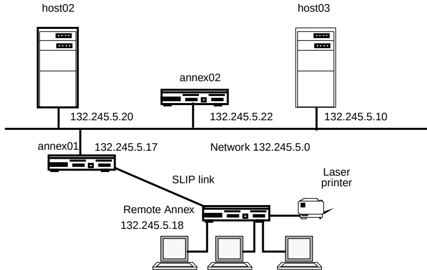
Figure A-13. Connecting a Remote Annex
